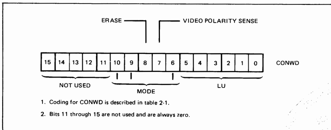
Figure 2-1. CONWD Format
