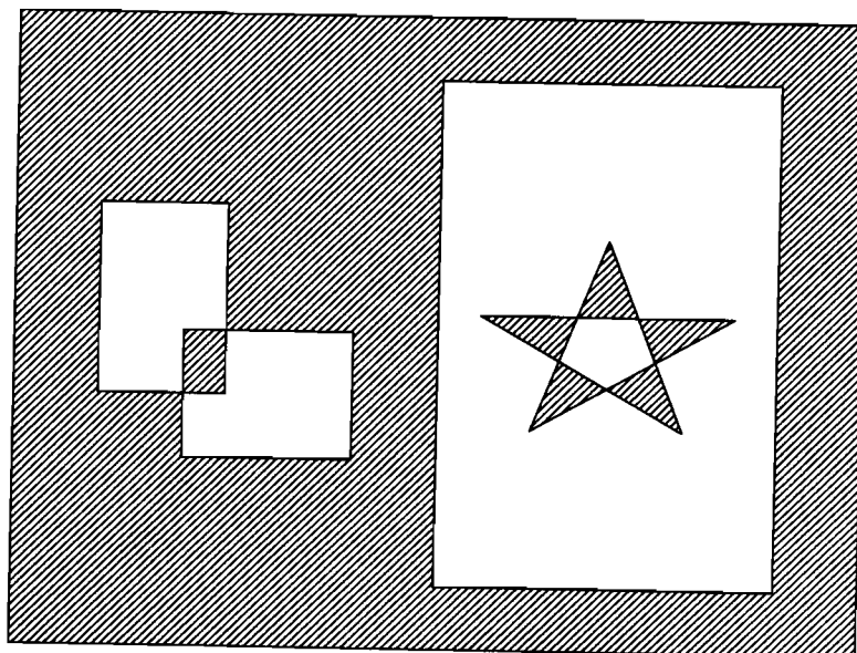
Polygon Filling
