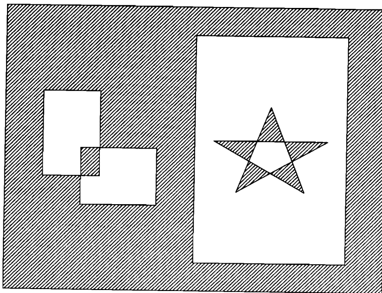
Polygon Filling
