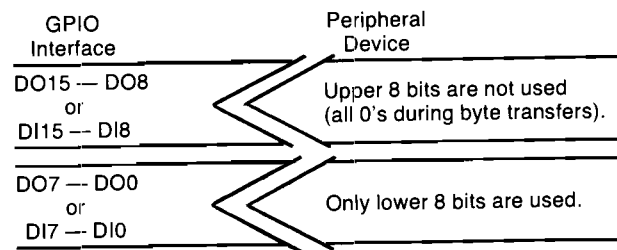
Diagram of Byte Transfers
