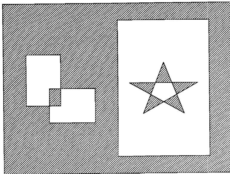
Polygon Filling
