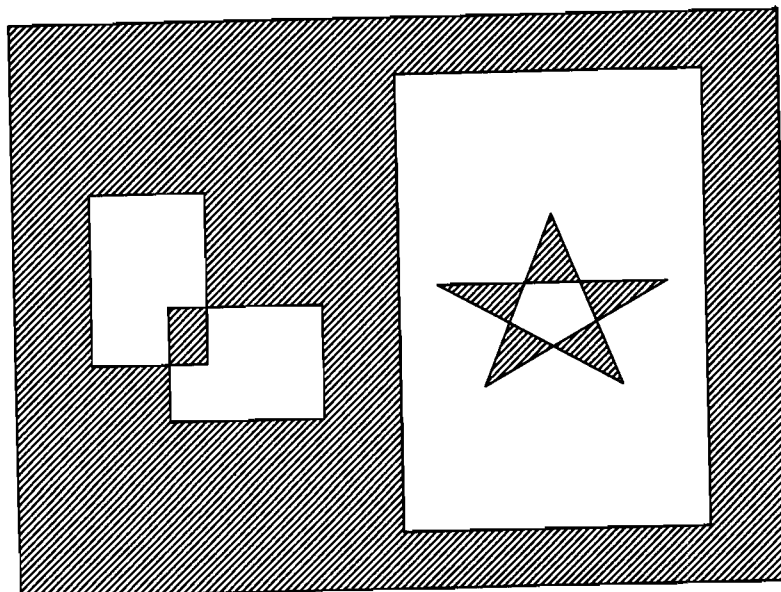
Polygon Filling
