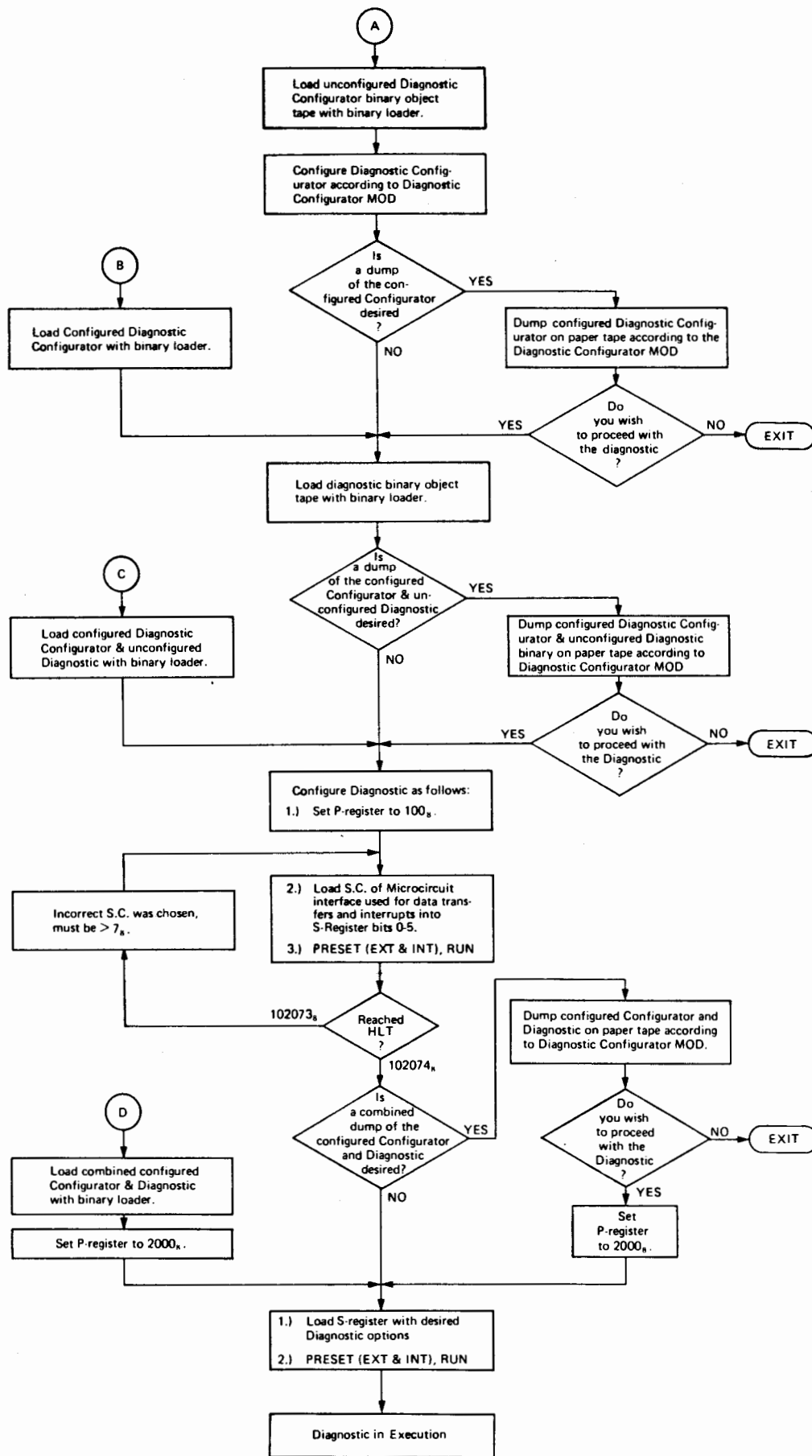
Figure 3-1. Operating Procedure Flowchart
