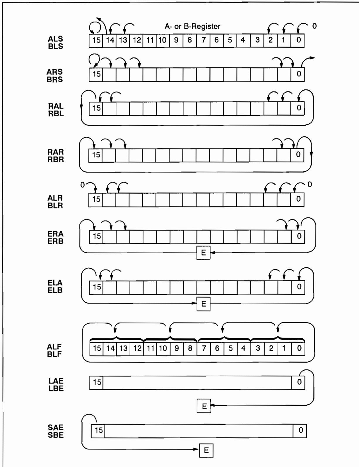
Figure 3-1. Instructions of the Shift-Rotate Group
