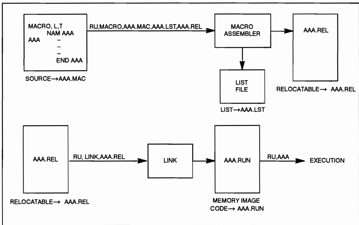
Figure 1-2. Assembly Process
