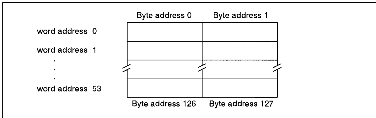
Figure 4-2. Byte Addressing
