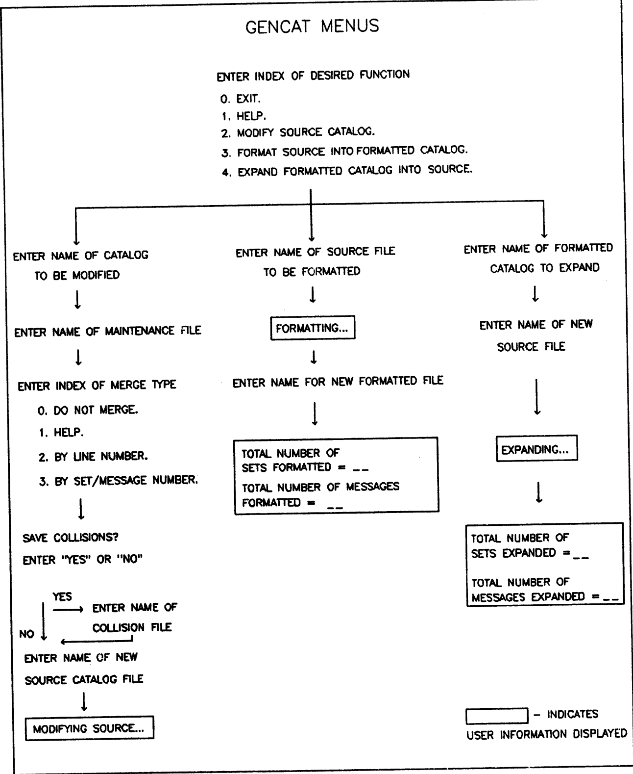
Figure 2-2. GENCAT Functions
