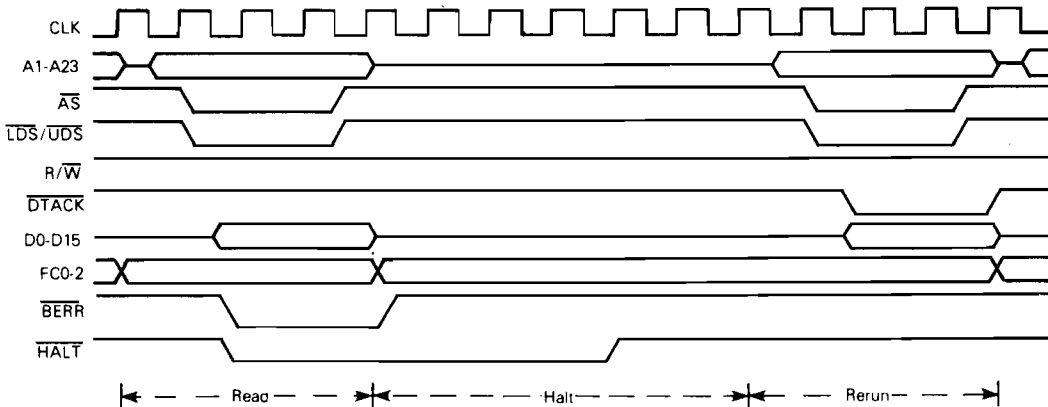
Figure 4-18. Re-Run Bus Cycle Timing Information
