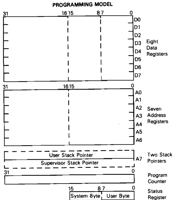
Figure 1-2. Programming Model
