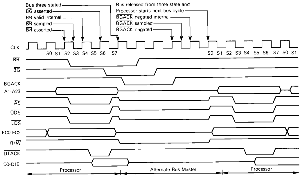
Figure 4-14. Bus Arbitration Timing During Active Bus Cycle
