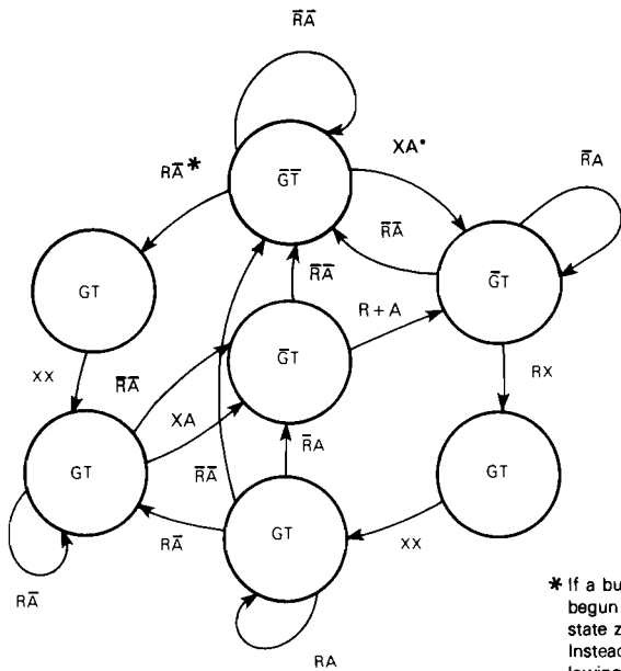
Figure 4-13. Bus Arbitration Control-State Diagram
