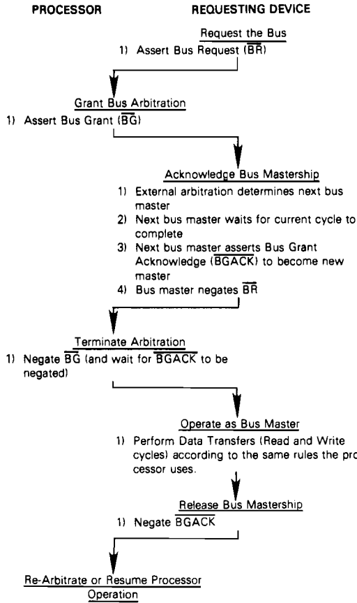
Figure 4-11. Bus Arbitration Cycle Flow-Chart
