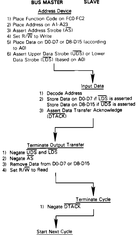
Figure 4-7. Byte Write Cycle Flow Chart
