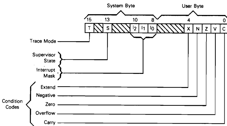
Figure 1-3. Status Register
