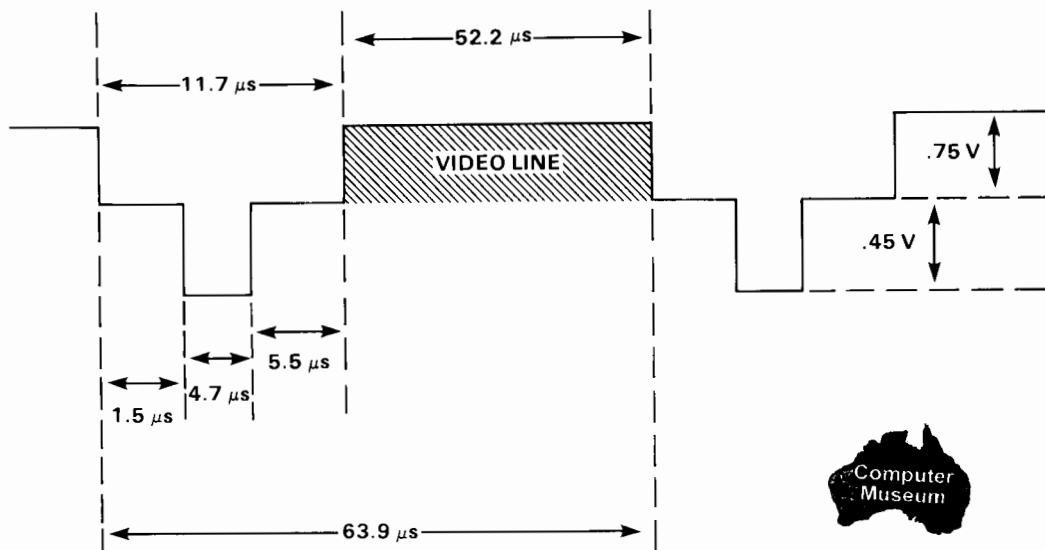
Horizontal Composite Waveform*
