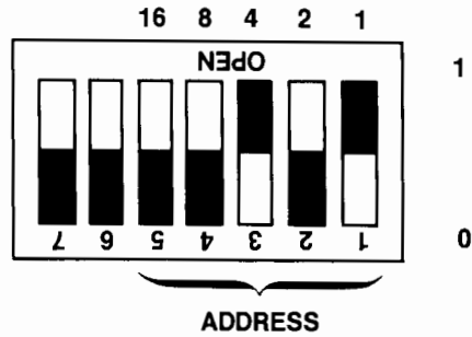
Device address switch of HP 7470A Plotter.
