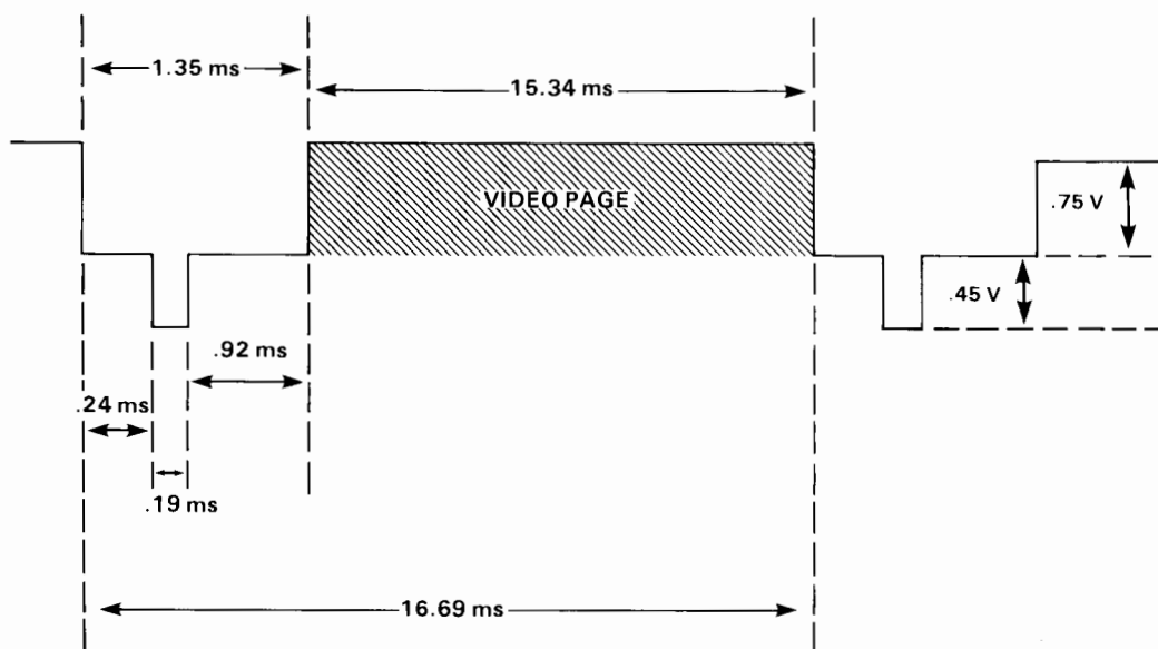
Vertical Composite Waveform*
