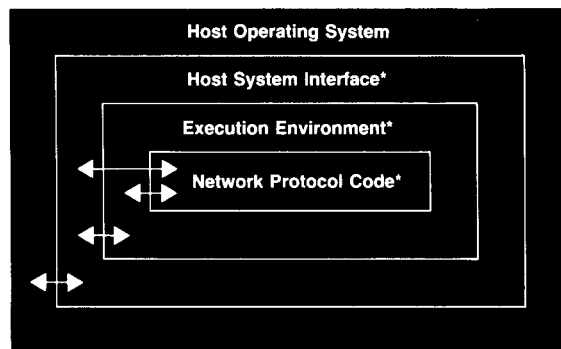
Fig. 3. Layered isolation of portable network code.
