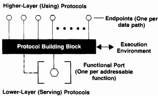
Fig. 4. Interfaces to the protocol building block.
