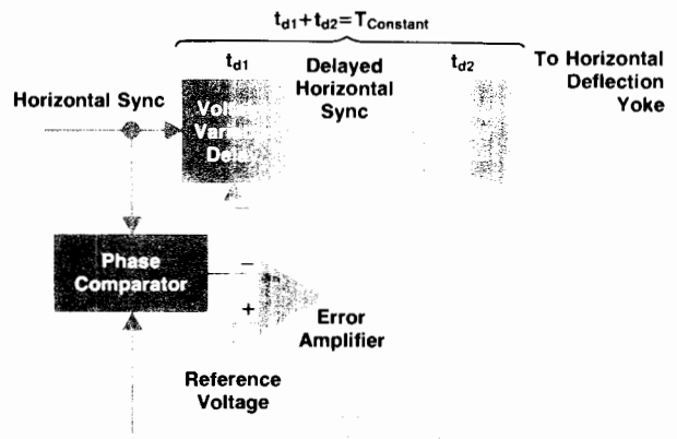
Fig. 4. Feedback loop stabilizes the horizontal sync pulse so the soft key labels on the CRT remain stable over the keys.
