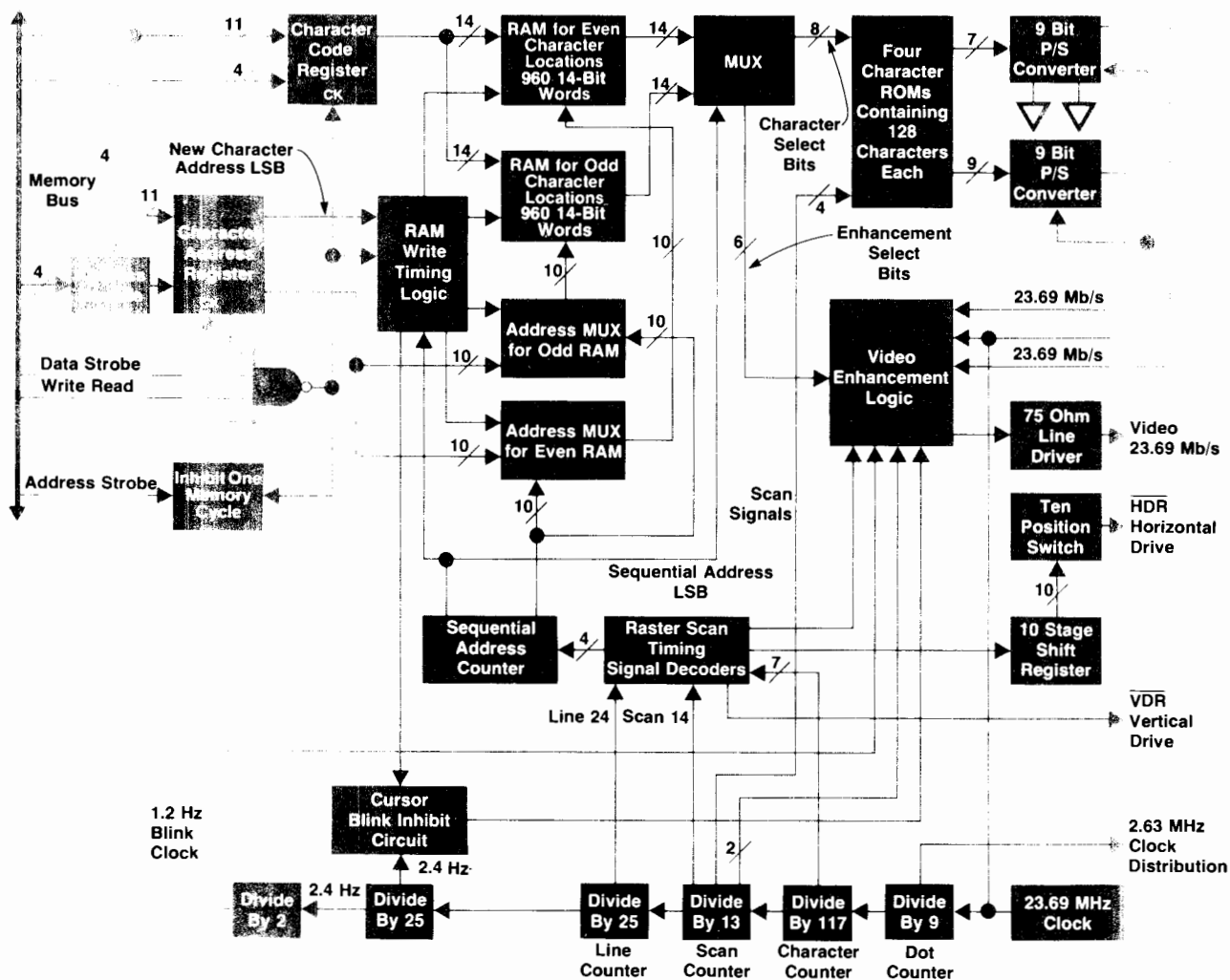
Fig. 2. Display logic board requires no processor attention for a static display. Separate random-access display memories (RAMs), one for even character locations and one for odd, make it possible to update the display without interfering with display refresh.
