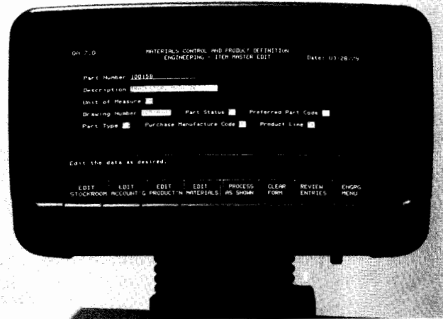
Fig. 1. Eight keys under the HP 250 CRT display can be defined differently in different applications programs to allow the operator to select various functions. The functions appear on the CRT above the keys. Also shown here is an example of a form in which data entry and display are programmed using standard INPUT, ENTER, and DISP statements.
