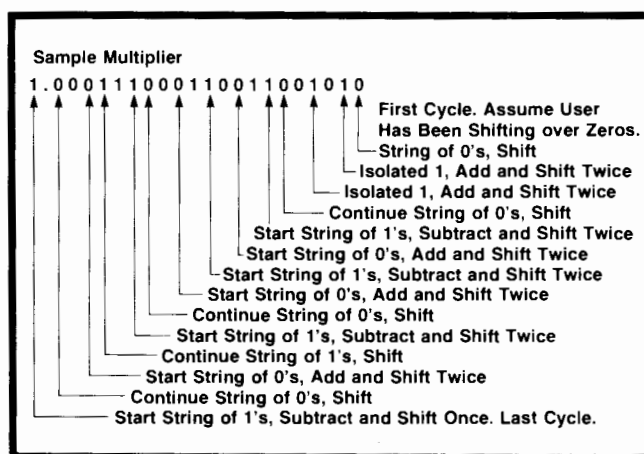
Fig. 5. Floating point multiplication in the F-Series floating point processor executes almost as fast as addition. The multiplication algorithm calls for an arithmetic operation (addition or subtraction) only at the start and end of a string of zeros or ones or at isolated ones in the multiplier. As shown here for this sample multiplier, this means that each arithmetic cycle is followed by two shift cycles. In the FPP this double shift is performed by hardware multiplexers, thereby eliminating the shift cycles and saving a great deal of time.
