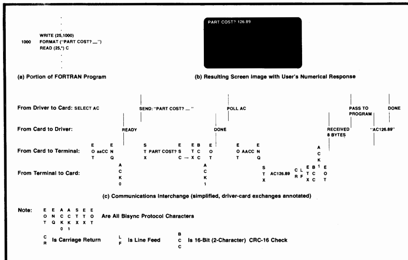
Fig. 2. HP 1000 multipoint protocol example, showing typical communications interchanges between the multipoint software (driver), the multipoint hardware (card), and a terminal. The multipoint interface card, which is microprocessor-based, handles the protocol requirements, relieving the computer of this burden.
