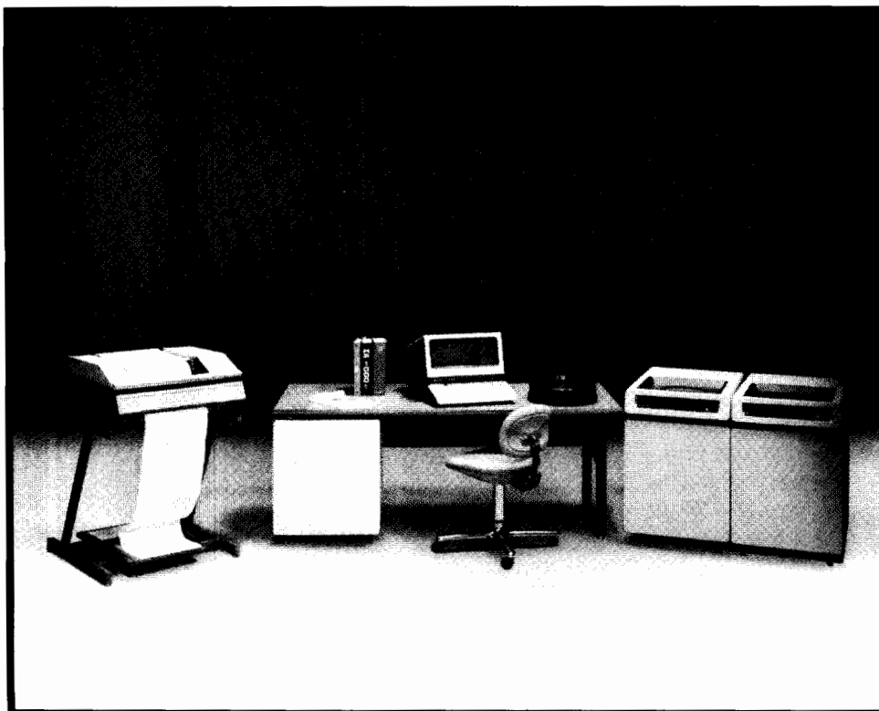
Fig. 1. The new Model 45, the most powerful HP 1000 System, features the new F-Series Computer with floating-point processor and the new RTE-IV operating system. It is designed for applications involving extensive computation, large programs, large data arrays, and graphics. It is shown here with 100M bytes of disc storage.
