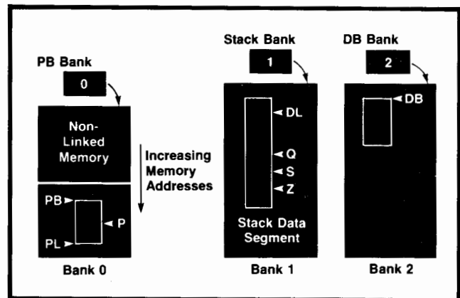
Fig. 3. Modified register structure of the HP 3000 Series II. Memory is divided into four banks of up to 64K words each. Three bank registers (shown at top) allow code and data segments in different banks to be used simultaneously.
