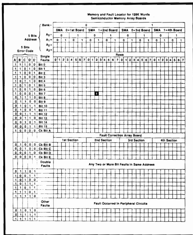
Fig. 5. The error code pinpoints the bit in error for all single-bit errors, as shown at left. All single-bit errors are corrected automatically and logged in a 1024-bit RAM, as shown here for the example of Fig. 3.
