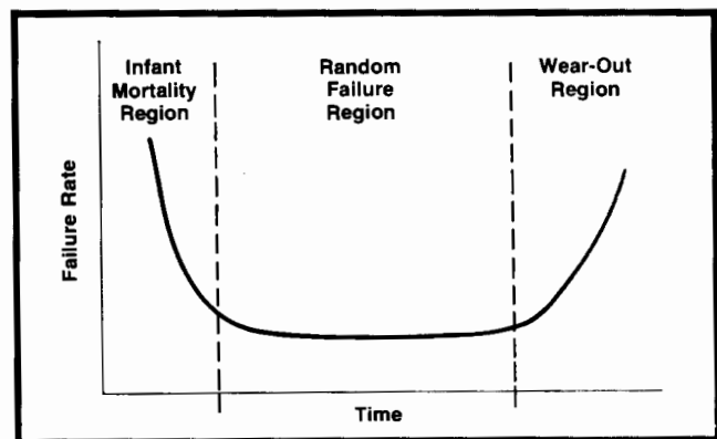
Fig. 2. 4K RAMs follow the well-known reliability life curve. Error correction reduces the effects of memory failures on system performance in all regions of the curve.
