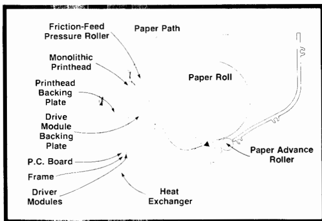
Fig. 2. Sectional view of the printhead/paper relationship.
