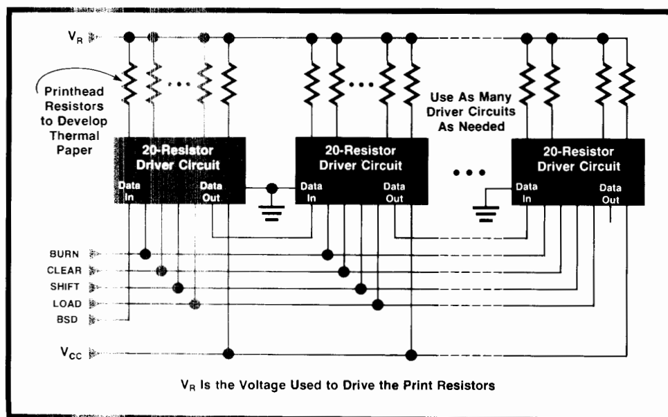
Fig. 3. Twenty-eight 20-resistor driver chips receive burn information from the printer's internal microprocessor and energize the printhead resistors.
