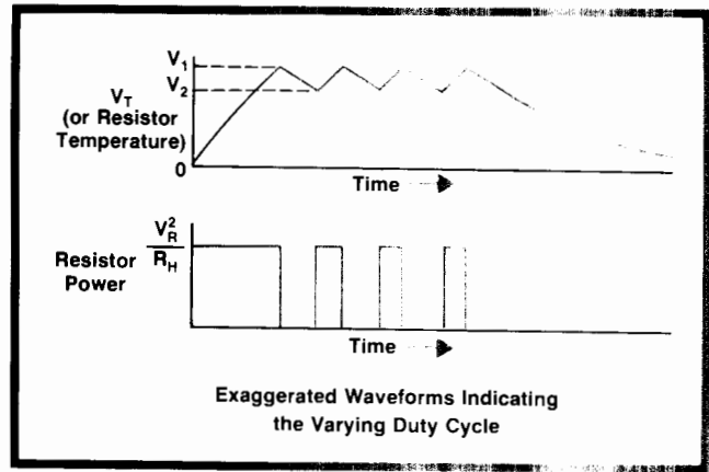
Fig. 6. Print resistor power is controlled to heat the resistor rapidly without exceeding a reliable burn temperature. Temperature is maintained by pulse modulating the resistor power.
