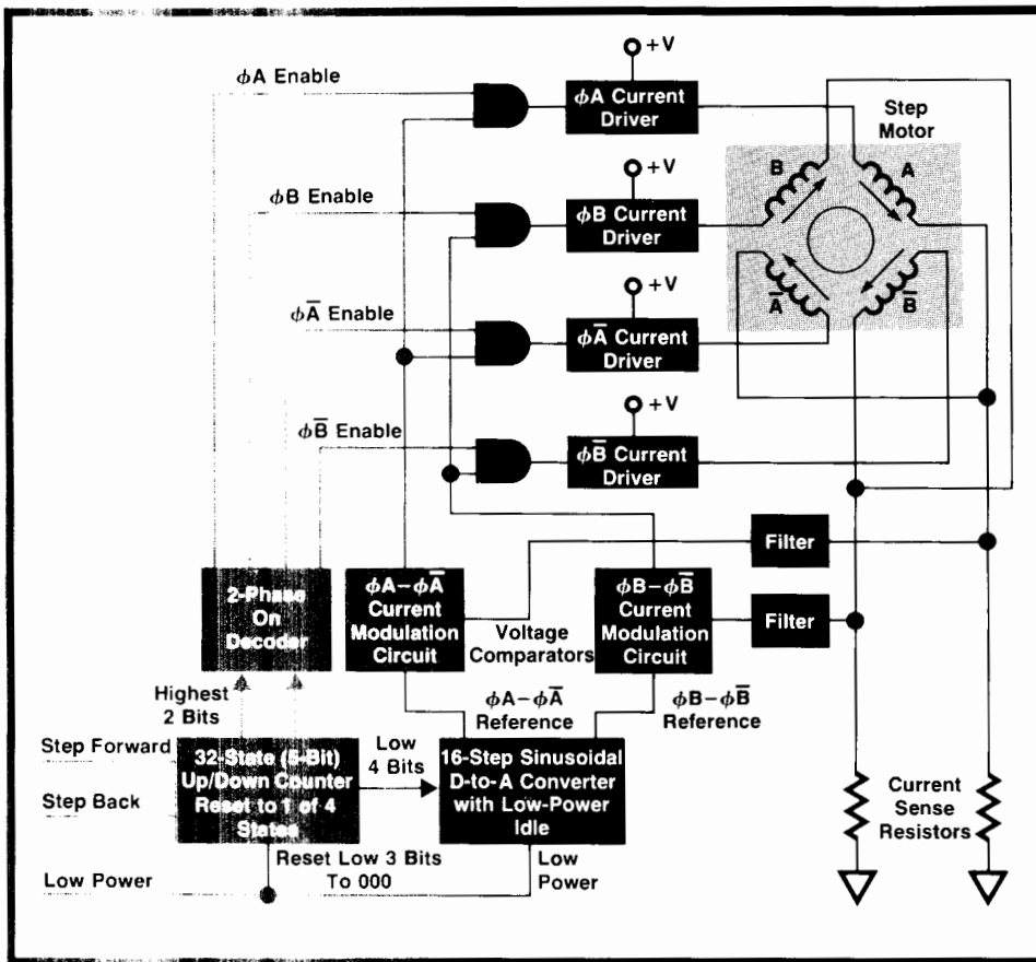
Fig. 7. Ministepped paper-advance motor drive system minimizes audible noise. Under microprocessor control, the drive system breaks each step-motor step into eight smaller steps, and slowly steps down the A-phase current while it steps up the B-phase current.
