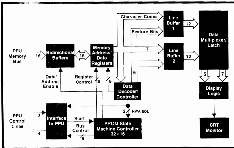
Fig. 10. Alphanumeric display block diagram.
