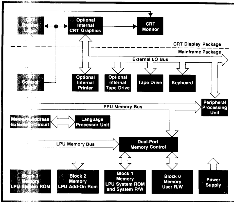
Fig. 1. System 45 architecture is similar to that of previous Series 9800 Desktop Computers except that System 45 has two micro-processors, the language processor unit (LPU) and the peripheral processing unit (PPU). The PPU is the master controller of the system.
