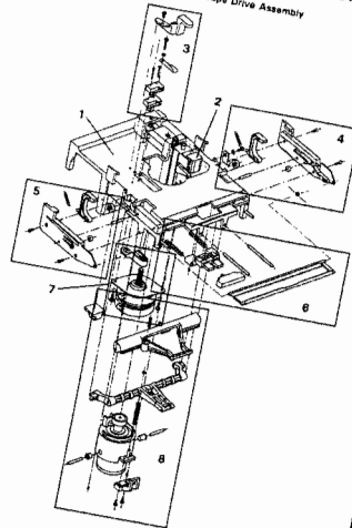
Figure 1: Tape Drive Assembly
