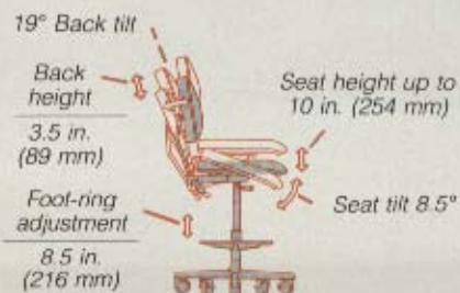
92209S Workbench chair
