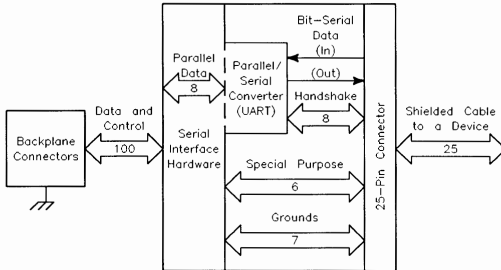
Block Diagram of the Datacomm Interface
