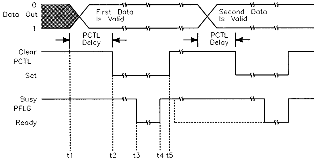
Ready Pulses with Pulse-Mode OUTPUT Handshakes
