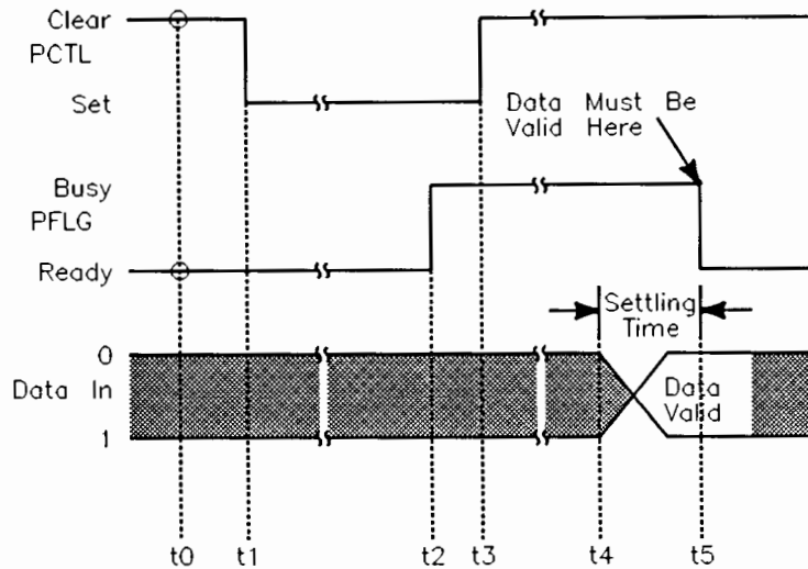
Full-Mode ENTER Handshake with RDY Clock Source
