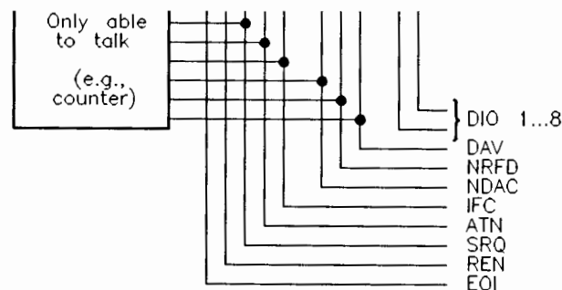
HP-IB Control Lines
