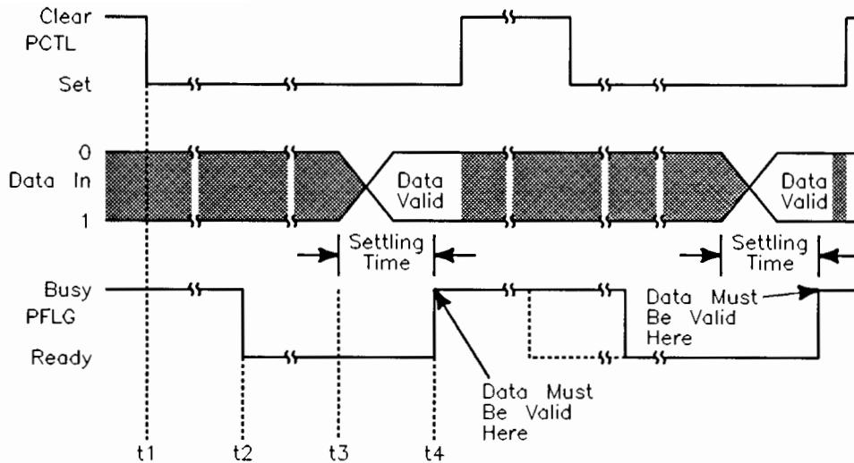
Ready Pulses with Pulse-Mode ENTER Handshakes (BSY Clock Source)
