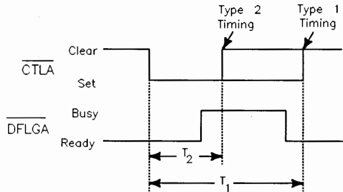
Measuring the BCD Interface's TIMEOUT Parameter
