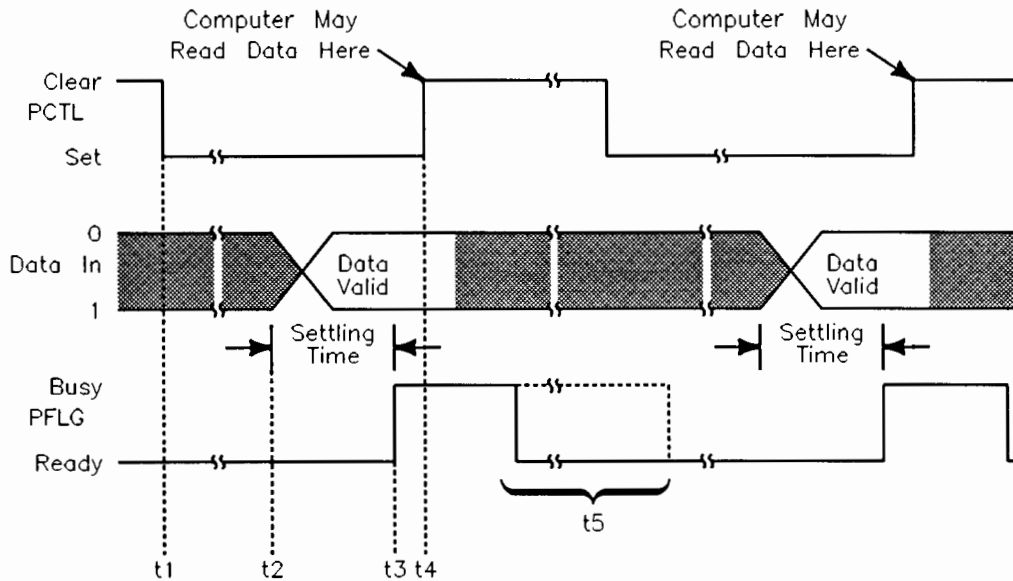
Busy Pulses with Pulse-Mode ENTER Handshakes (RDY Clock Source)
