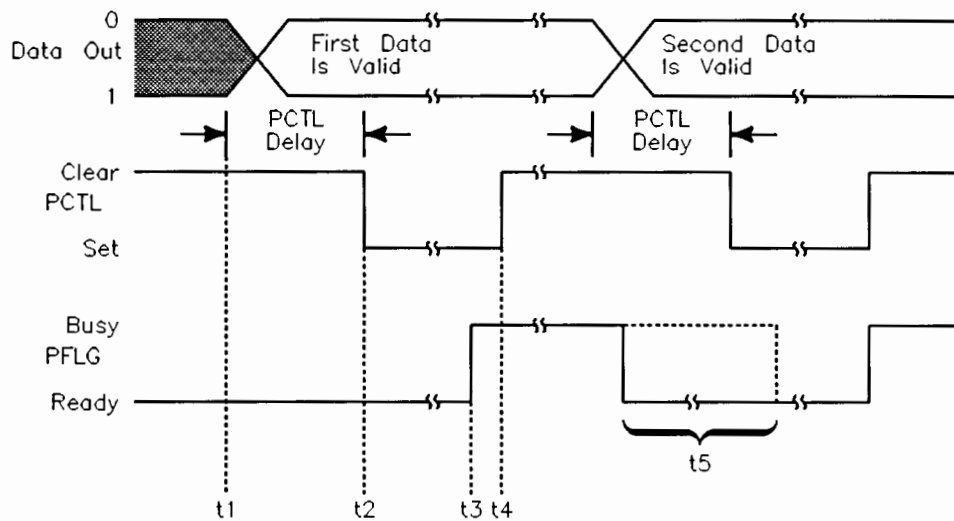
Busy Pulses with Pulse-Mode OUTPUT Handshake
