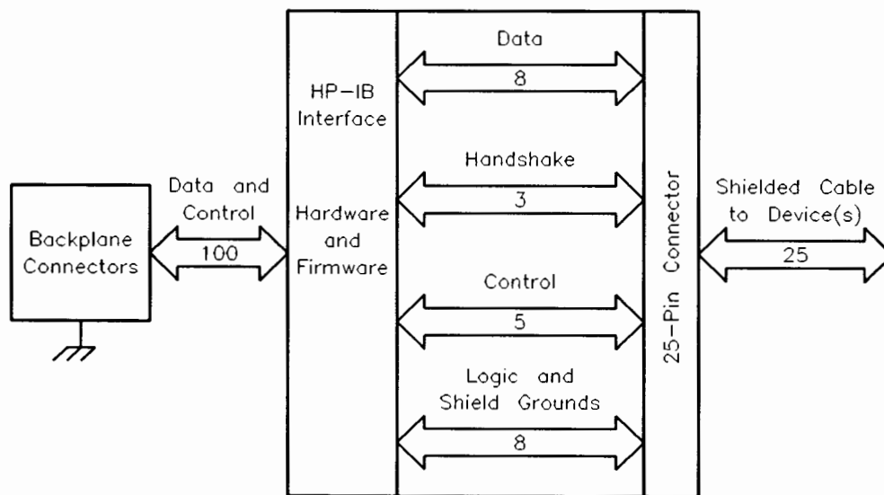
HP-IB Interface Block Diagram
