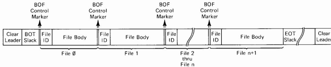
Figure 5-3. Tape Structure
