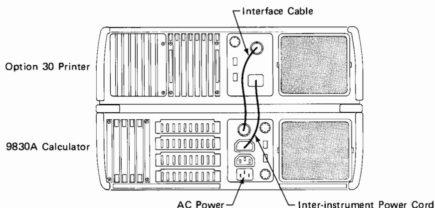
Figure A-3. Connecting the 9866A Printer
