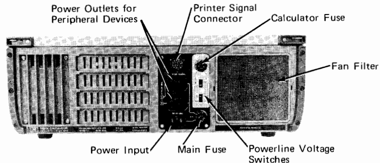
Figure A-1. The Rear Panel
