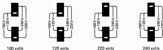
Figure A-2. Switch Settings for the Nominal Powerline Voltages
