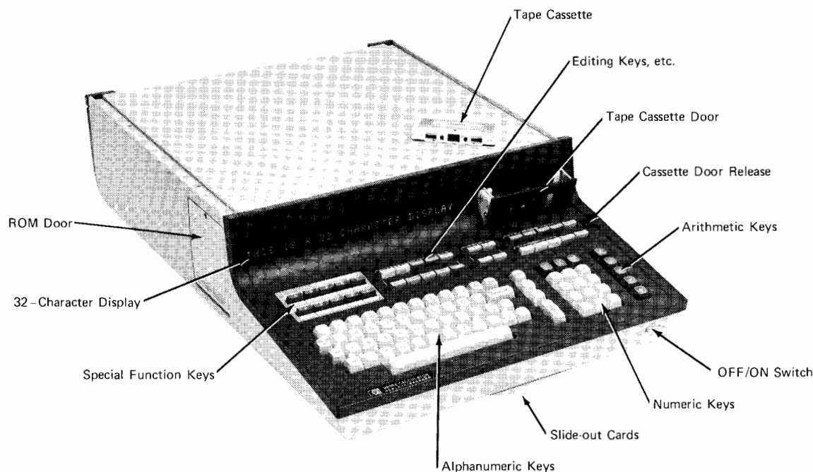
Figure 1-1. The Model 30 Calculator
