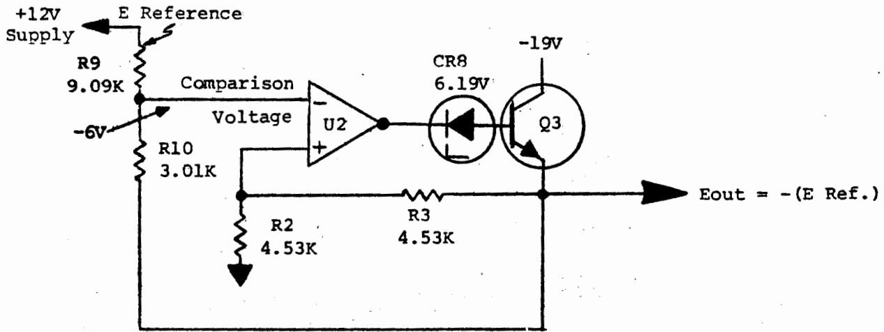
Figure 6-6. -12V Simplified Schematic
