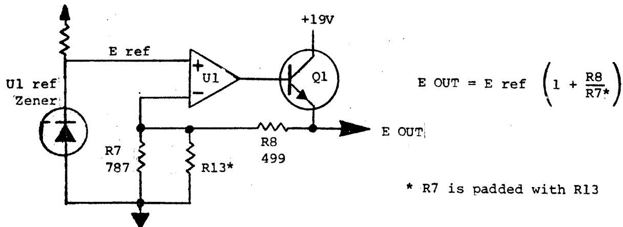
Figure 6-5. +12V Power Supply
