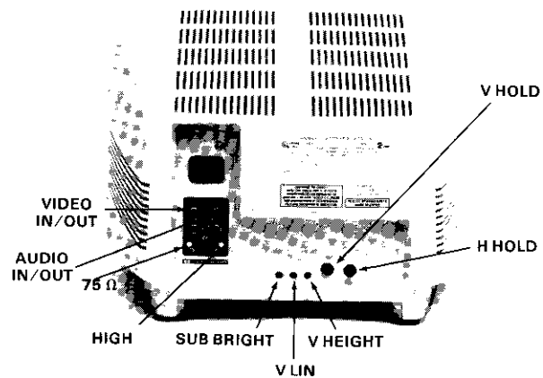
HP 82913A Video Monitor (12-inch)
