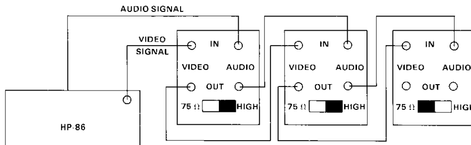
With an HP 82913A Video Monitor:
