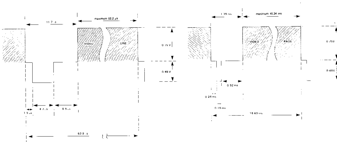
Vertical Composite Waveform
