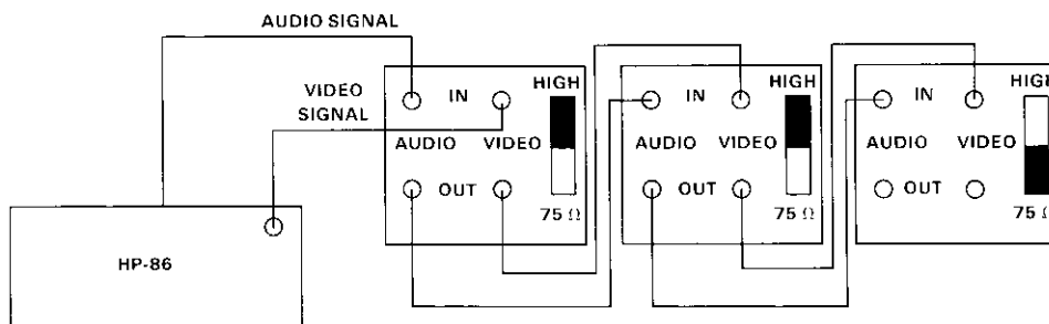
With an HP 82912A Video Monitor:
