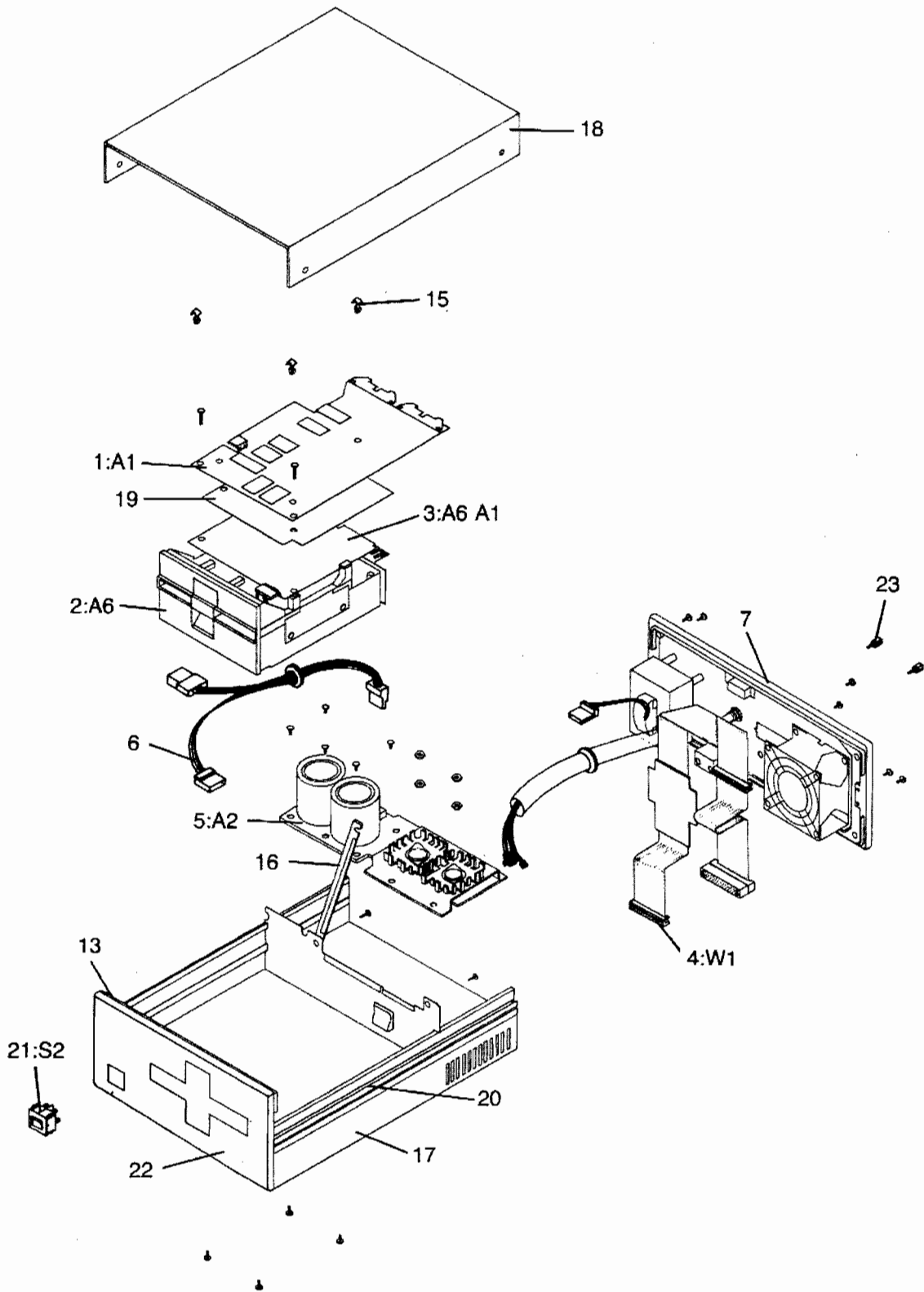
Figure 5-1. 82900 Exploded View
