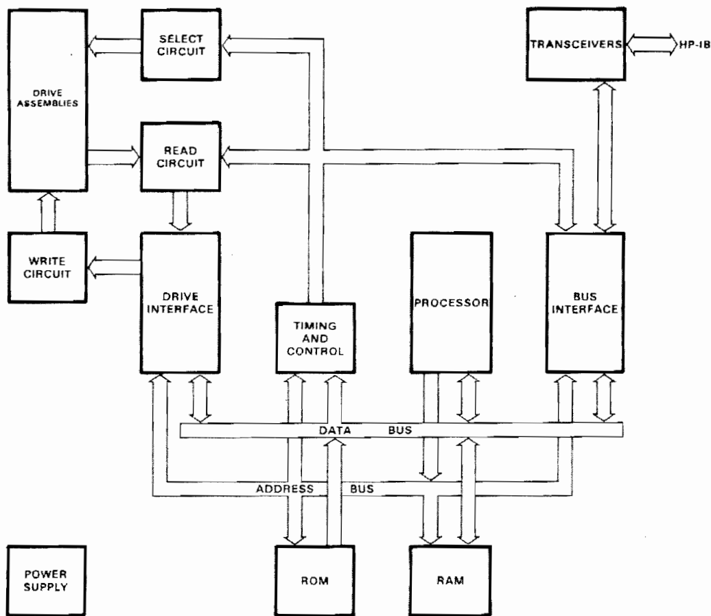
Figure 2-1. Flexible Disc Drive Controller Block Diagram
