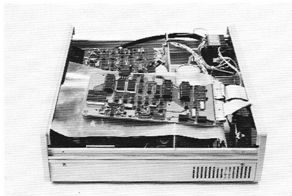
Figure 4-2. Substituting a Controller PCA
