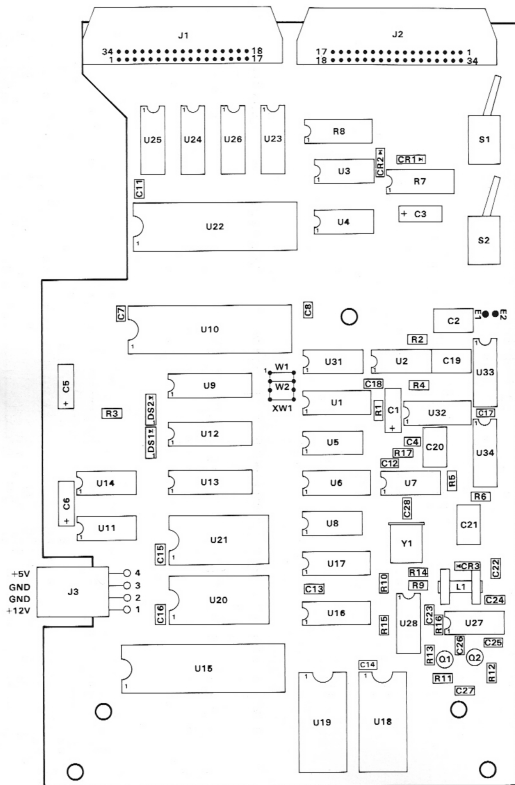
Figure 6-1. Controller PCA Component Location Diagram (P/N 82901-69002)
