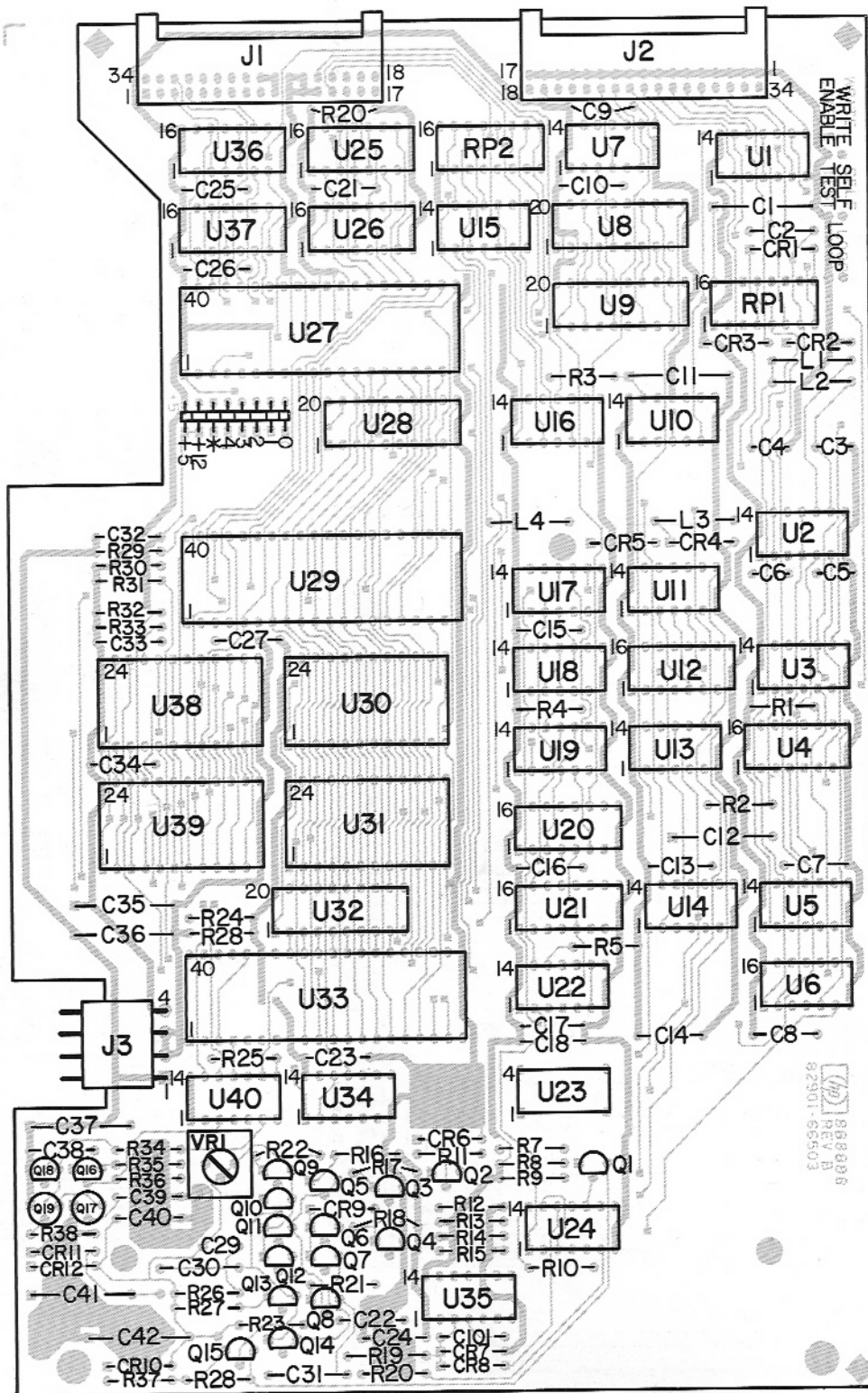
Figure 6-3. Controller PCA Component Location Diagram (P/N 82901-66503)
