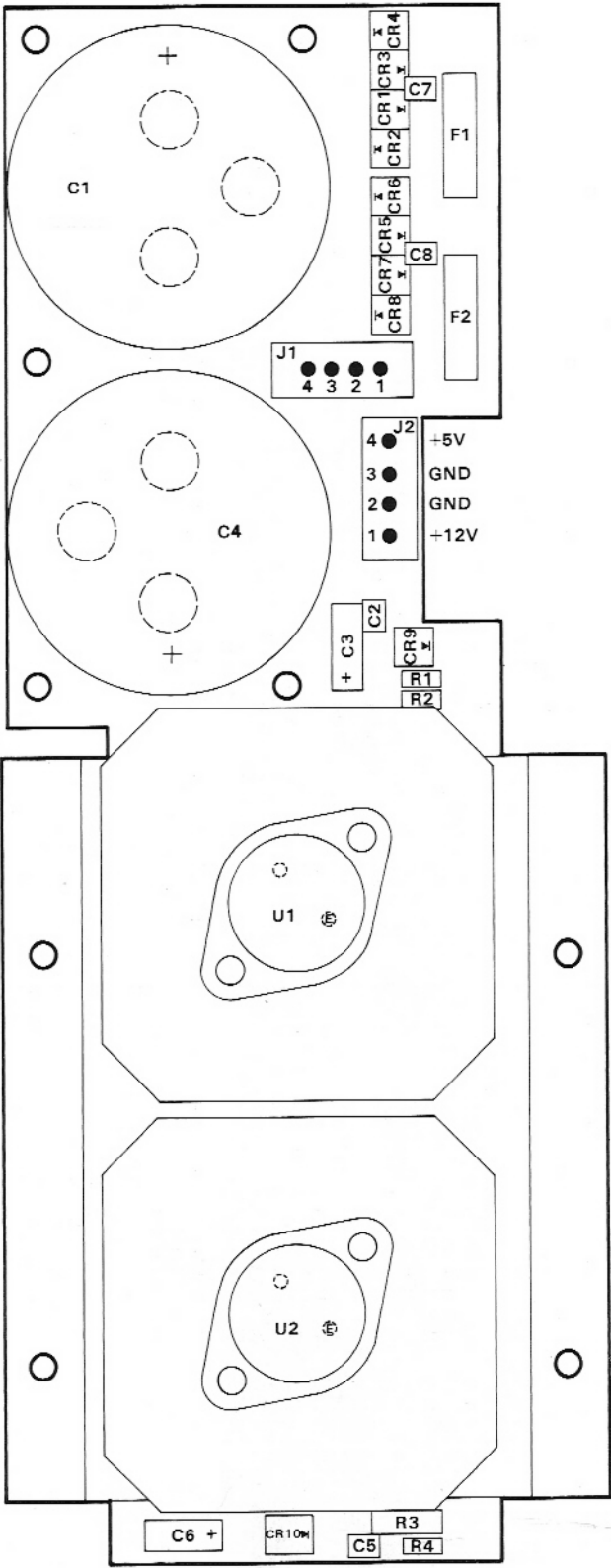
Figure 6-5. Power Supply Component Location Diagram
