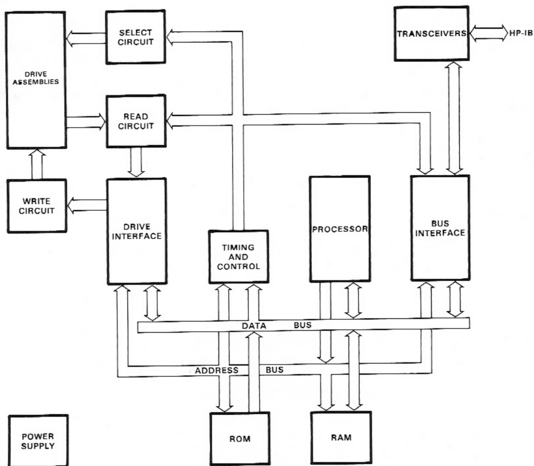
Figure 2-1. Flexible Disc Drive Controller Block Diagram
