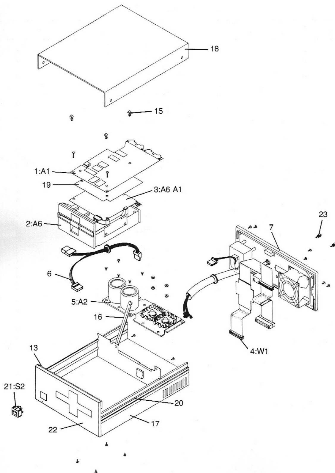
Figure 5-1. 82900 Exploded View
