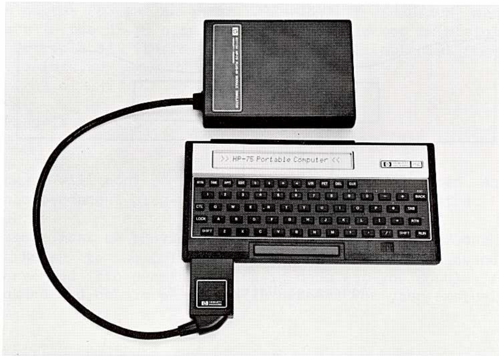
The HP 82713A Plug-In Module Simulator System
