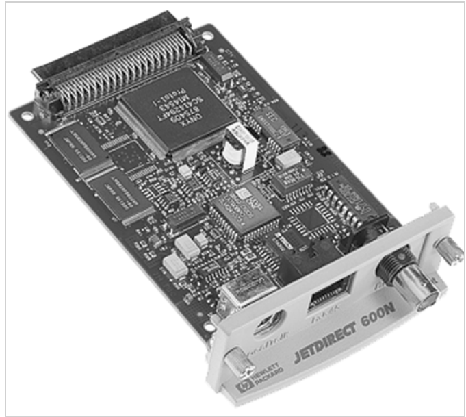
Typical EIO Card (not to scale)
