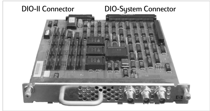
Typical DIO-II Card.
