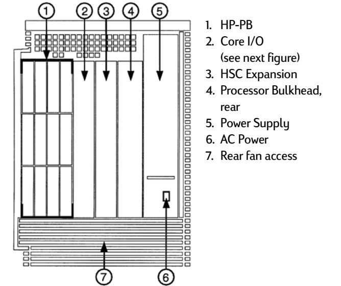
K-Class Rear Slots and Bays
