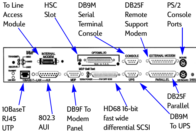
K-Class Core I/O
