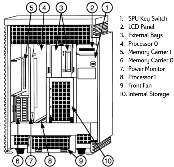
K-Class Front Slots and Bays
