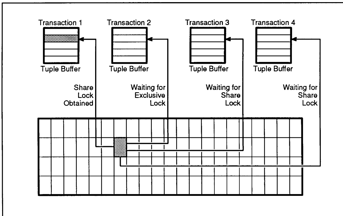
Figure 5-7. Lock Requests 1: Waiting for Exclusive Lock
