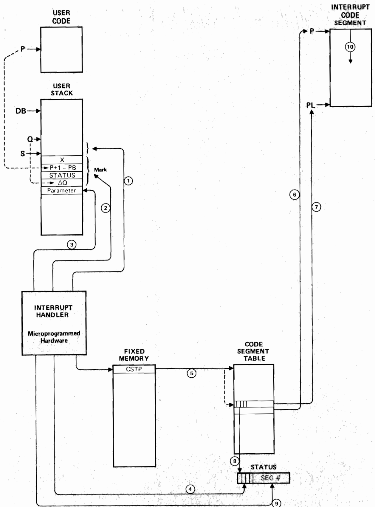
Figure 7-9. Non-ICS Internal Interrupt Operations
