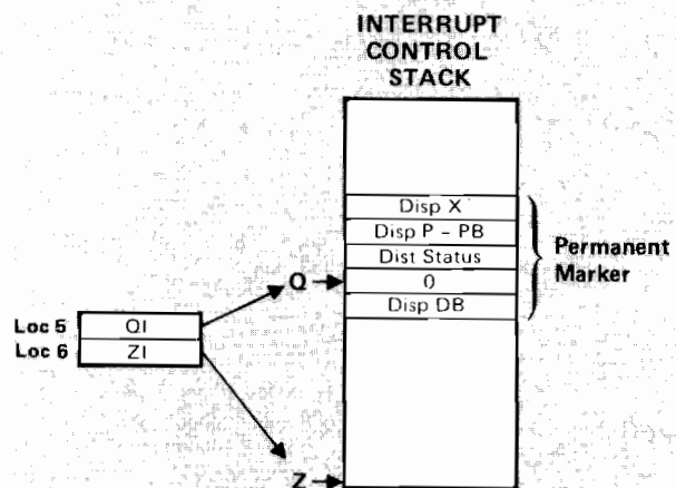
Figure 7-1. Dispatcher Marker on ICS
