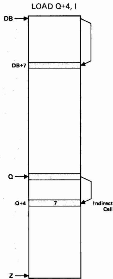
Figure 3-9. Examples of Indirect Addressing
