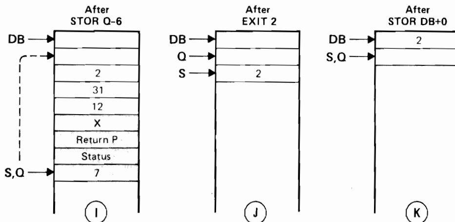
Figure 4-14. Executing a Simple Procedure
