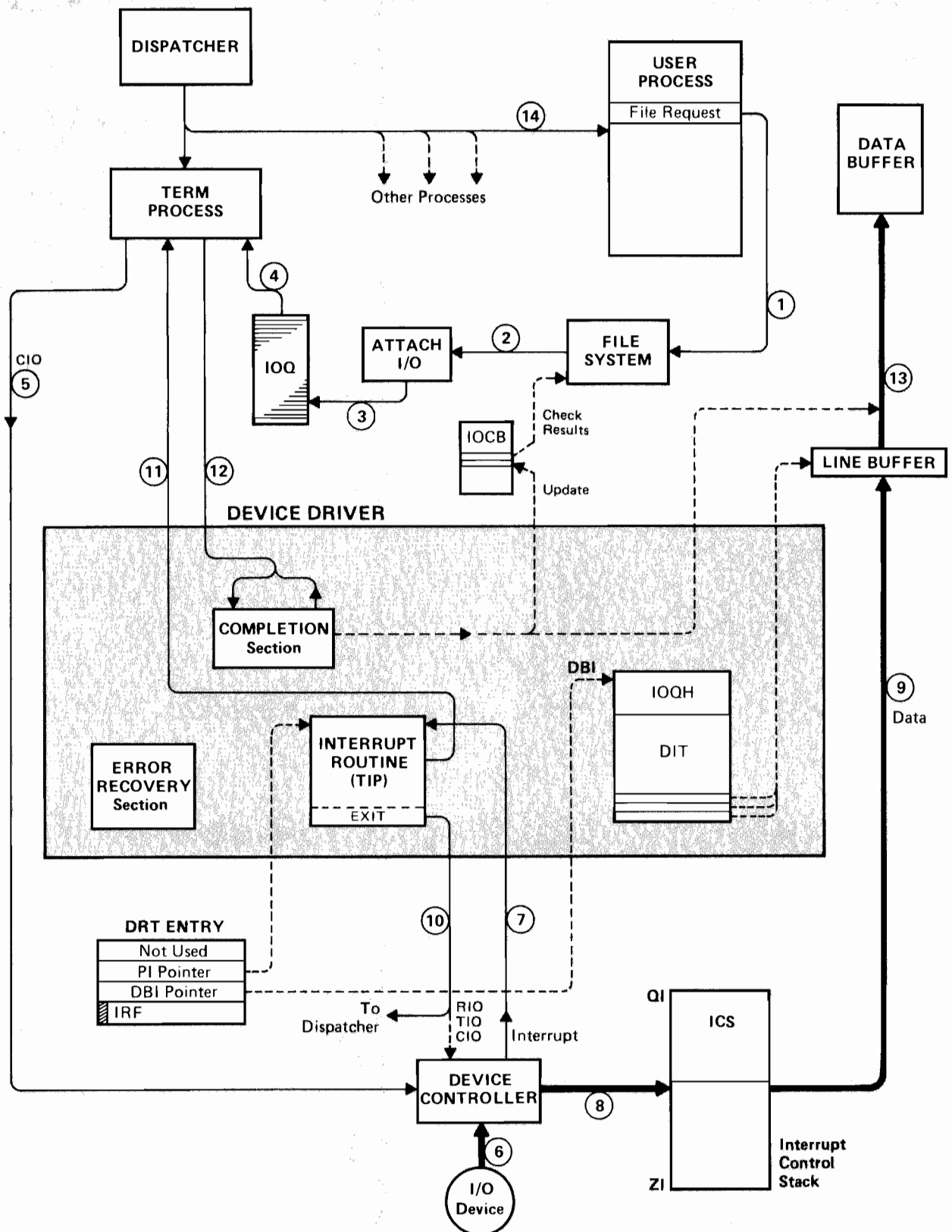
Figure 6-6. Direct Read for Terminal Devices
