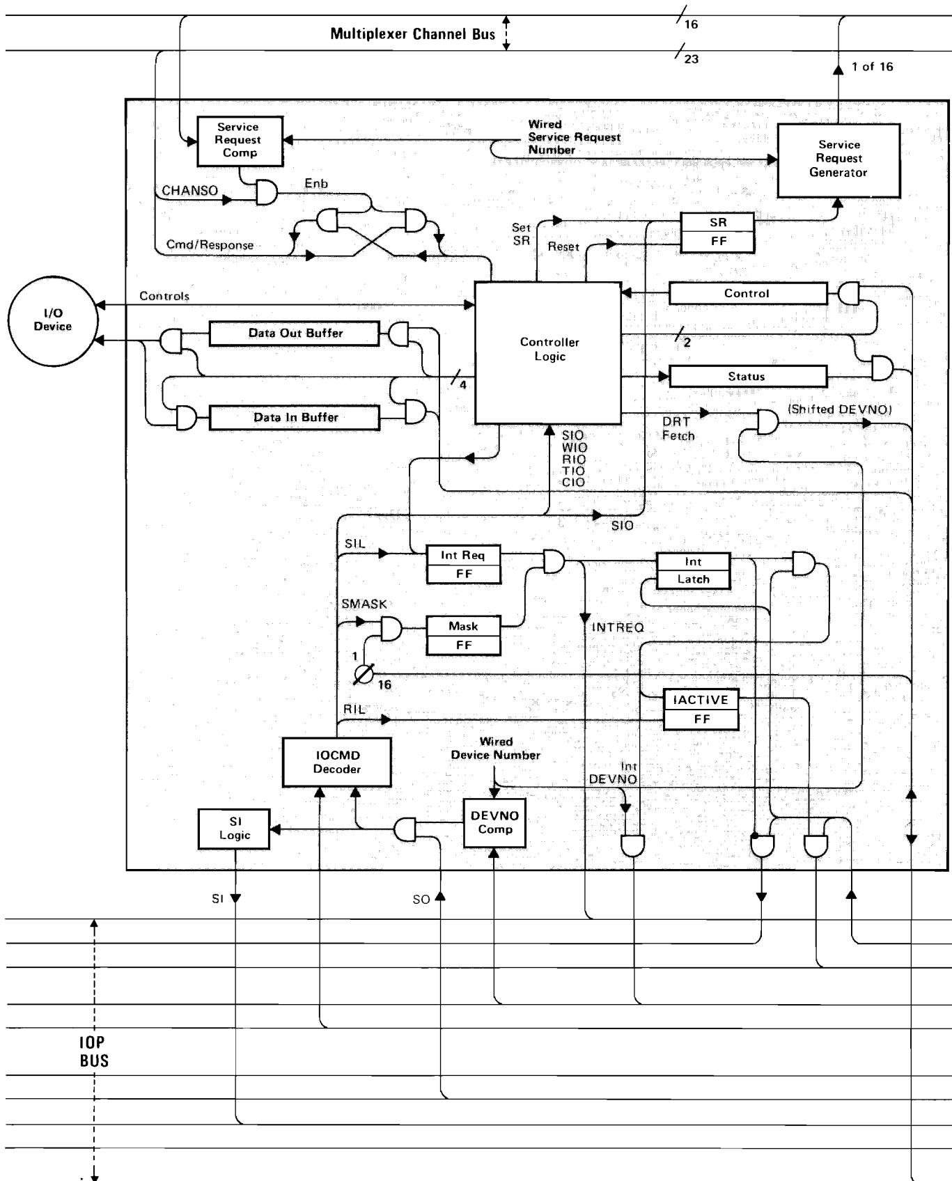
Figure 8-12. Multiplexer Channel Device Controller
