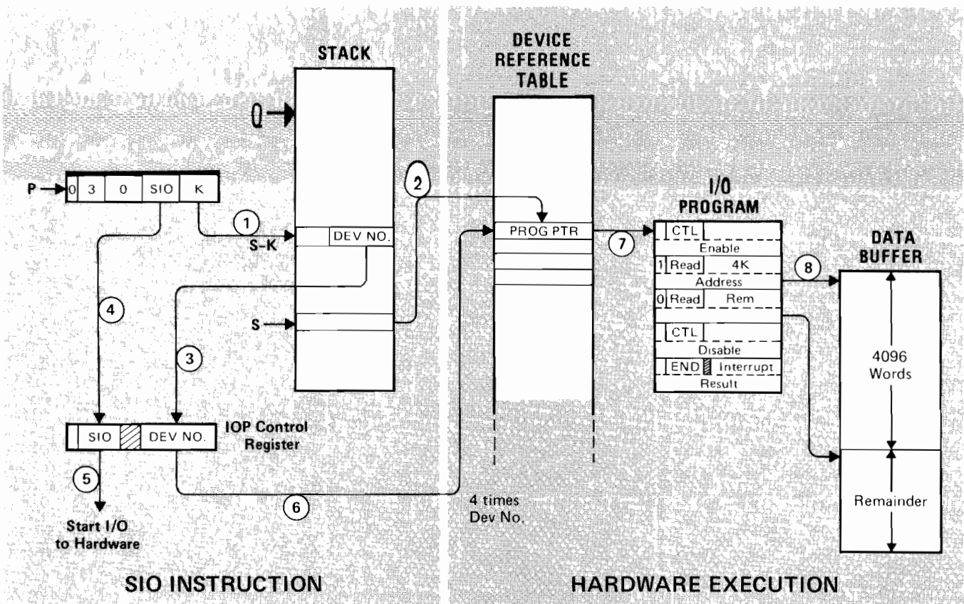
Figure 6-11. I/O Program Operation
