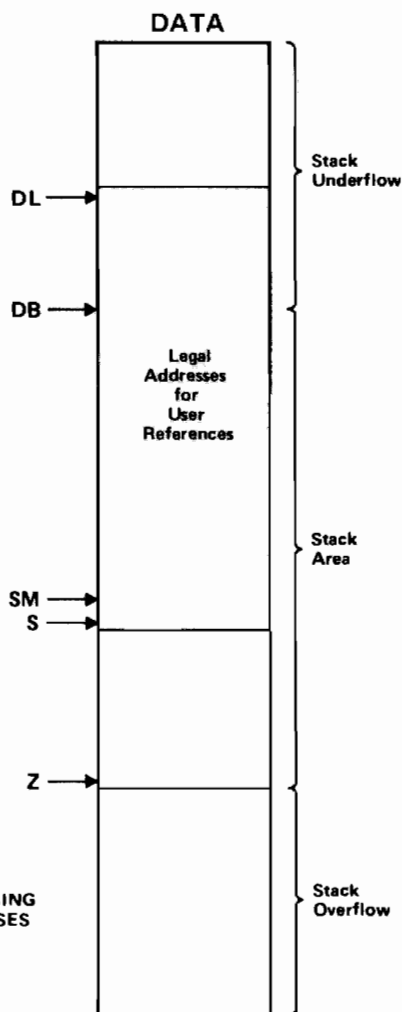
Figure 3-12. Addressing and Stack Bounds
