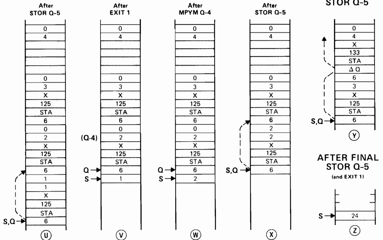
Figure 4-17. Recursive Exits
