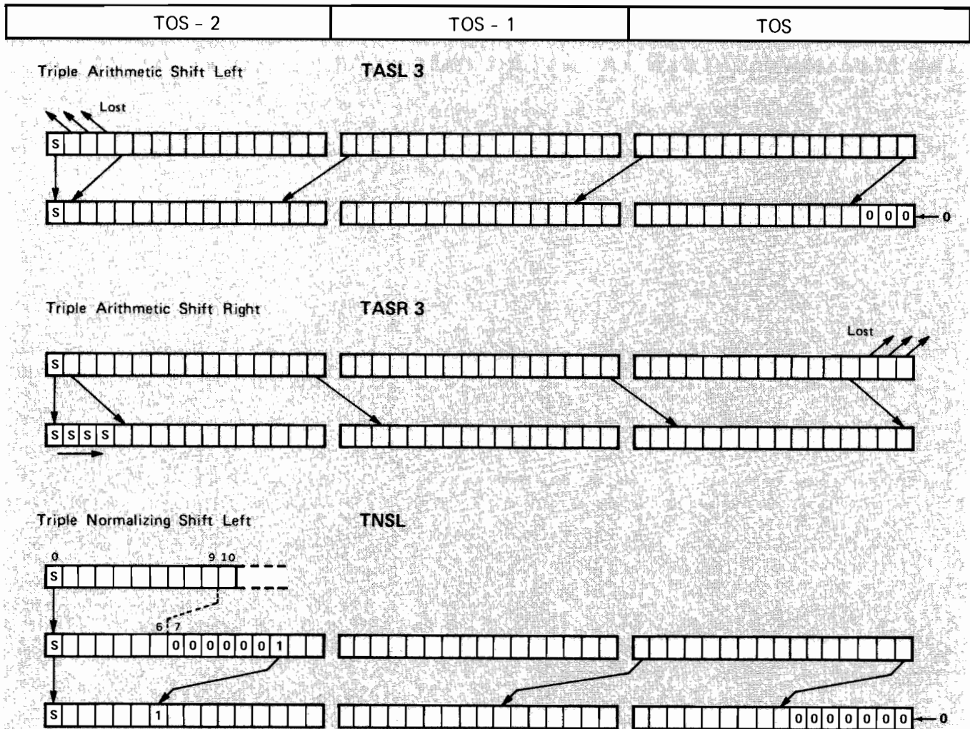
Figure 5-6. Triple Word Shifts
