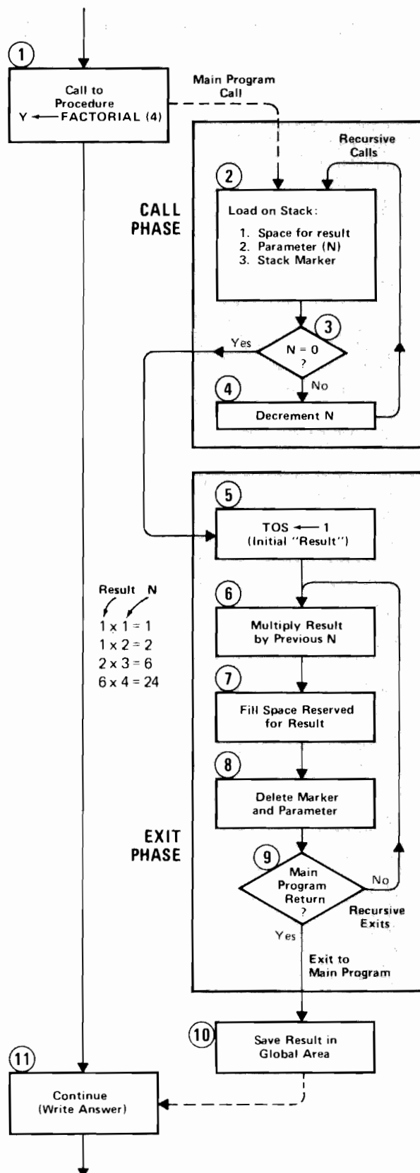
Figure 4-15. Example of Recursive Procedure
