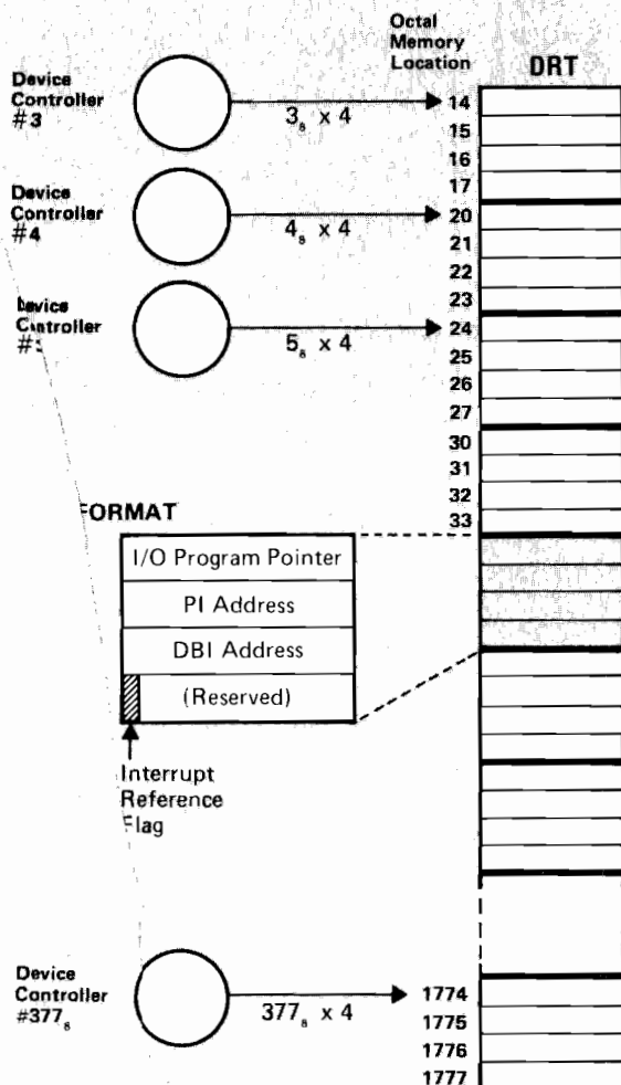
Figure 6-4. Device Reference Table
