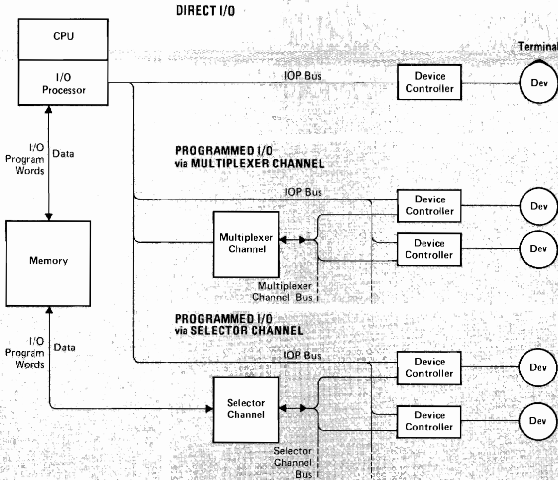
Figure 6-9. Hardware I/O Elements
