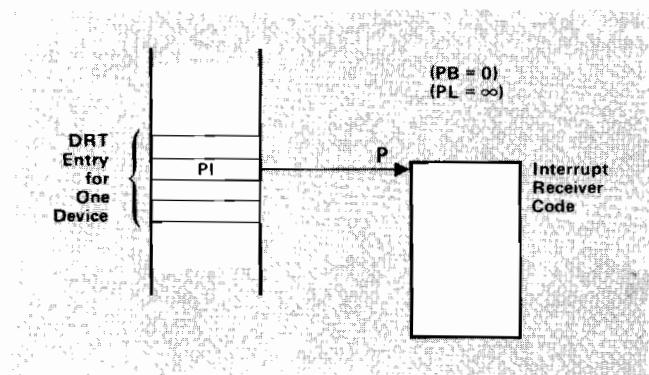
Figure 7-4. Interrupt Program Pointer
