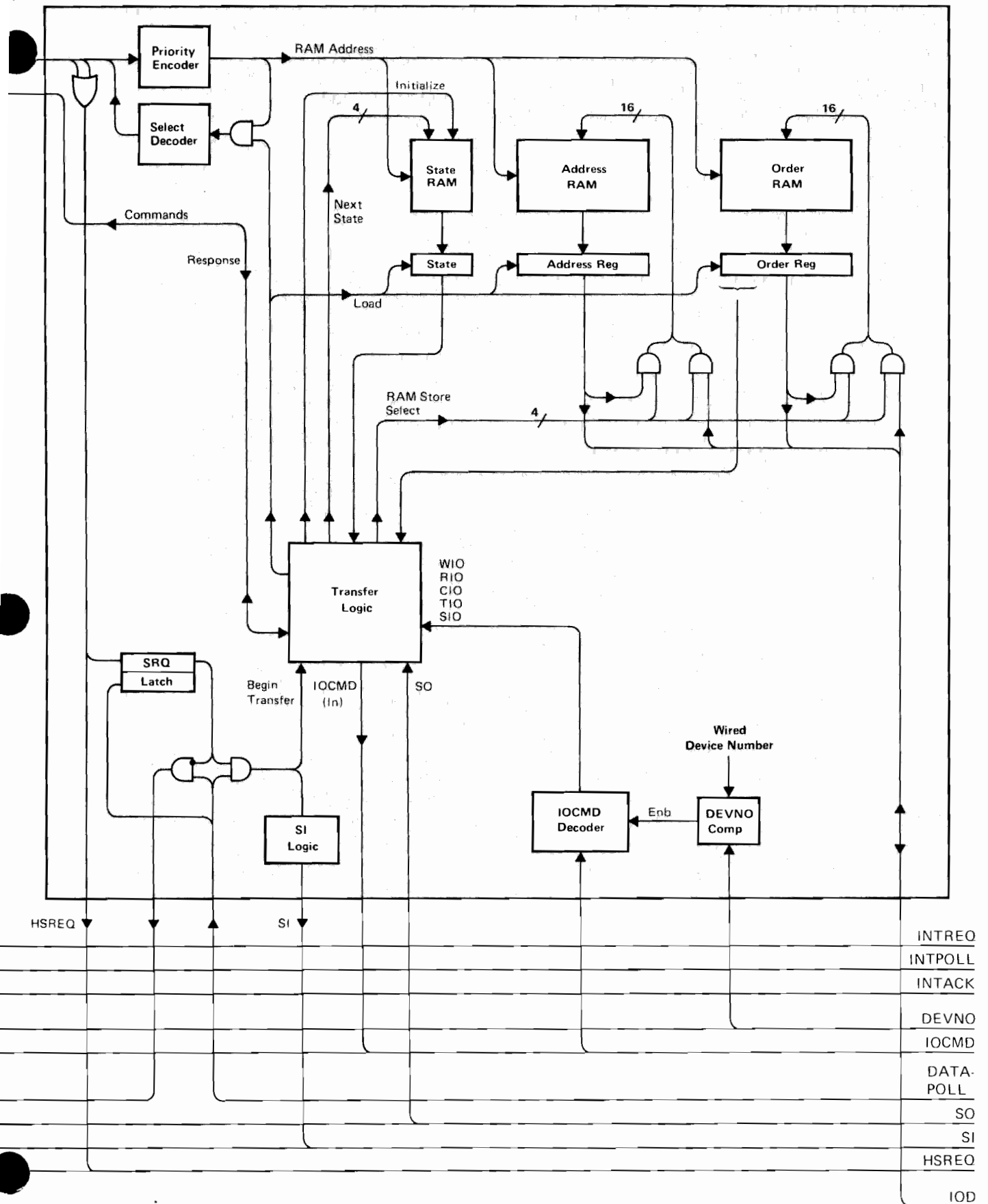
Figure 8-13. Multiplexer Channel
