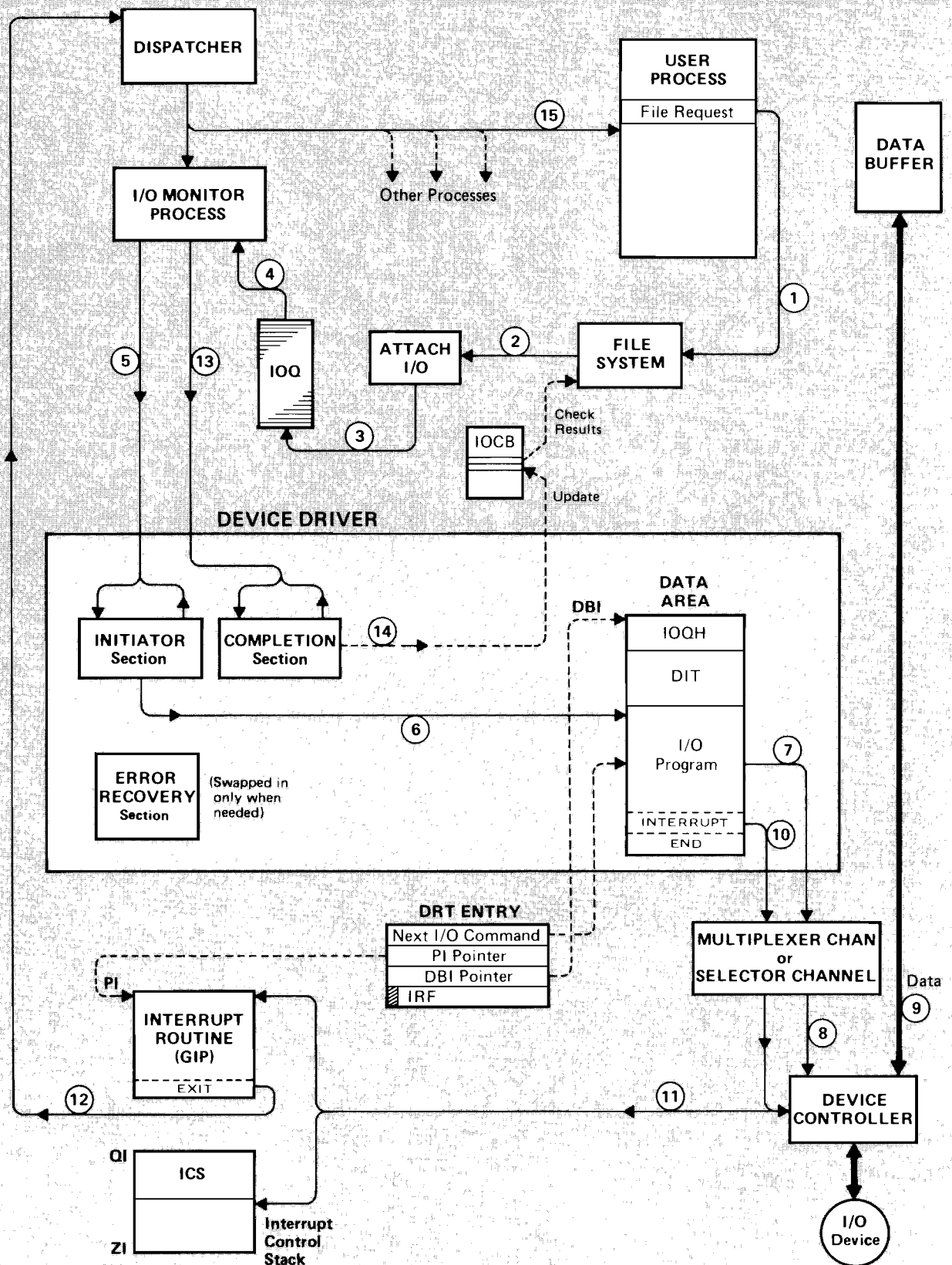
Figure 6-5. I/O System Overview
