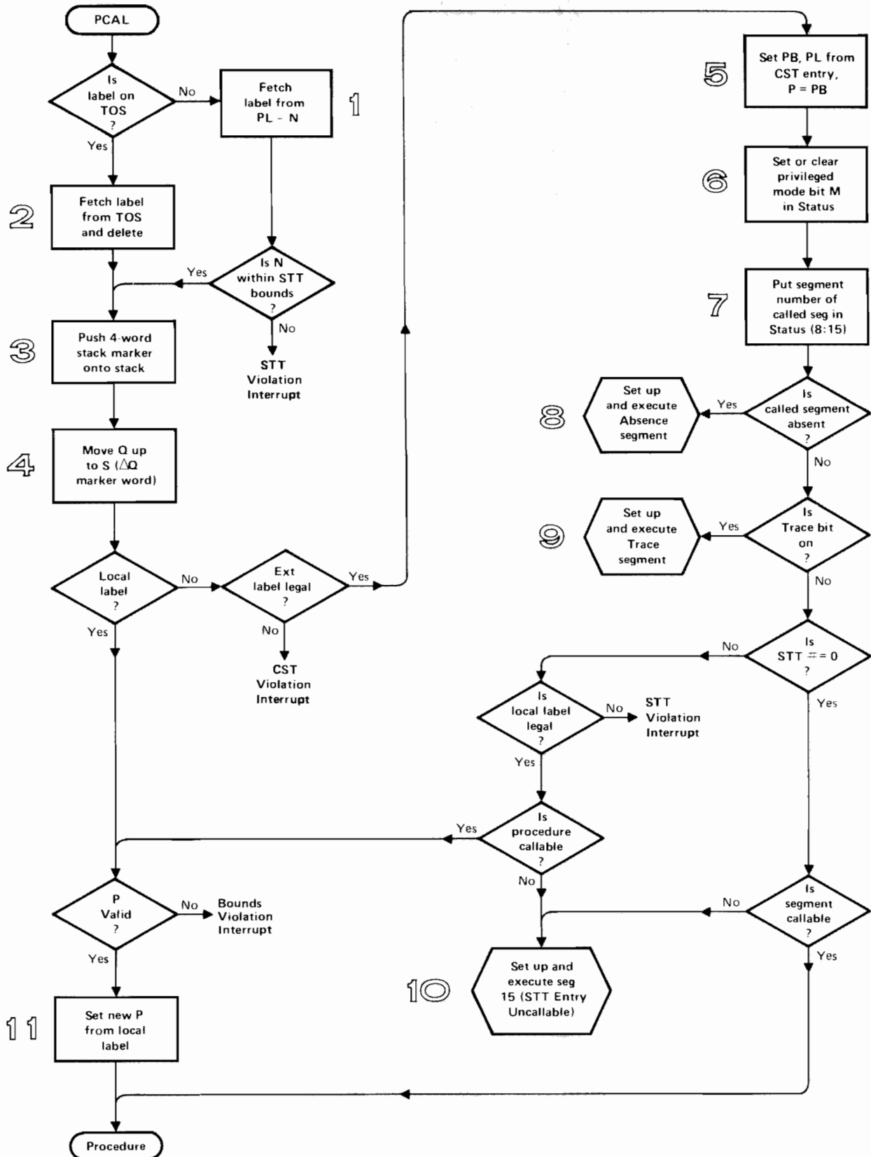
Figure 5-13. Operations of PCAL
