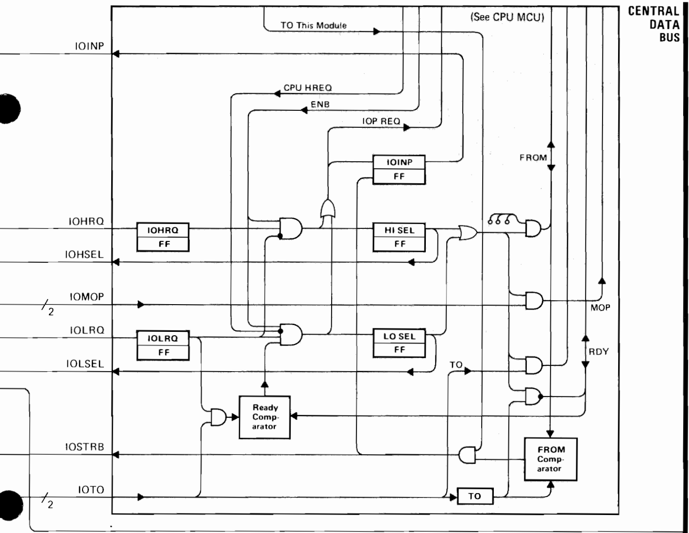
Figure 8-11. IOP Module Control Unit
