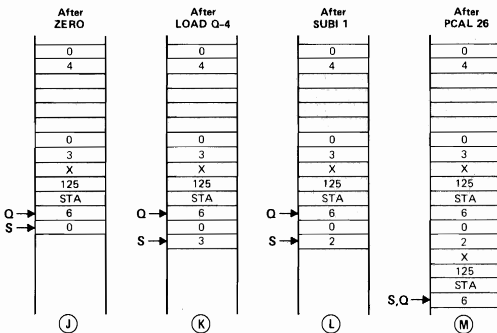
Figure 4-16. Recursive Calls
