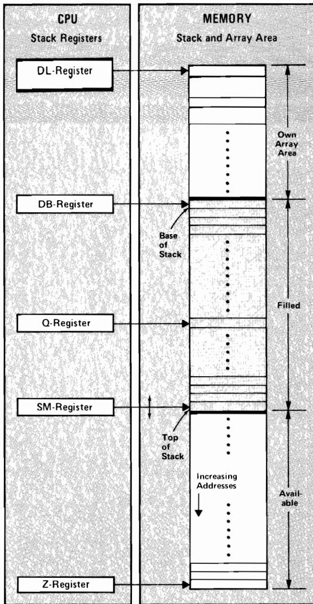
Figure 4-8. Stack Registers and One Stack
