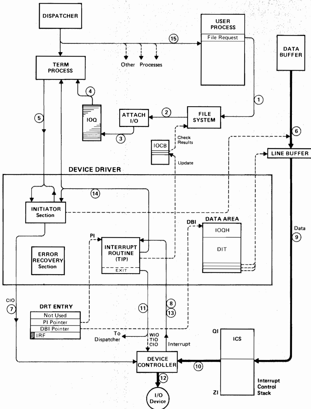
Figure 6-7. Direct Write for Terminal Devices
