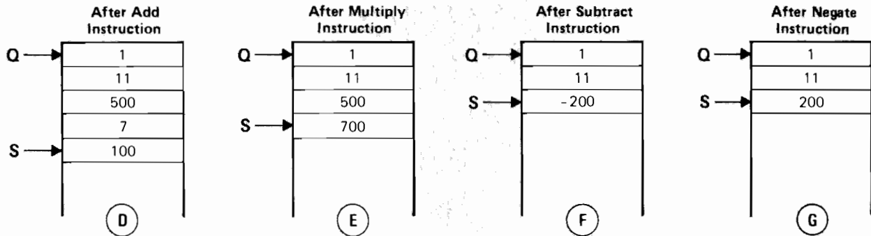
Figure 4-12. Basic Arithmetic Stack Operations
