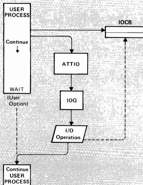
Figure 6-8. Blocked and Unblocked I/O
