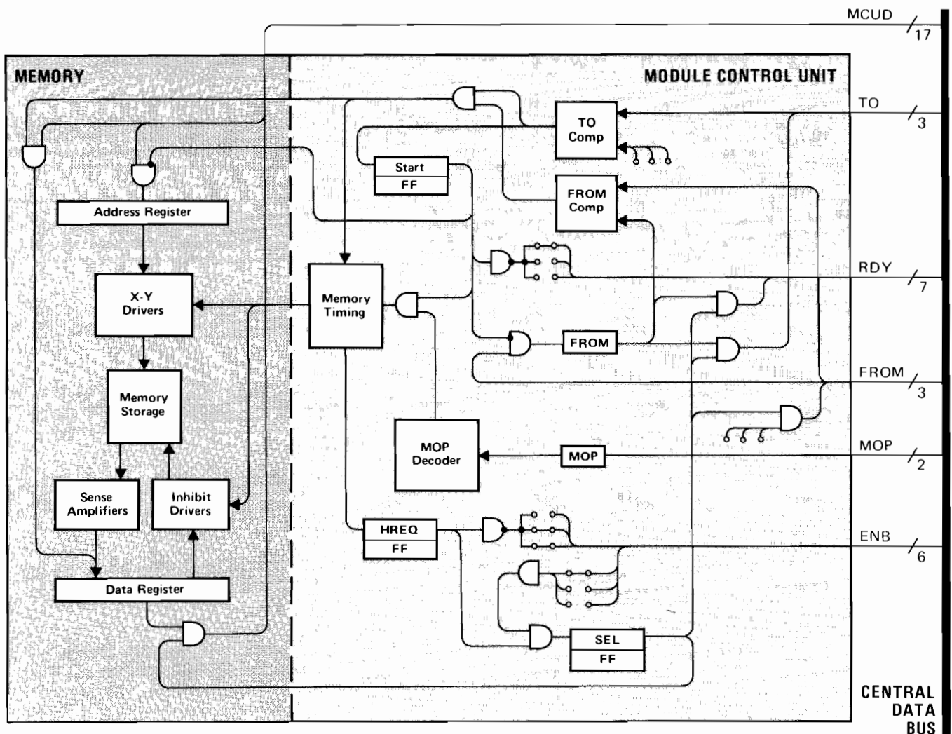
Figure 8-6. A Typical Memory Module
