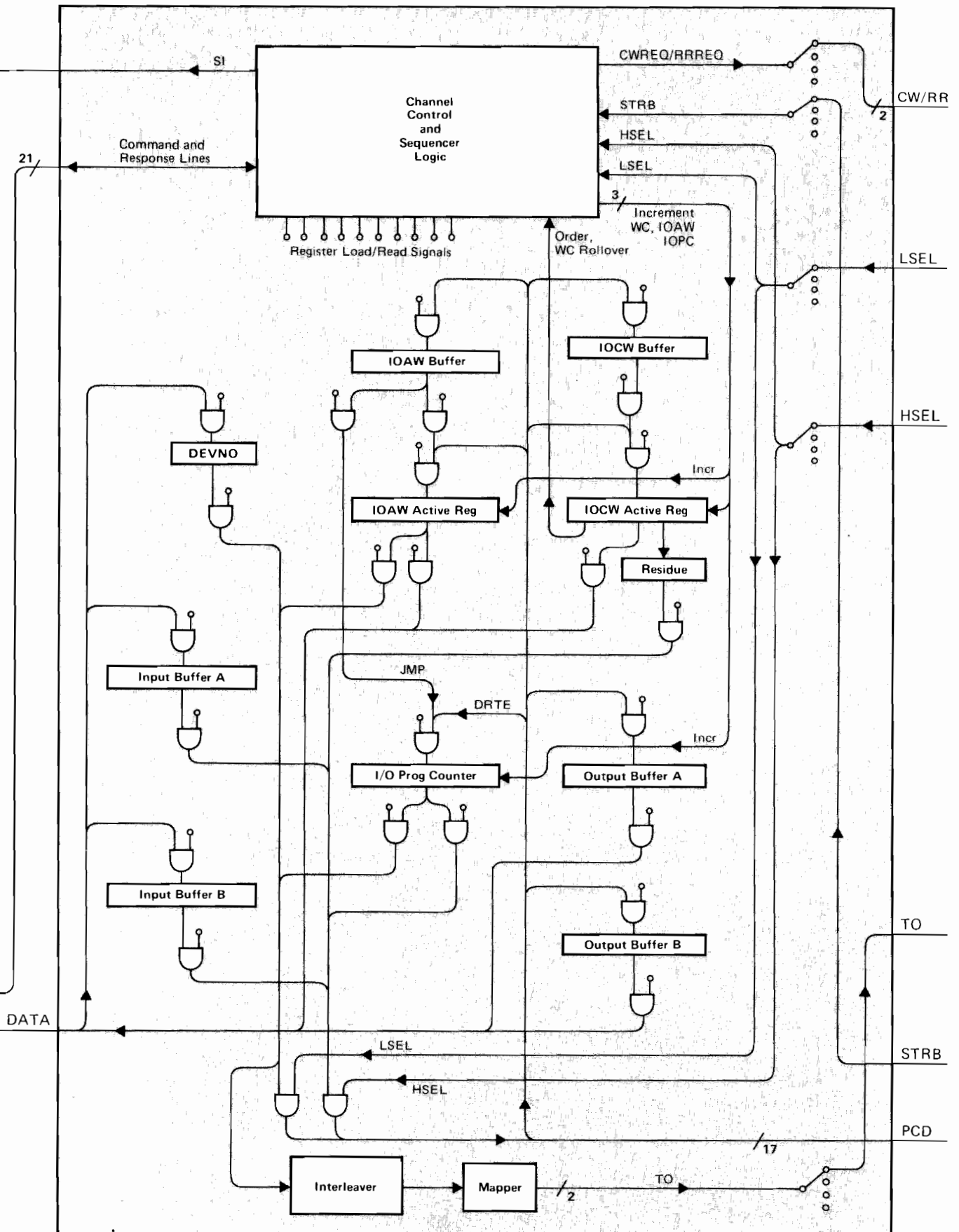
Figure 8-16. Selector Channel
