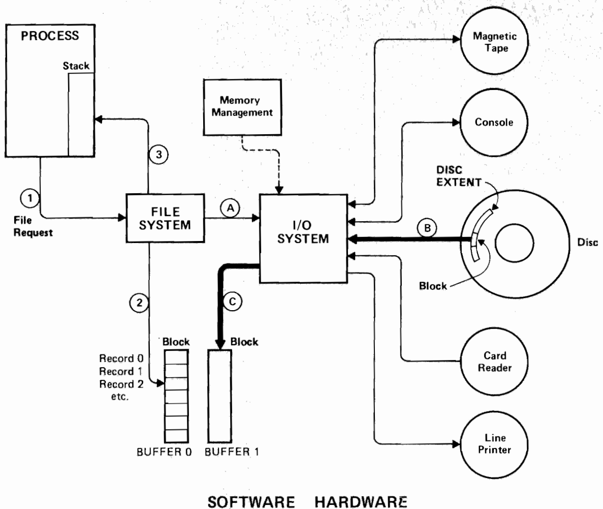
Figure 6-2. File System Basic Operation
