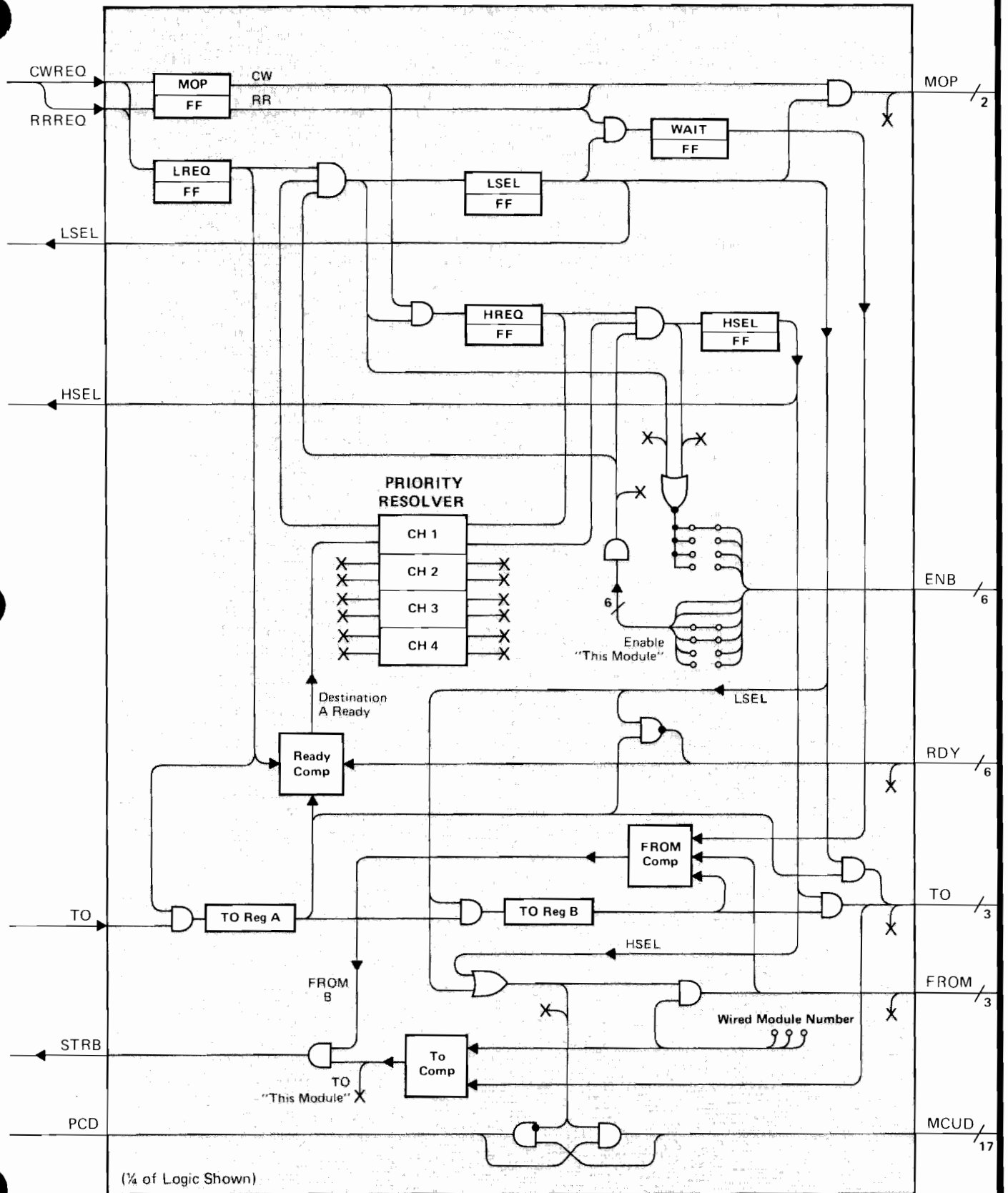
Figure 8-14. Port Controller
