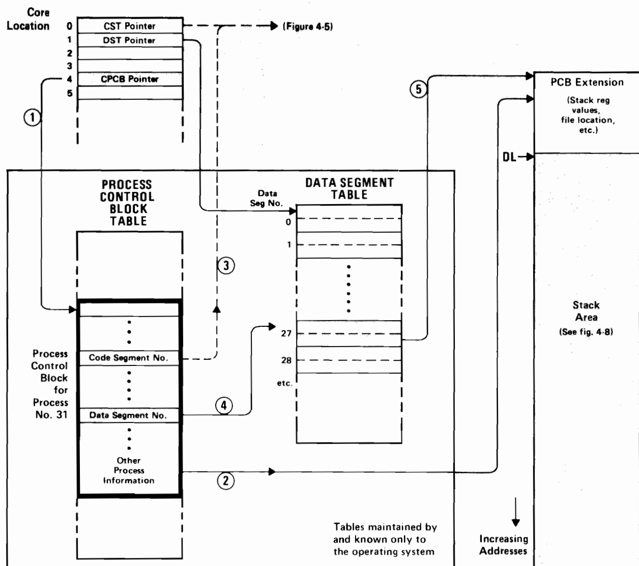
Figure 4-7. Locating the Stack for One Process
