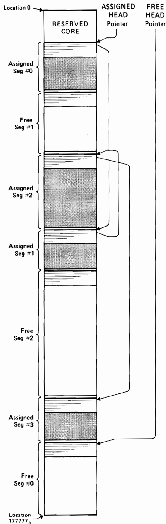
Figure 4-4. Main Memory Links
