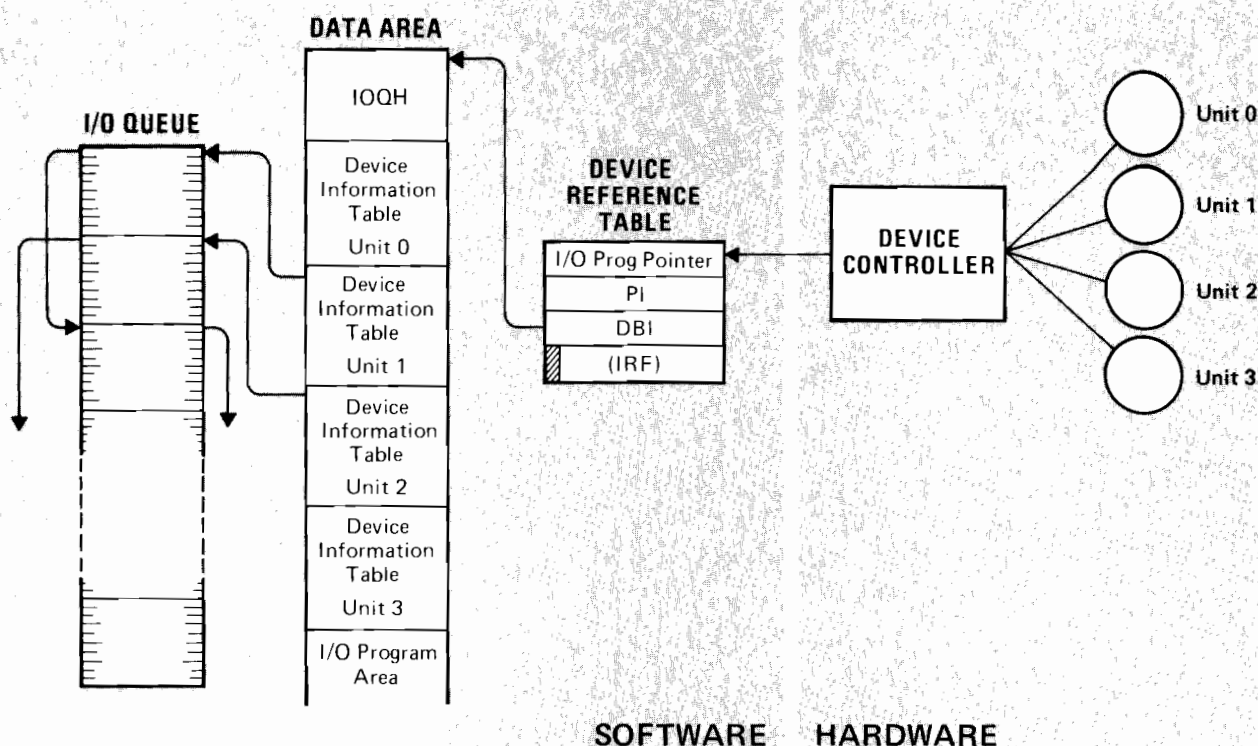
Figure 6-3. Fundamental Elements of I/O System
