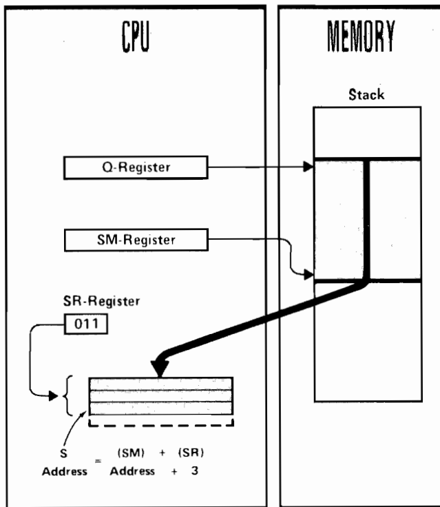
Figure 4-9. Top-of-Stack in the CPU
