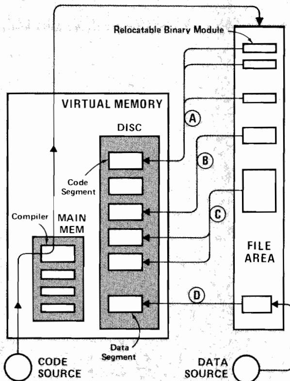
Figure 4-2. Sources of Segments
