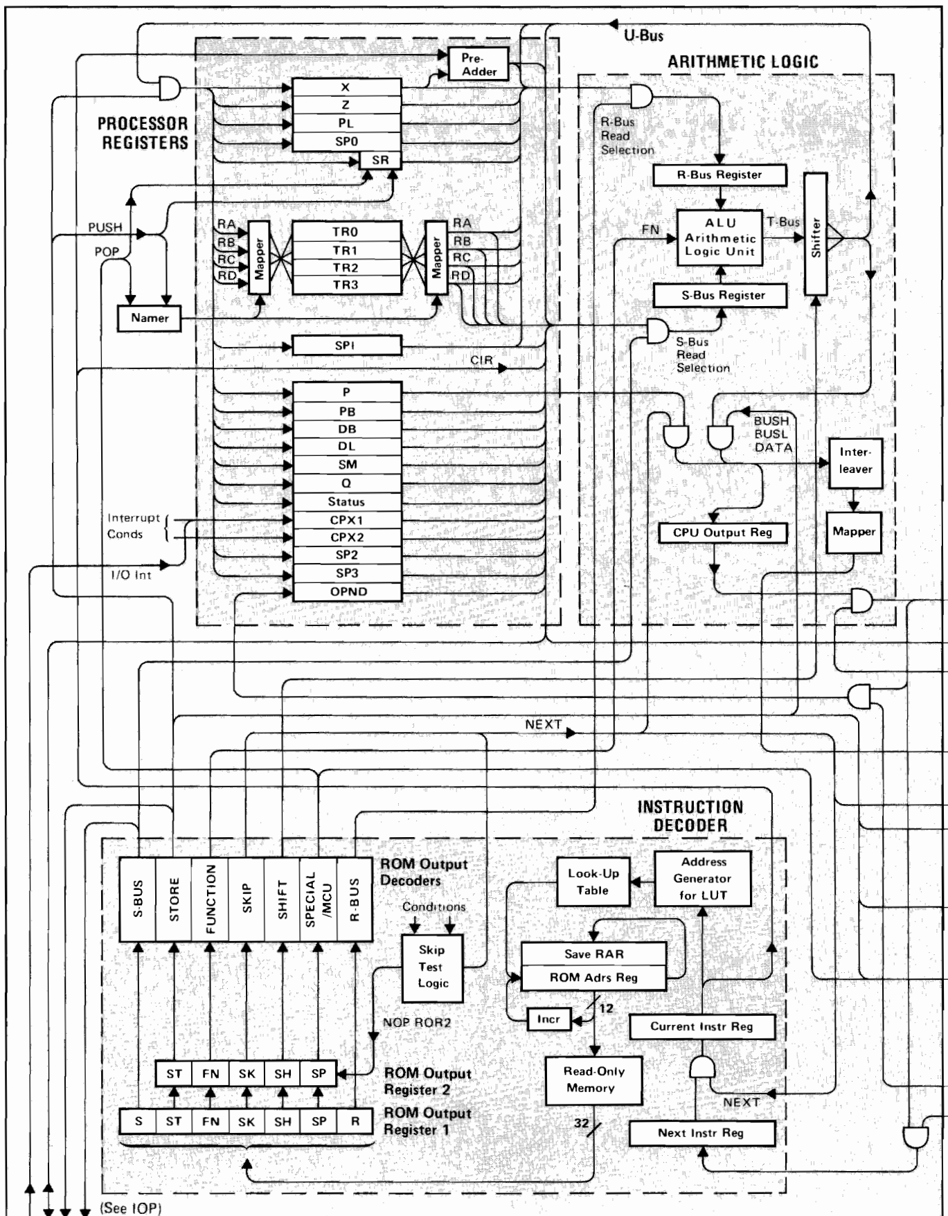
Figure 8-3. Central Processor Unit
