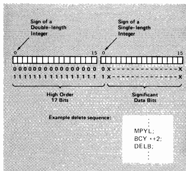
Figure 5-1. Deleting a High Order Word
