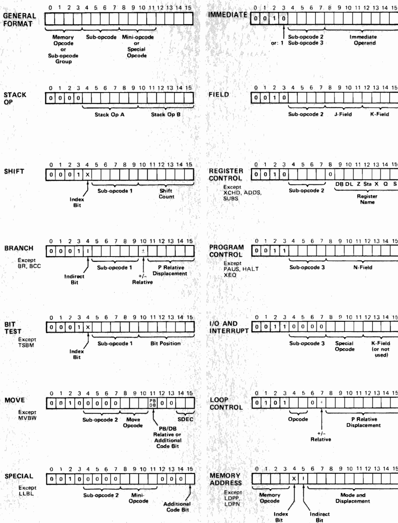
Figure 3-5. Instruction Formats
