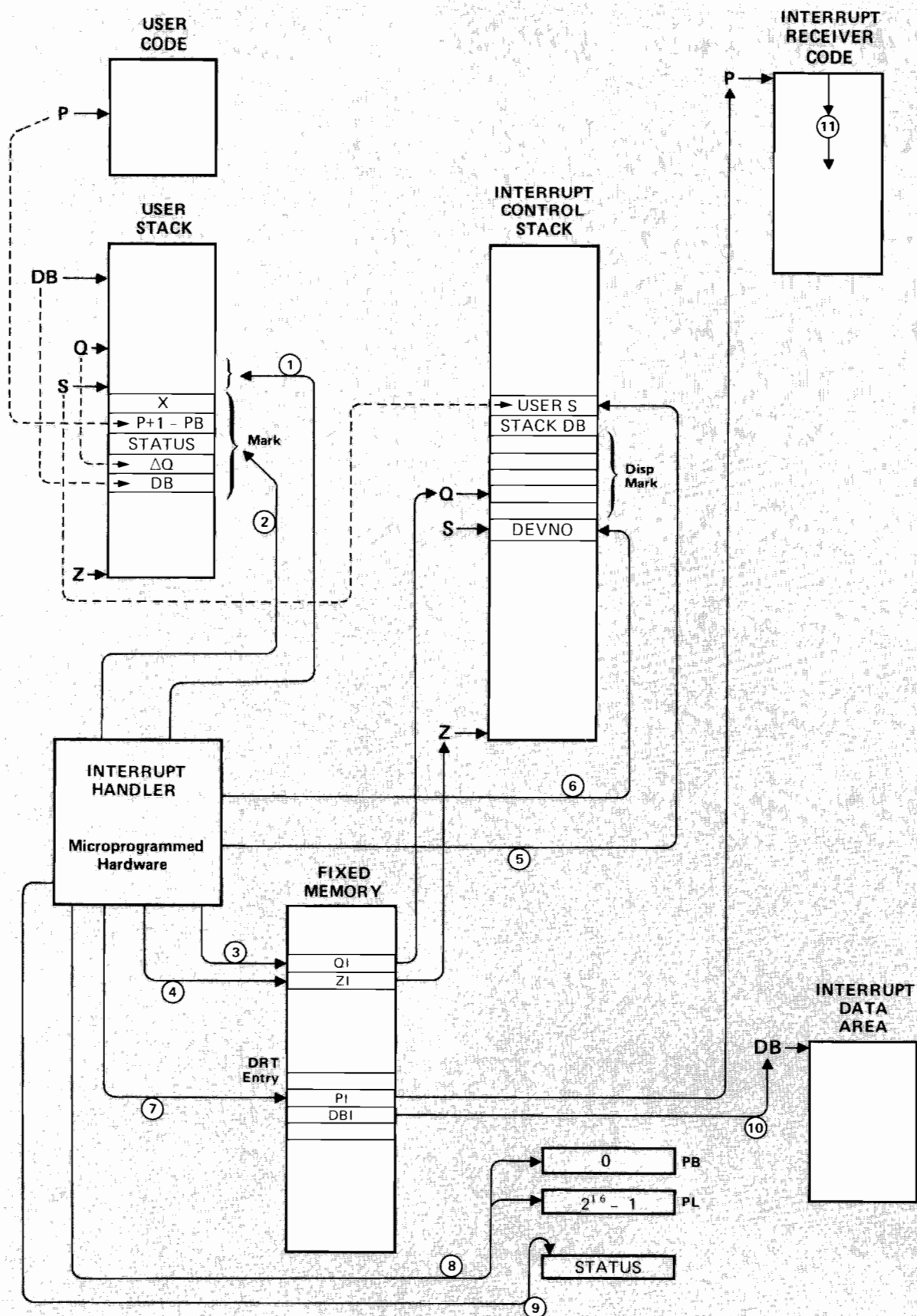
Figure 7-5. External Interrupt Operations
