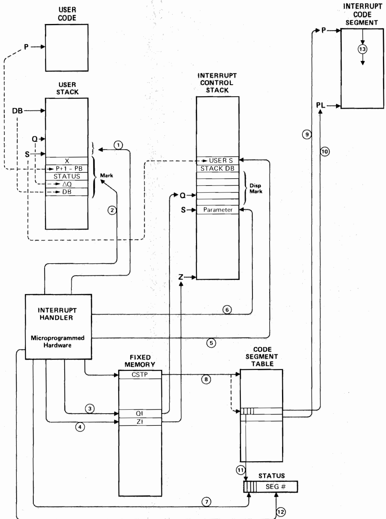
Figure 7-8. ICS Internal Interrupt Operations
