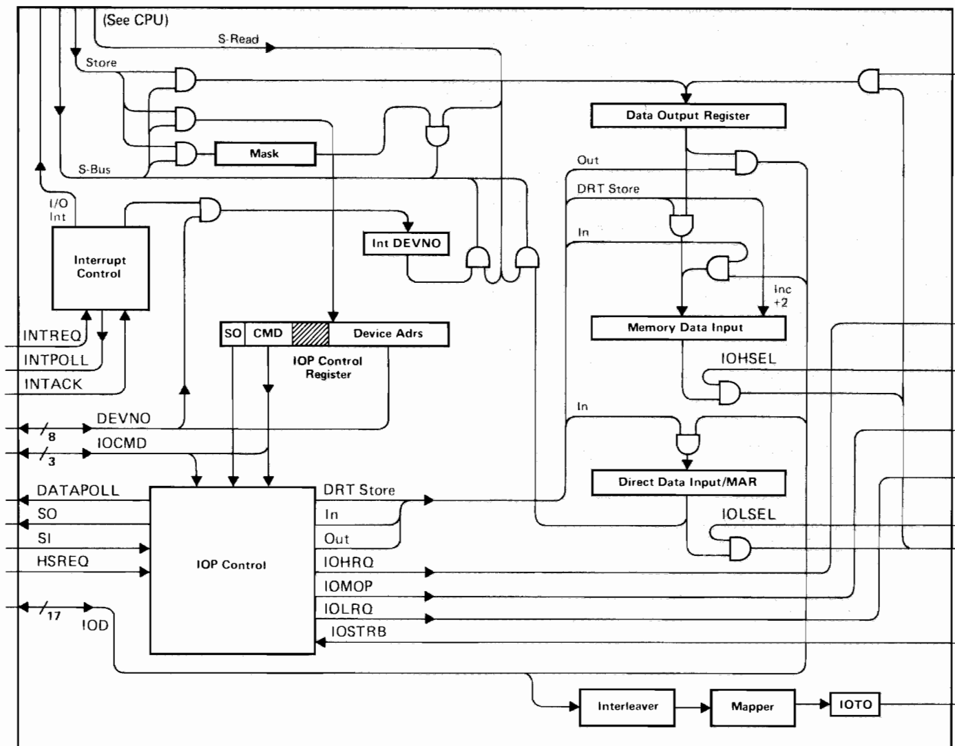
Figure 8-10. I/O Processor
