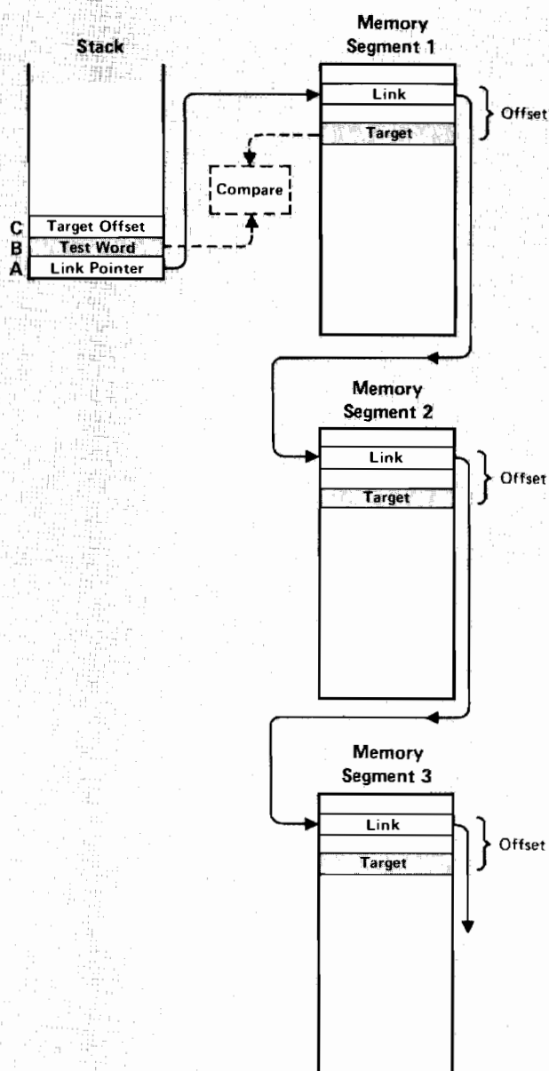
Figure 5-10. LLSH Operation
