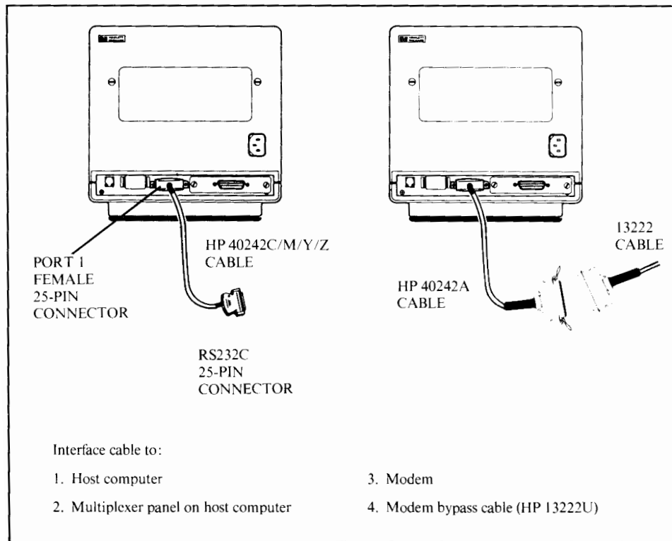
Figure 6-2. Terminal Cabling (HP 40242 and 13222 Cables)
