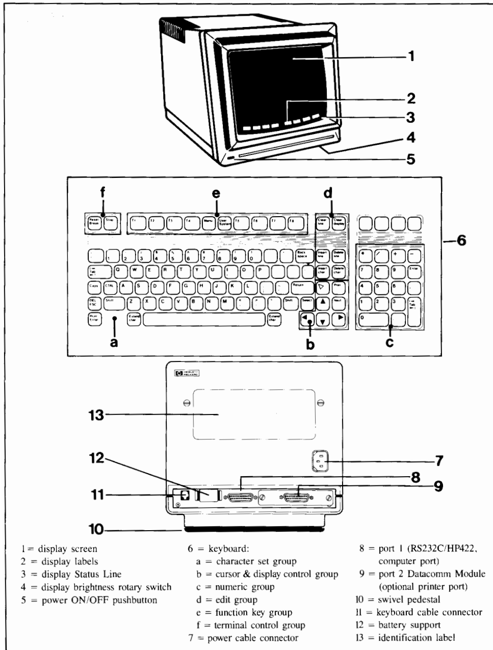
Figure 1-1. 2392A Display Terminal/2394A Data Entry Terminal
