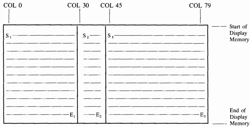
Figure 4-7. Vertical Range Tab Sequence Example Ec&a30s45s . ( S_n is the starting point and E_n is the ending point of the tab sequence in the n th region.)
