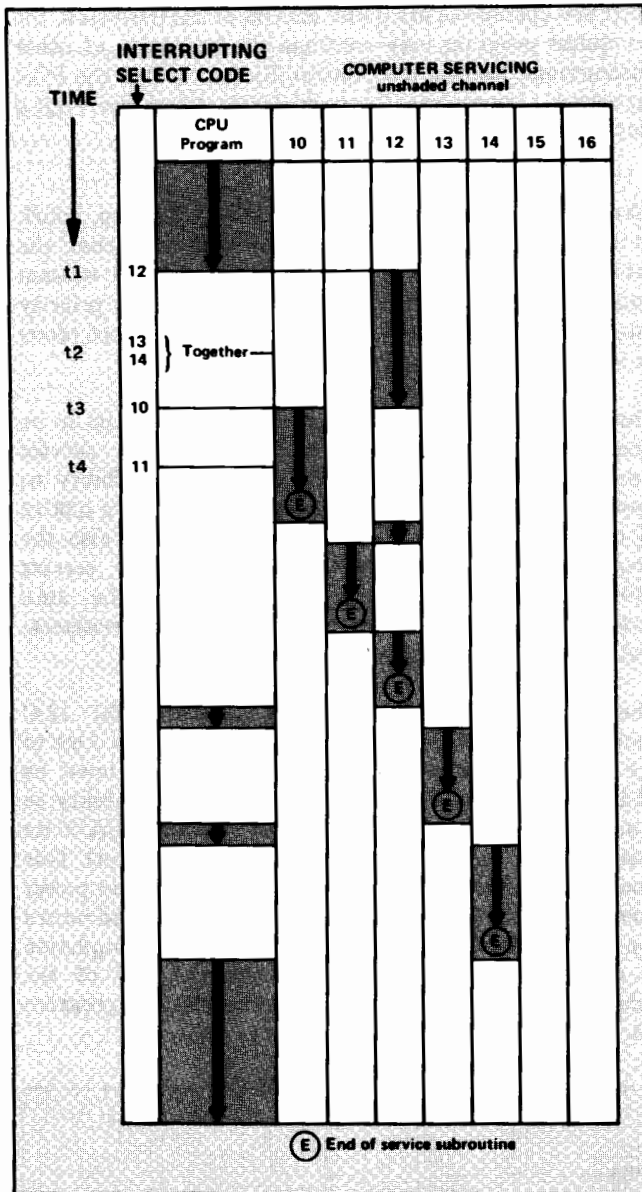
Figure 7-4. Interrupt Sequences
