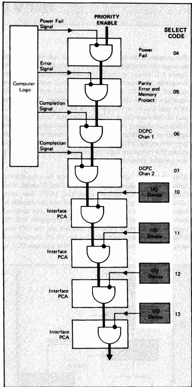
Figure 7-3. Priority Linkage
