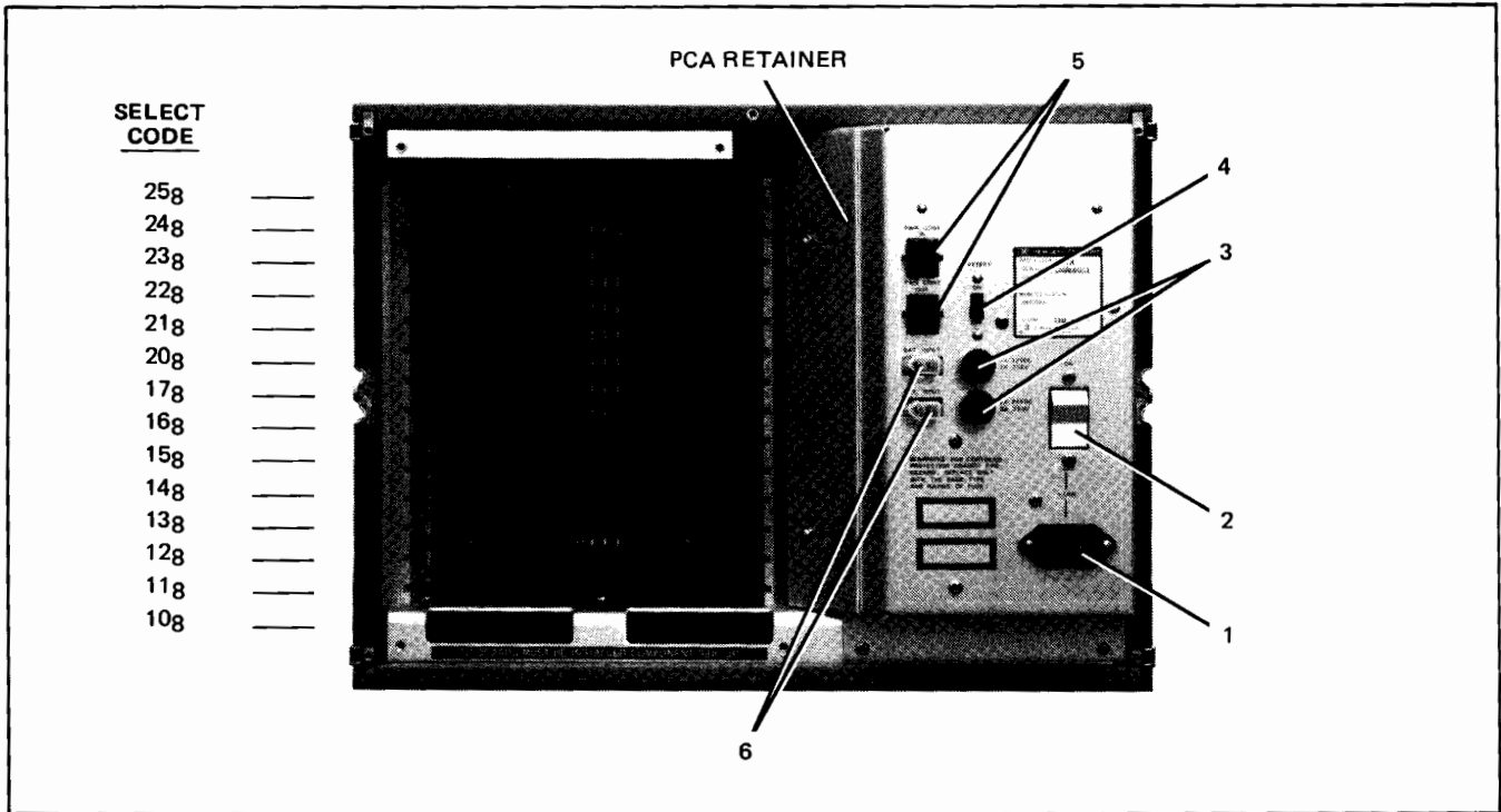
Figure 2-3. HP 2113A Rear Panel and I/O PCA Cage
