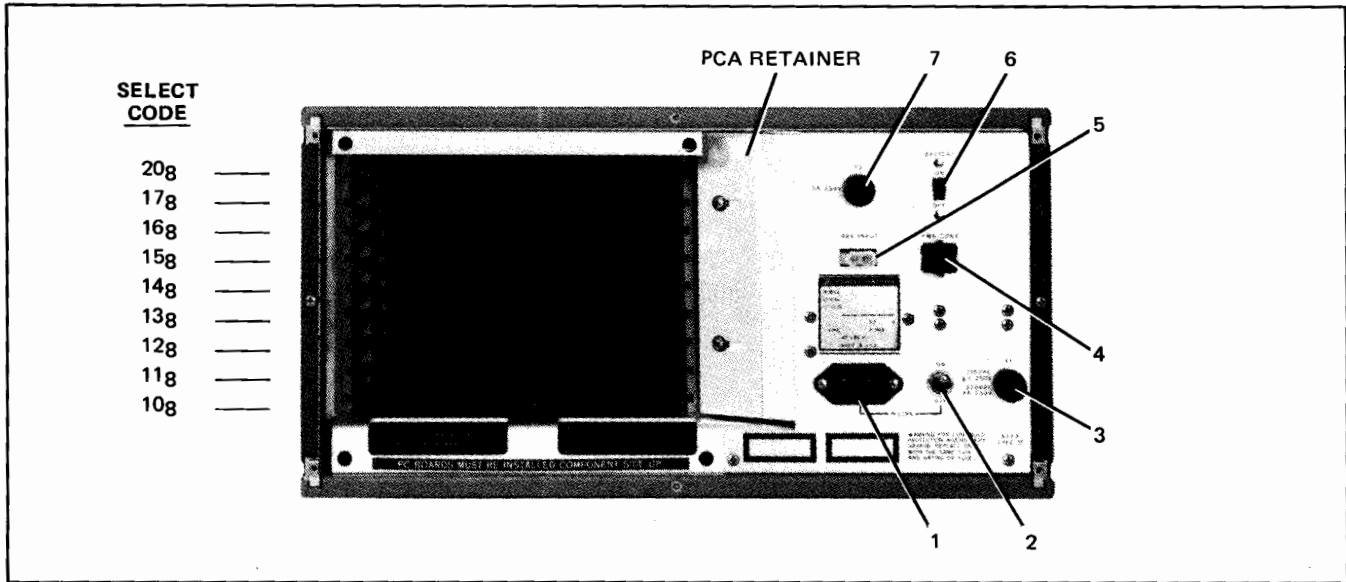
Figure 2-2. HP 2109A Rear Panel and I/O PCA Cage
