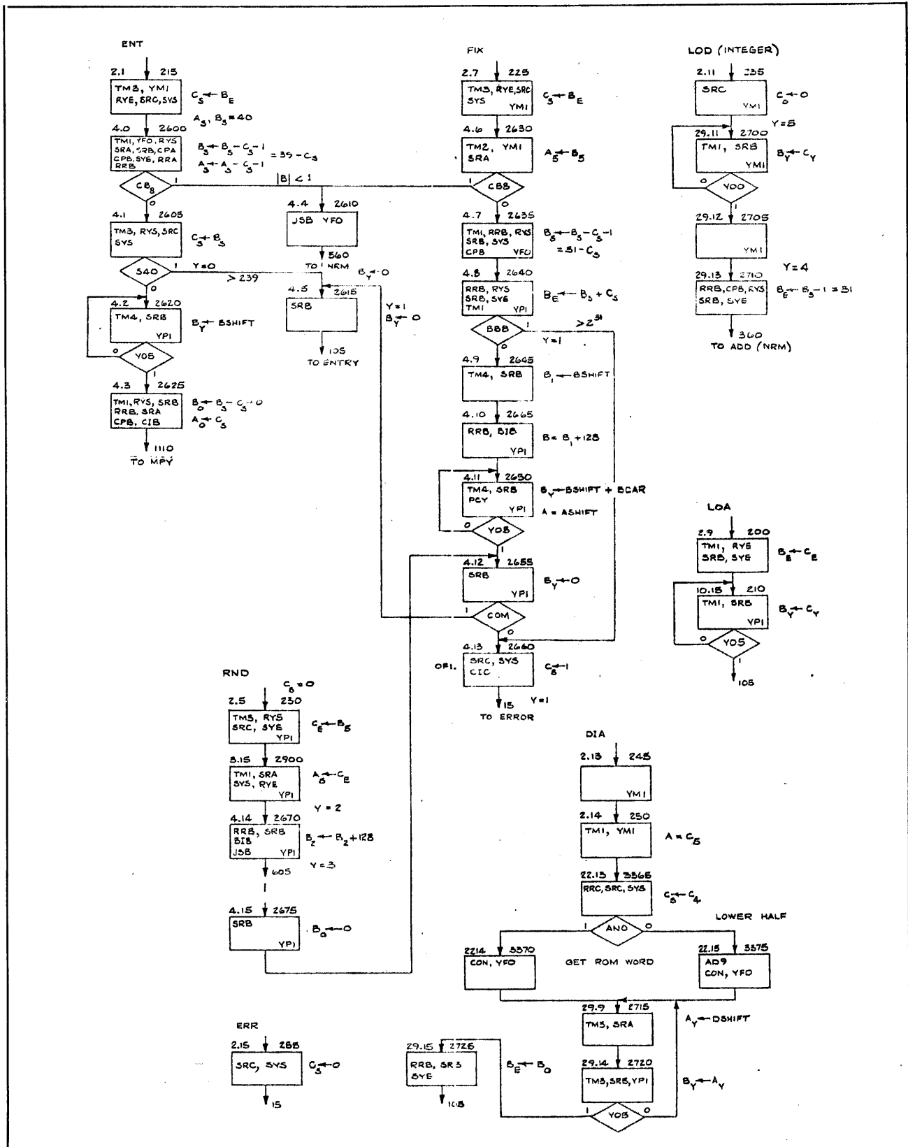
Figure 7-33. Entier/Fix/Load/Load I/Round Flowcharts
