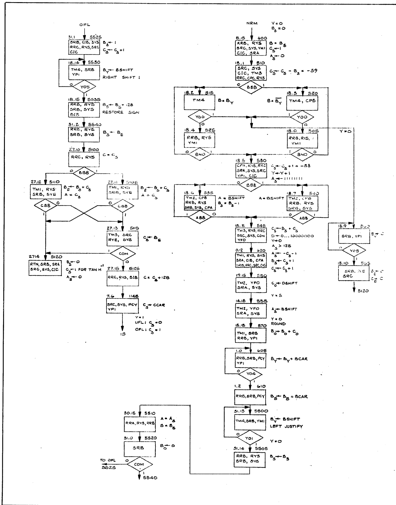
Figure 7-35. Overflow/Normalize Flowcharts
