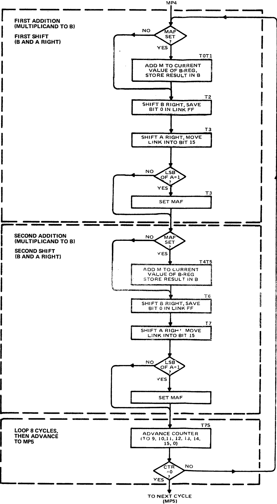
Figure 5-26. Multiply Cycle 4
