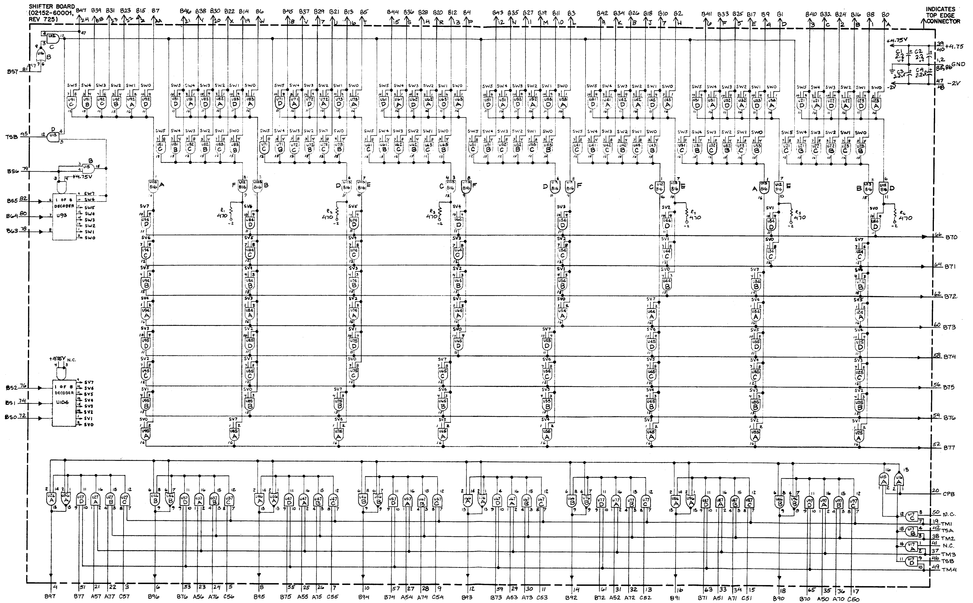
Figure 7-20. B-Shifter Card A13, Logic Diagram 7-22A
