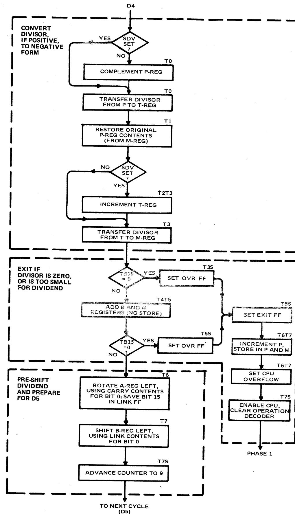
Figure 5-31. Divide Cycle 4
