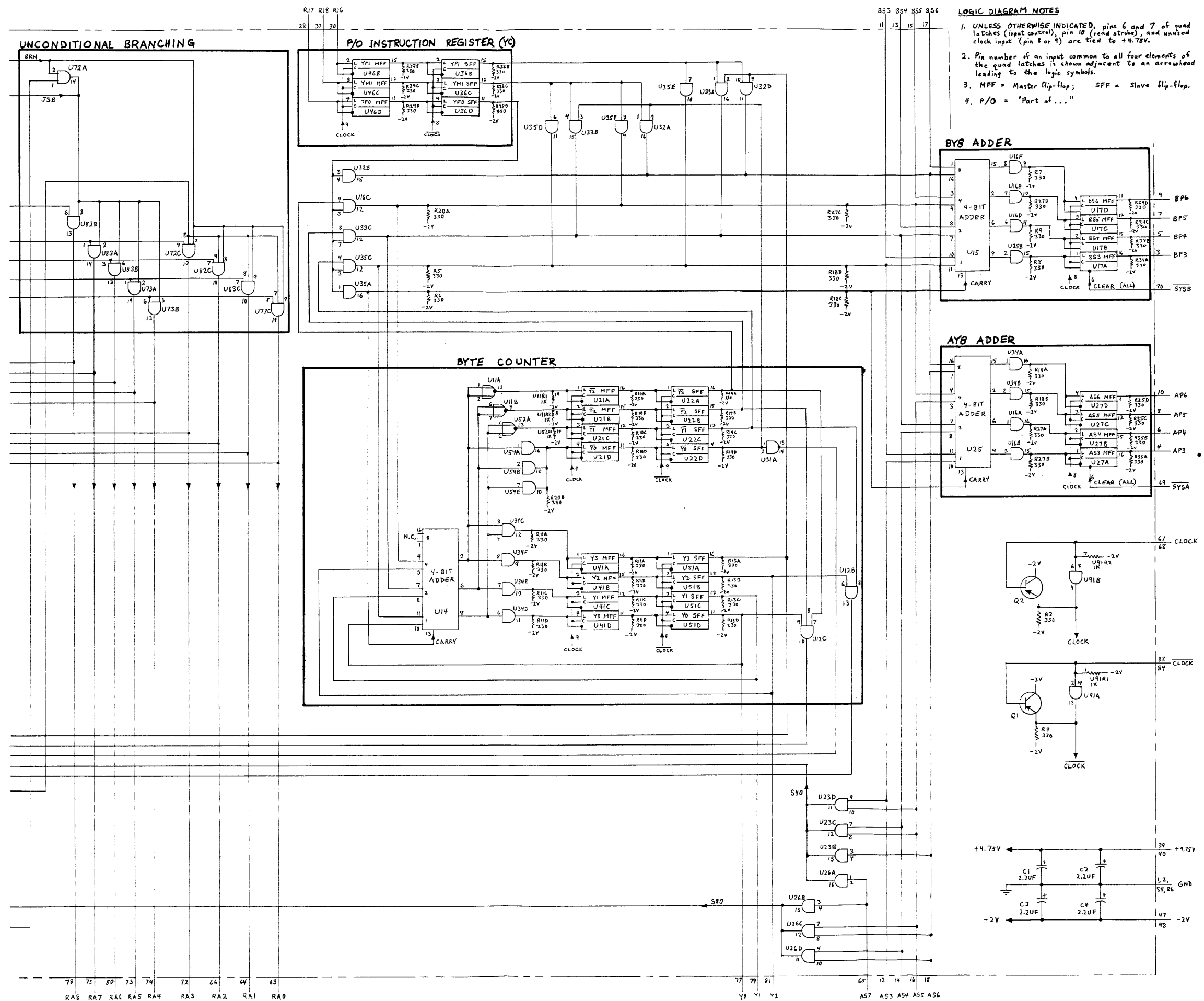
Figure 7-10. ROM Address Card A8, Logic Diagram (Cont'd)
