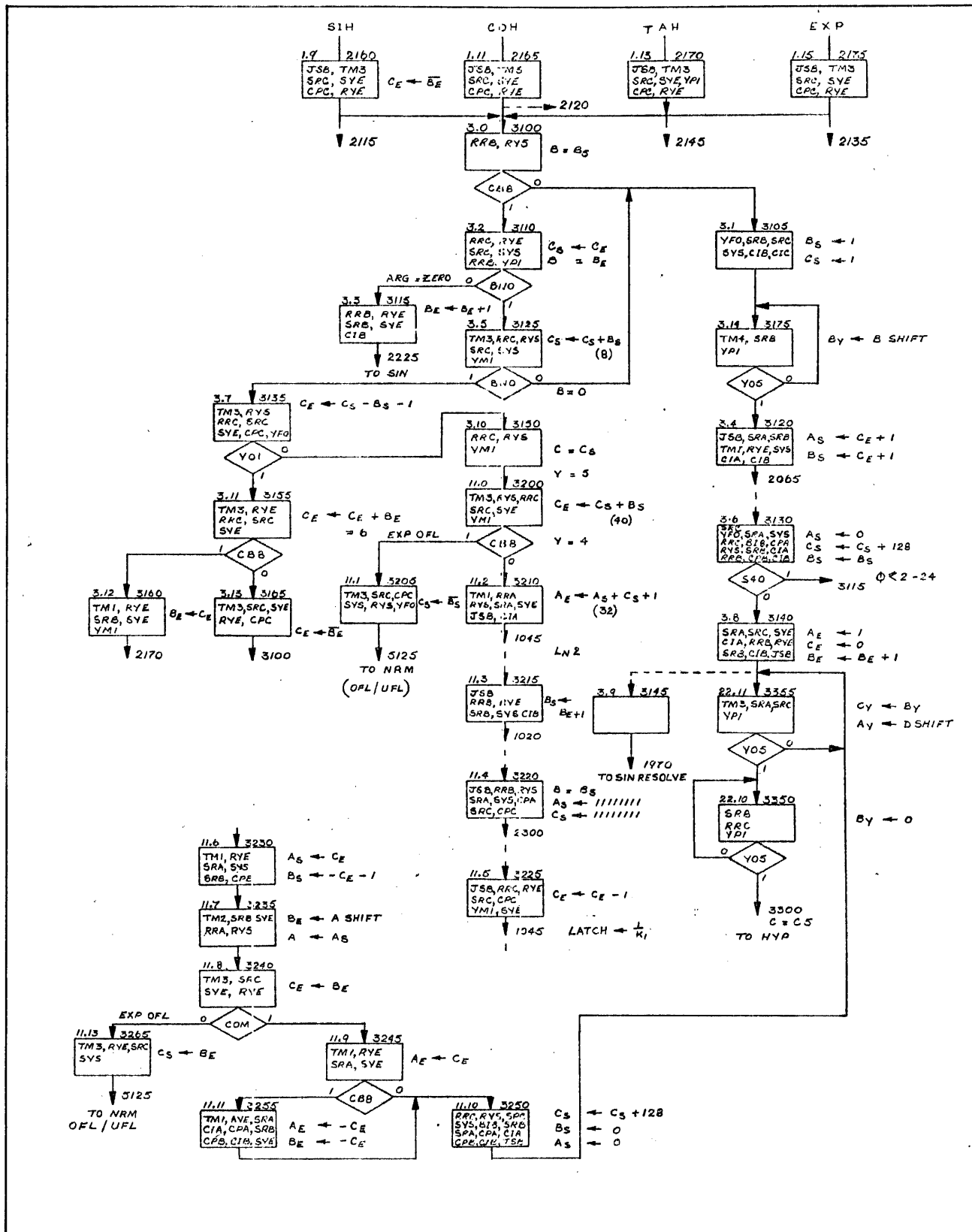
Figure 7-41. Hyperbolic Prescale Flowchart
