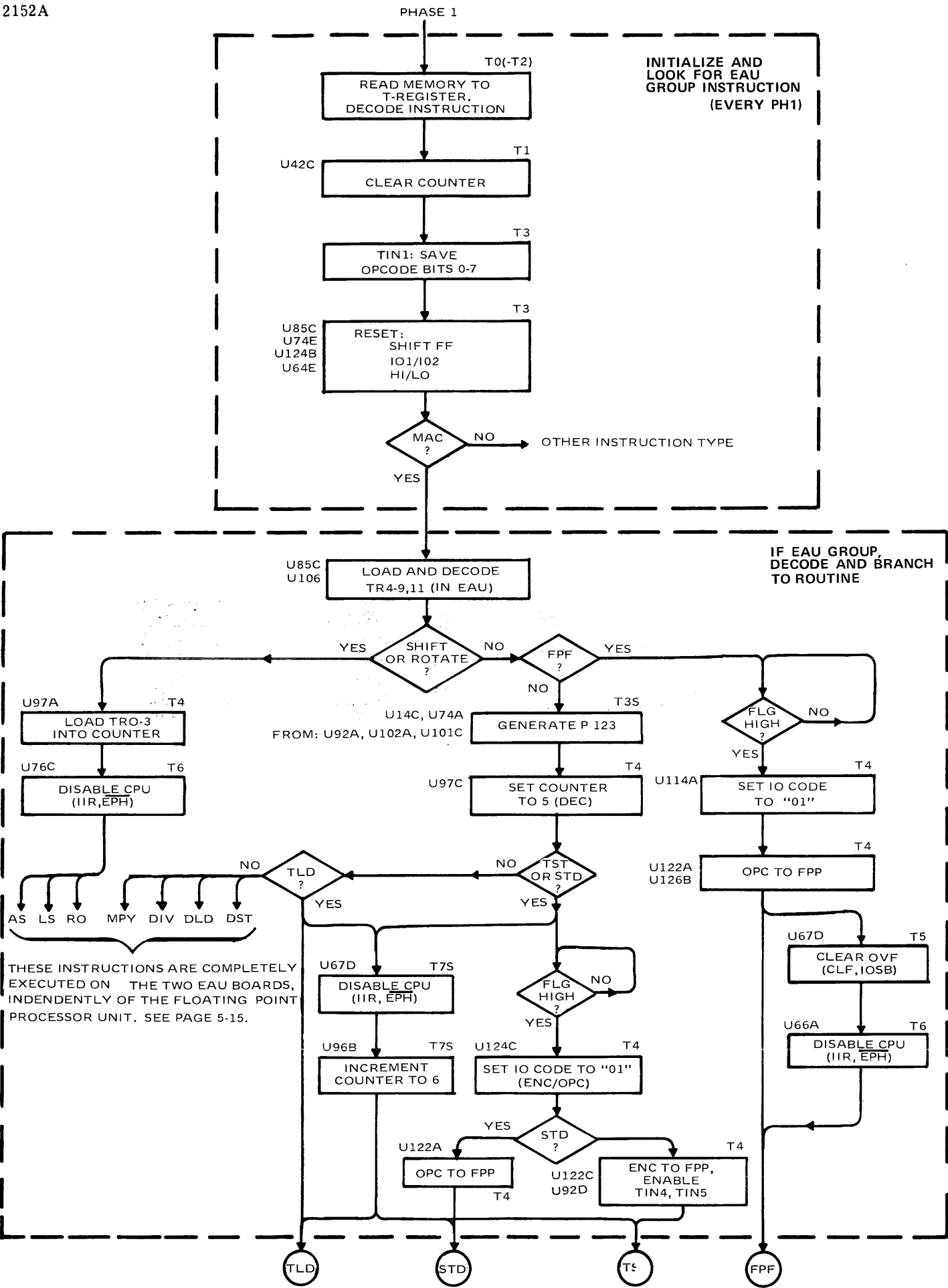
Figure 5-4. Phase 1 Flowchart
