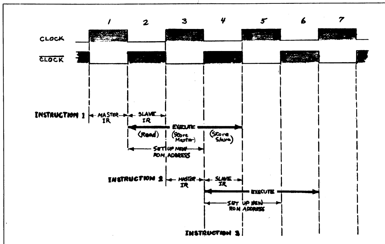
Figure 4-4. Instruction Execution Timing
