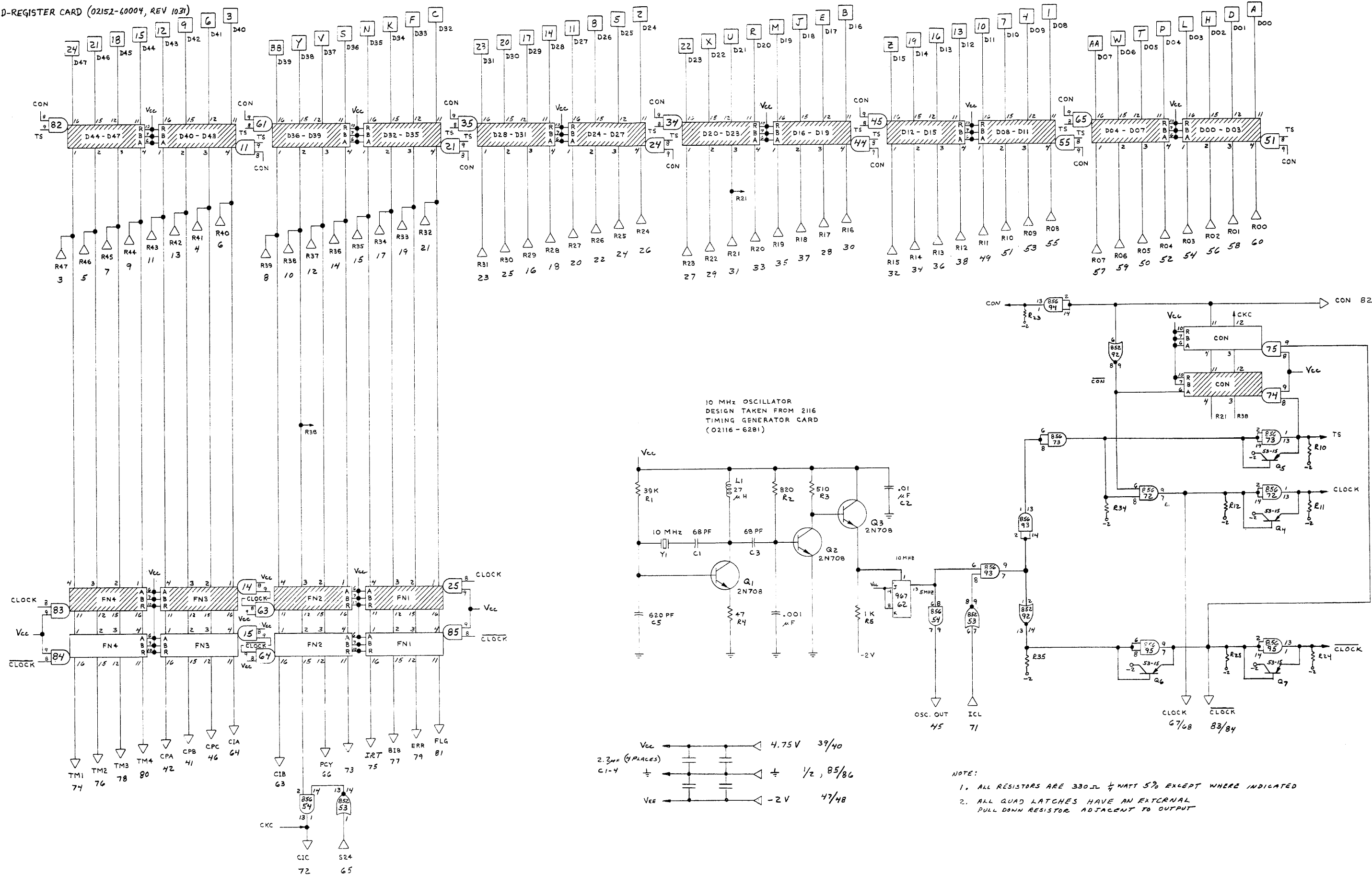
Figure 7-14. D-Register Card A10, Logic Diagram 7-16A
