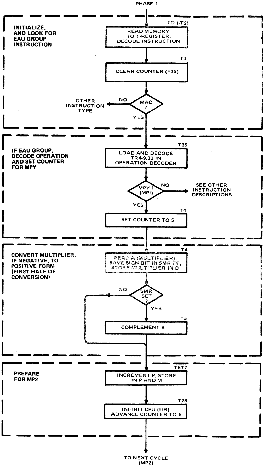
Figure 5-23. Multiply Cycle 1
