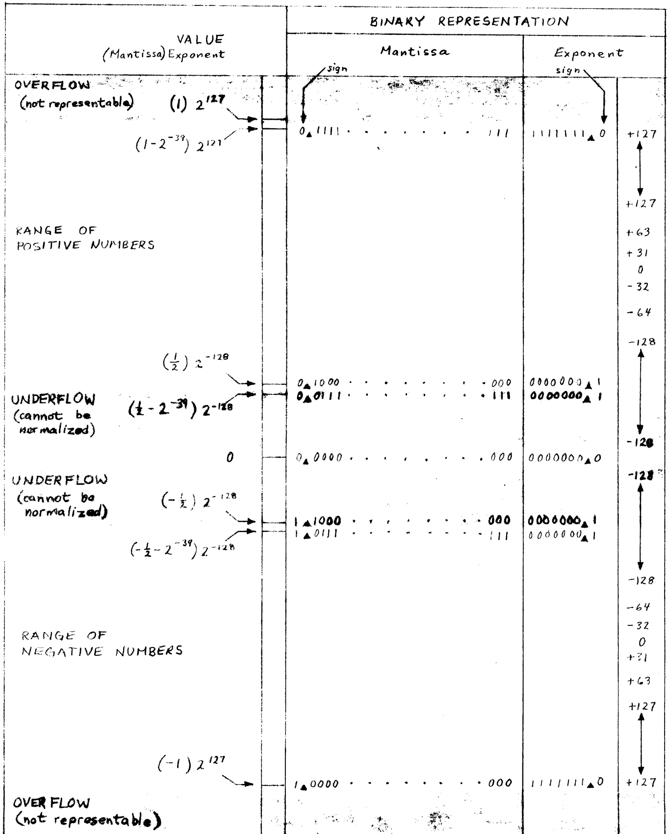
Figure 3-4. Ranges of Extended Floating Point Numbers
