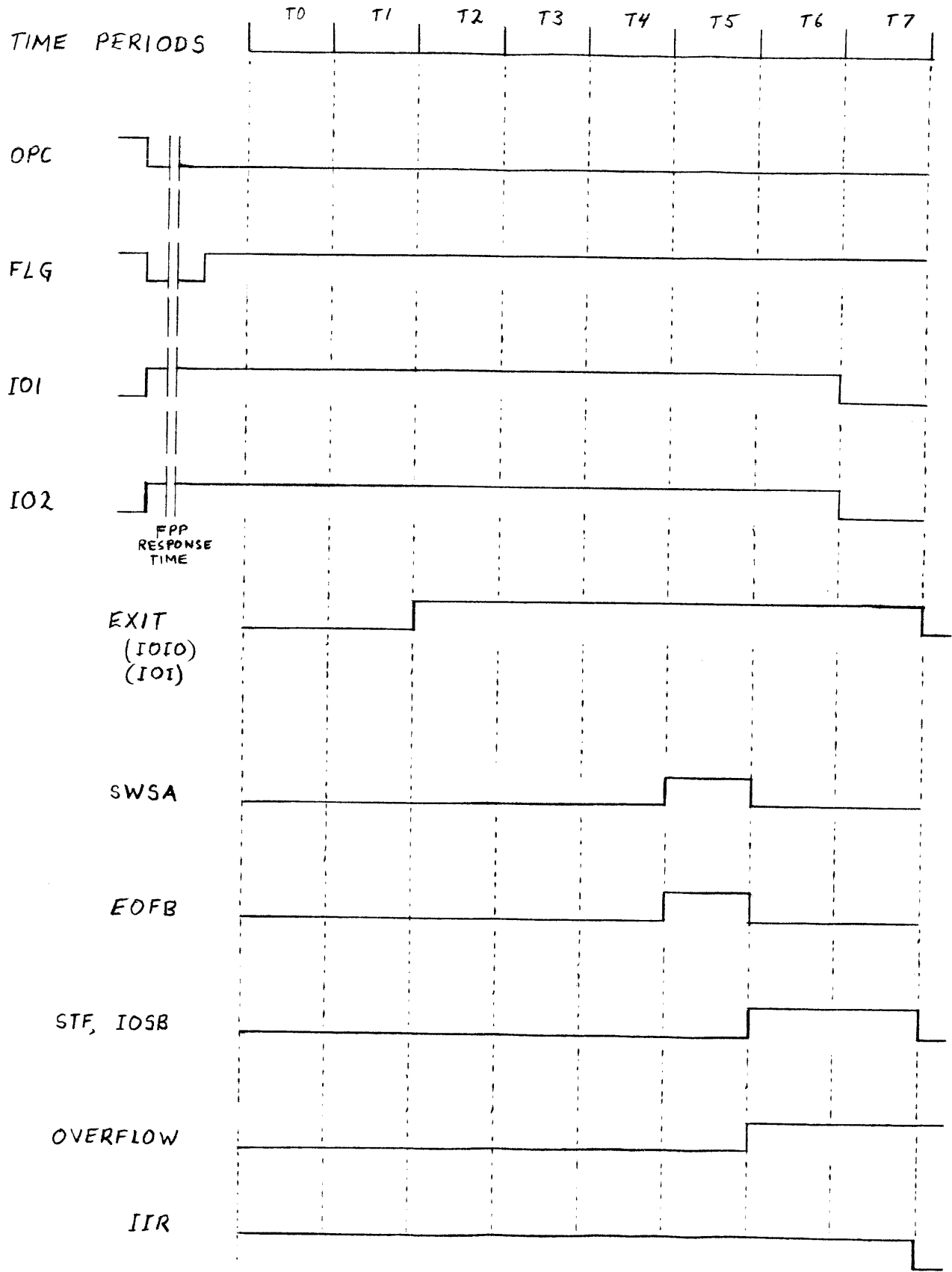
Figure 5-13. FPP Timing 5-13
