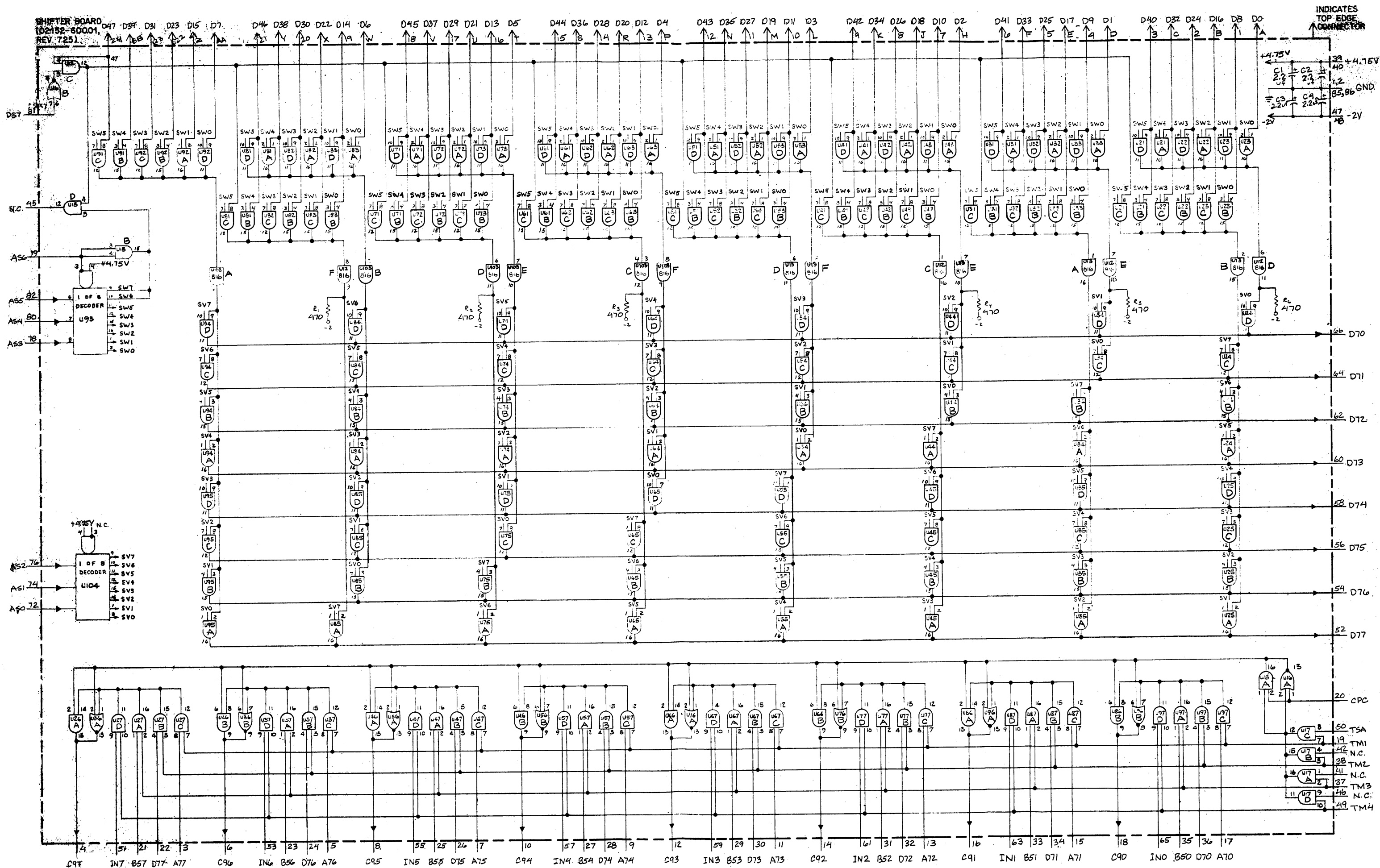
Figure 7-16. D-Shifter Card A11, Logic Diagram 7-18A
