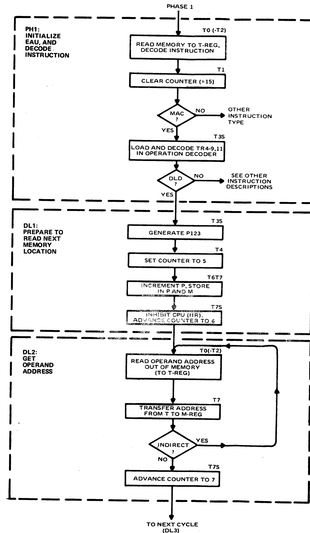
Figure 5-34. Double Load Cycles 1 and 2
