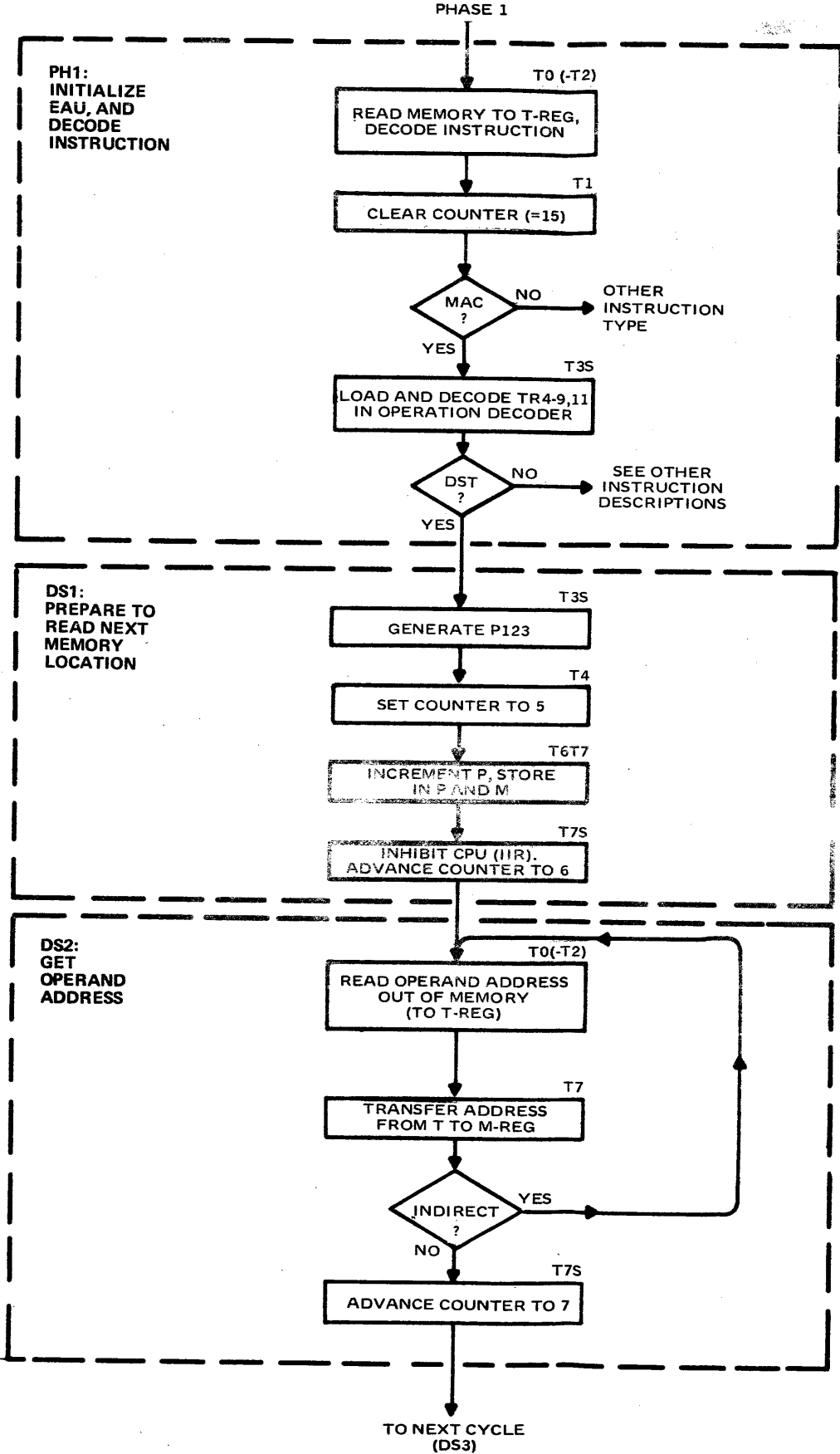
Figure 5-36. Double Store Cycles 1 and 2
