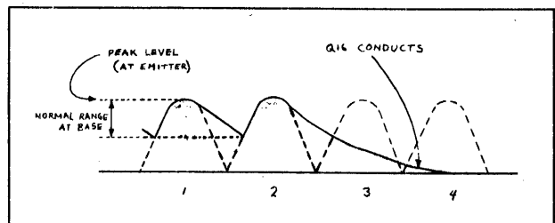
Figure 4-9. Line-Fail Sensing
