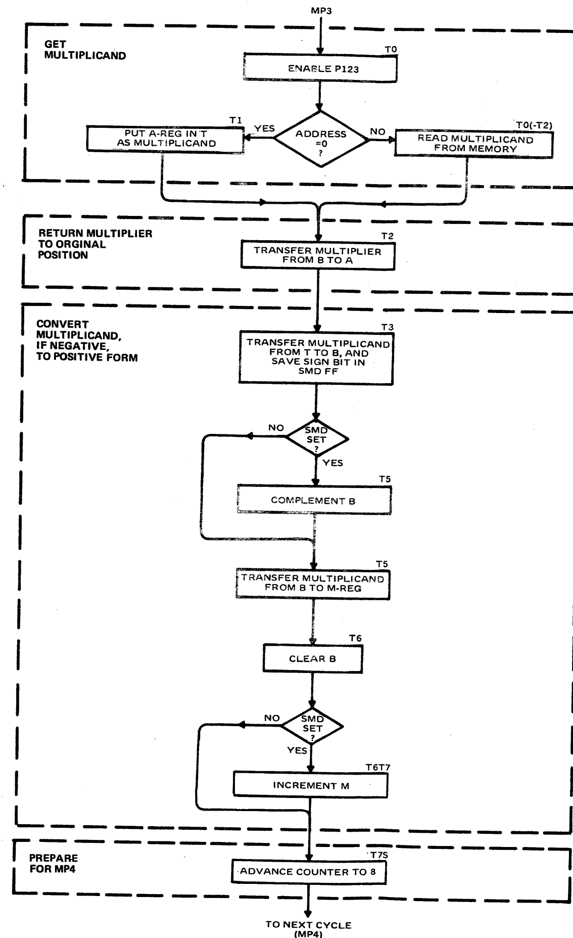
Figure 5-25. Multiply Cycle 3
