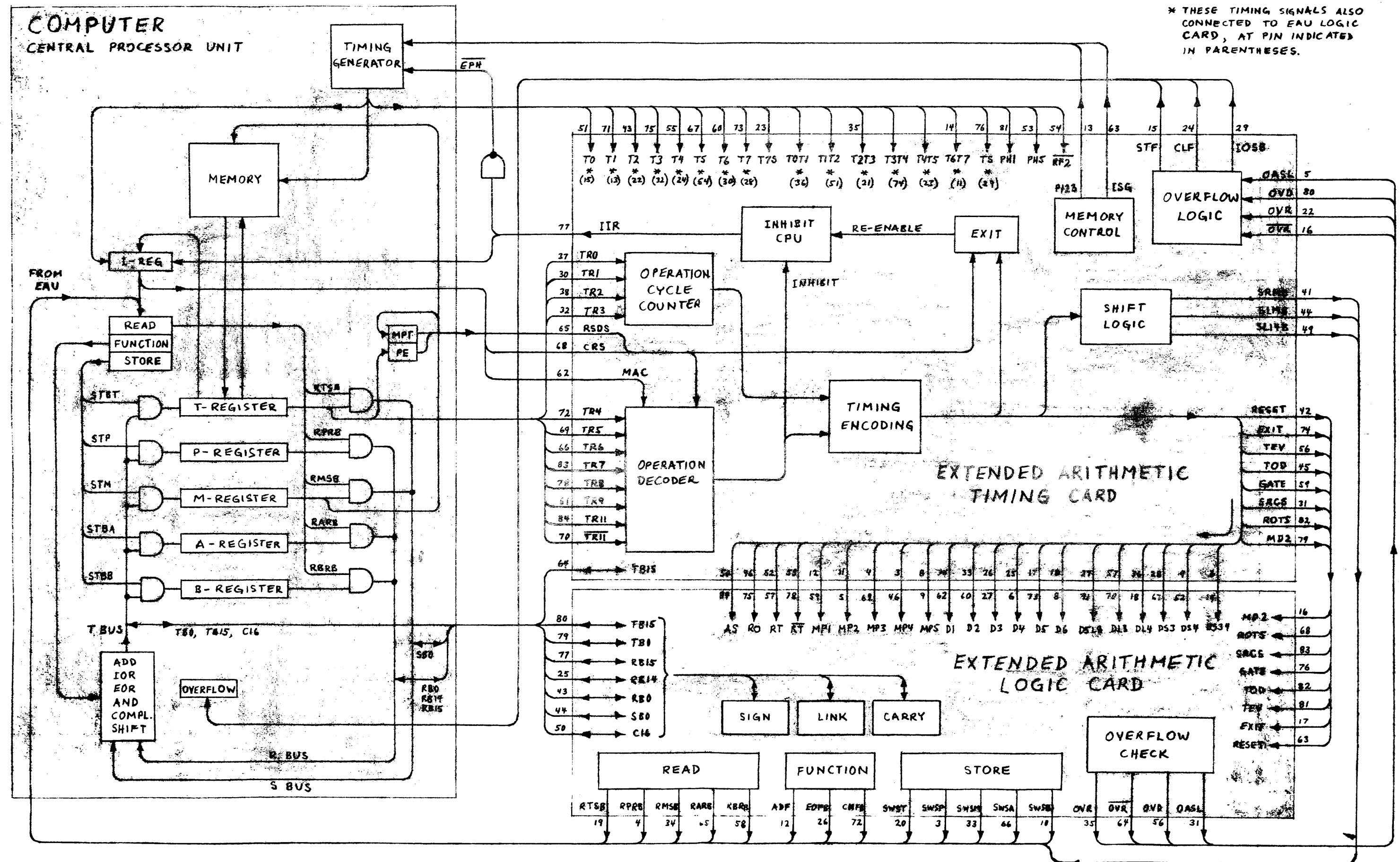
Figure 5-22. EAU Block Diagram 5-39
