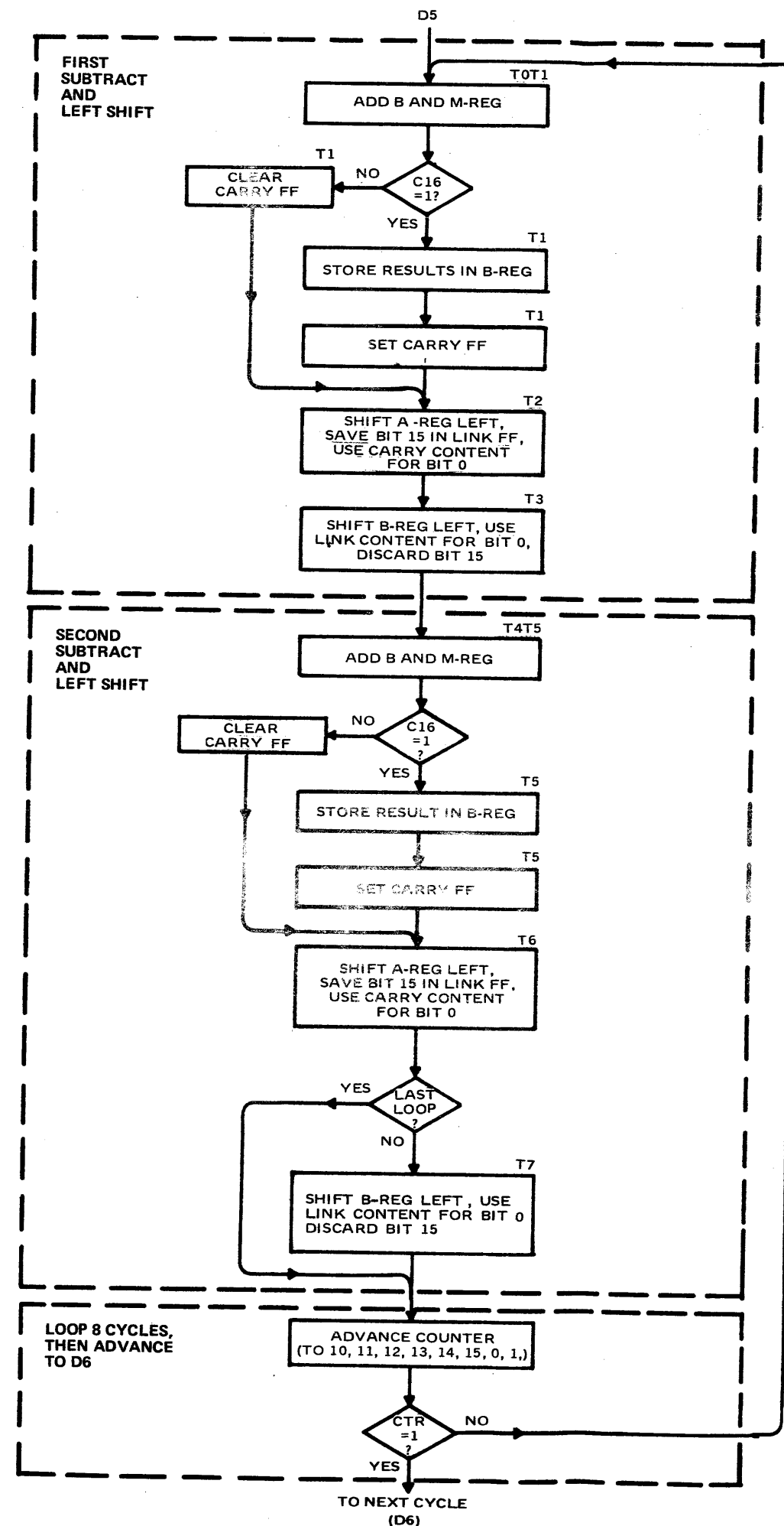
Figure 5-32. Divide Cycle 5
