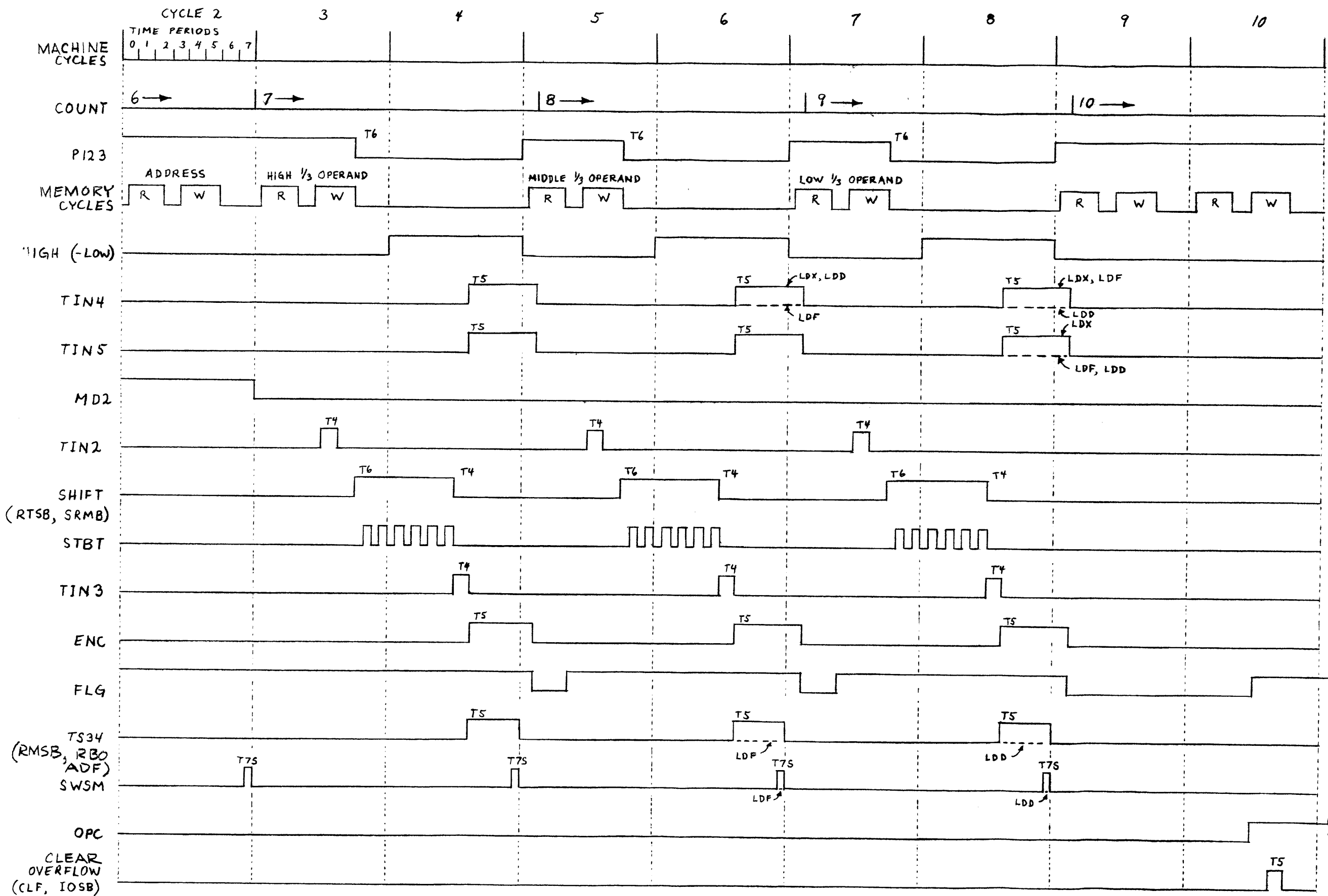
Figure 5-11. TLD Timing
