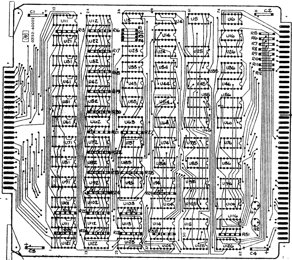
Figure 7-17. C-Adder Card A12, Parts Location View
