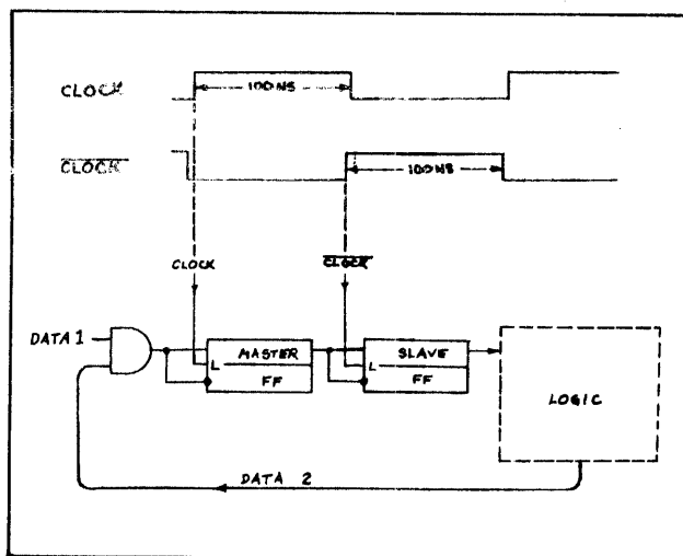
Figure 4-3. Clock Timing
