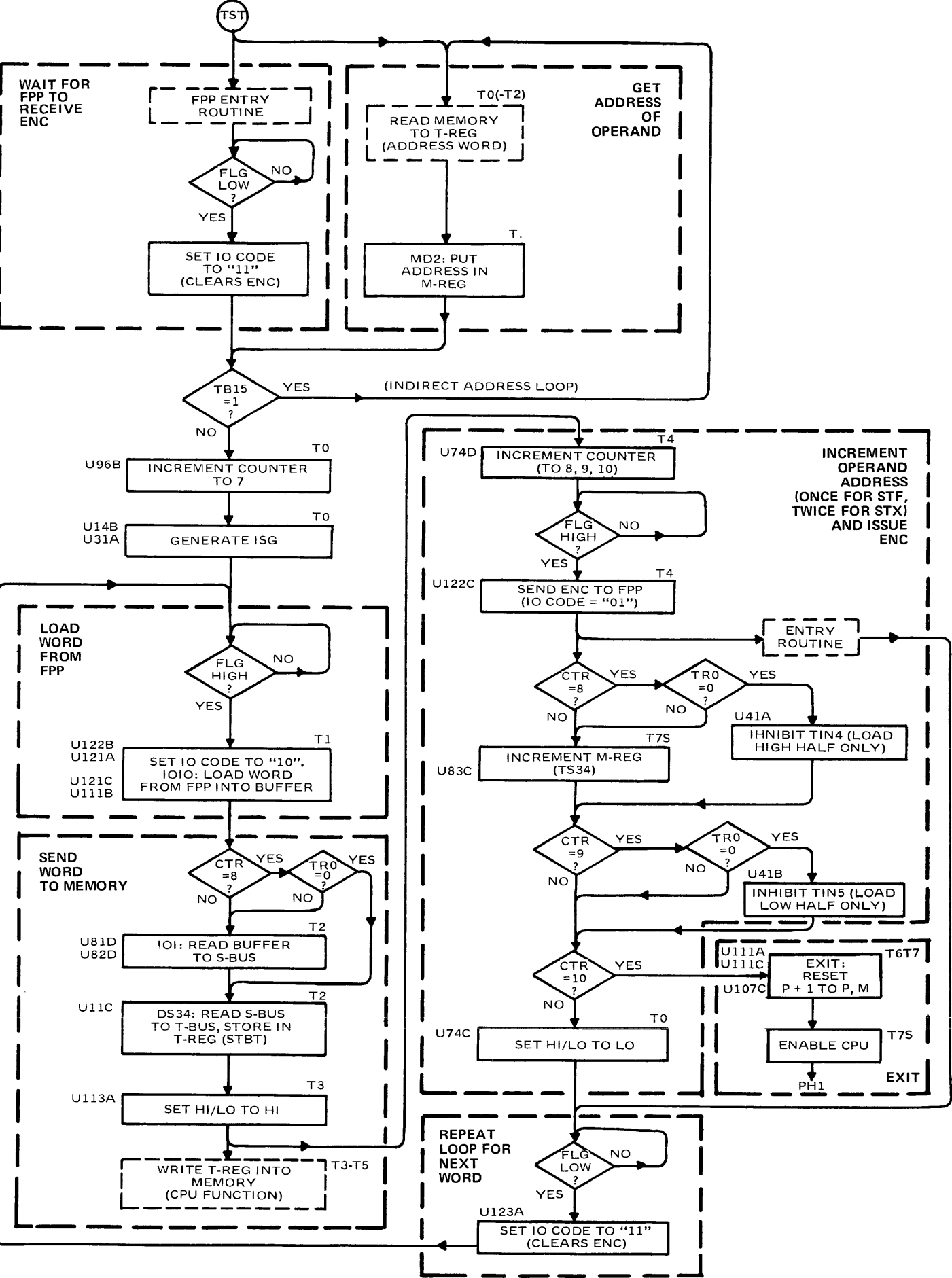
Figure 5-6. TST Flowchart
