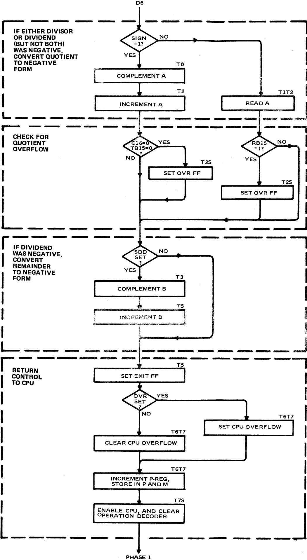
Figure 5-33. Divide Cycle 6
