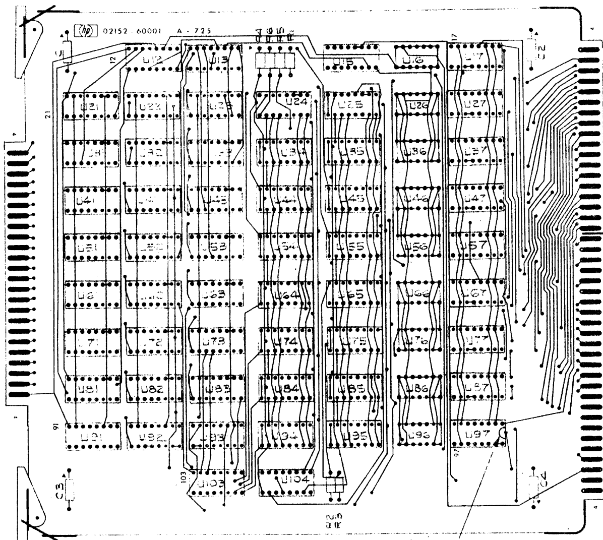
Figure 7-23. A-Shifter Card A15, Parts Location View
