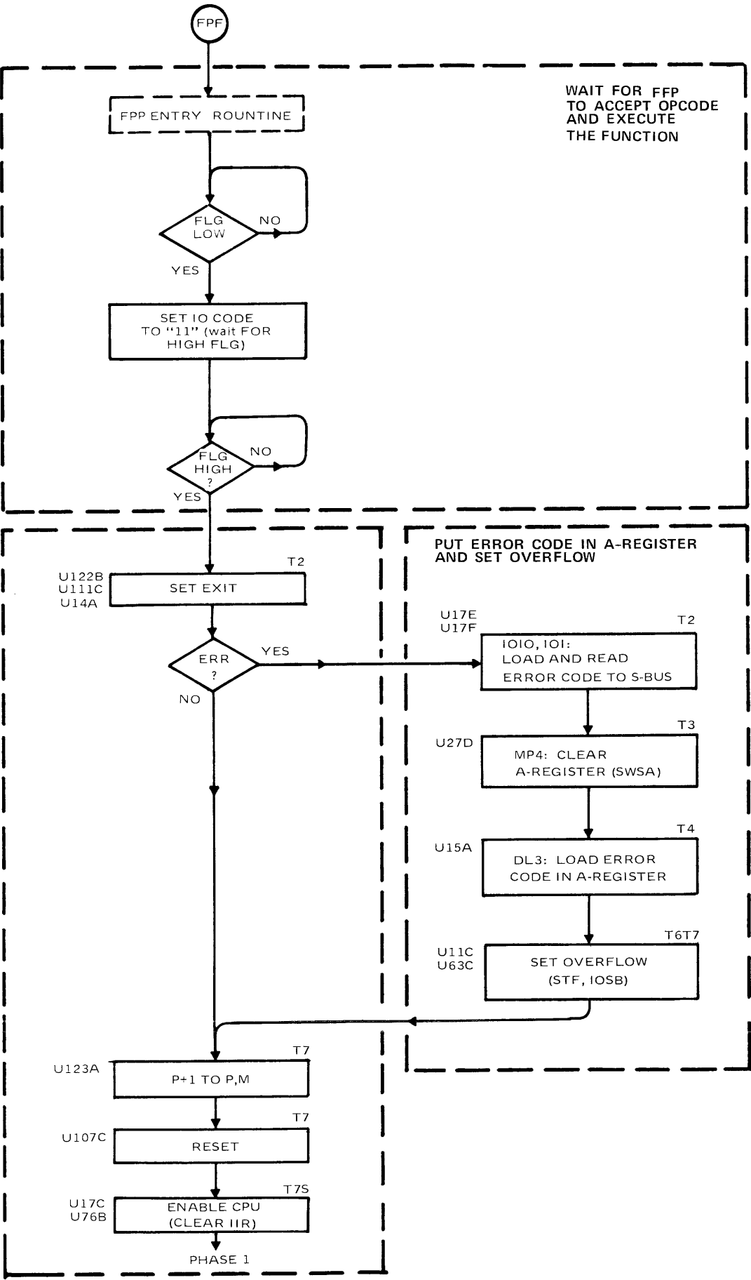
Figure 5-12. FPF Flowchart
