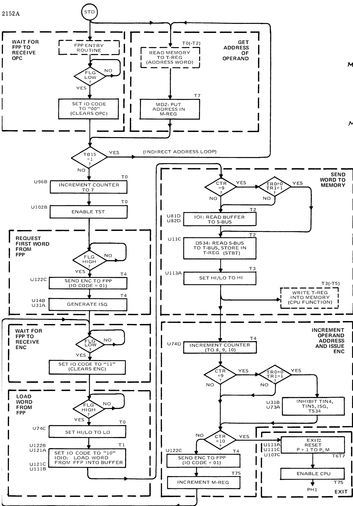
Figure 5-8. STD Flowchart
