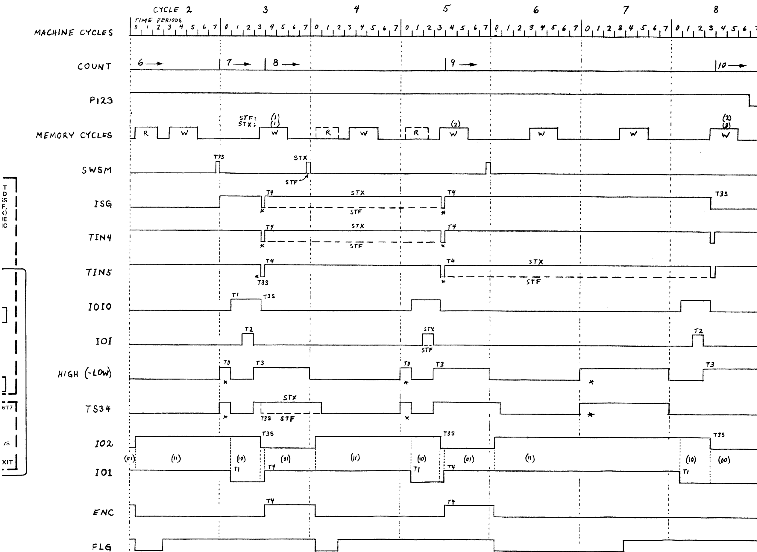
Figure 5-7. TST Timing 5-7
