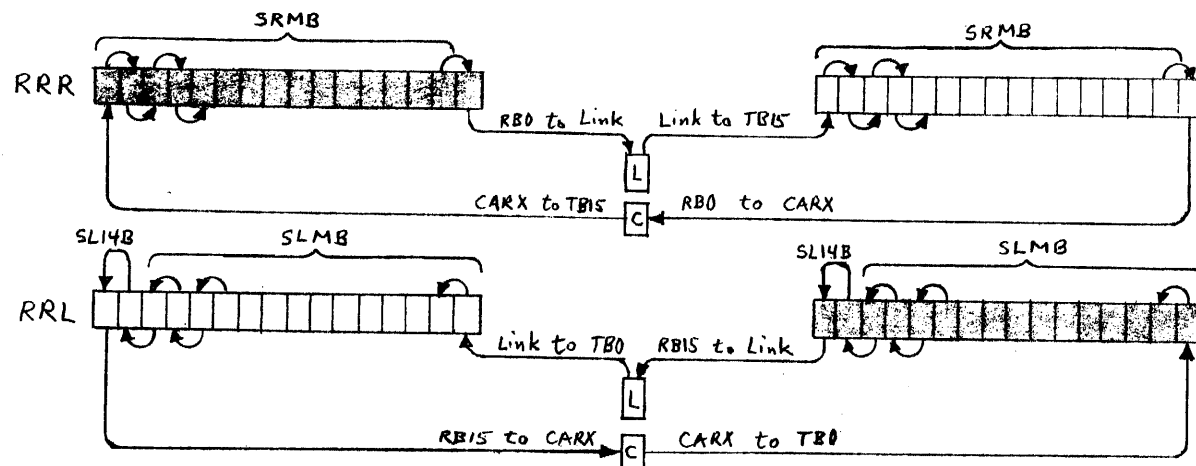
Figure 5-21. Shift Operations
