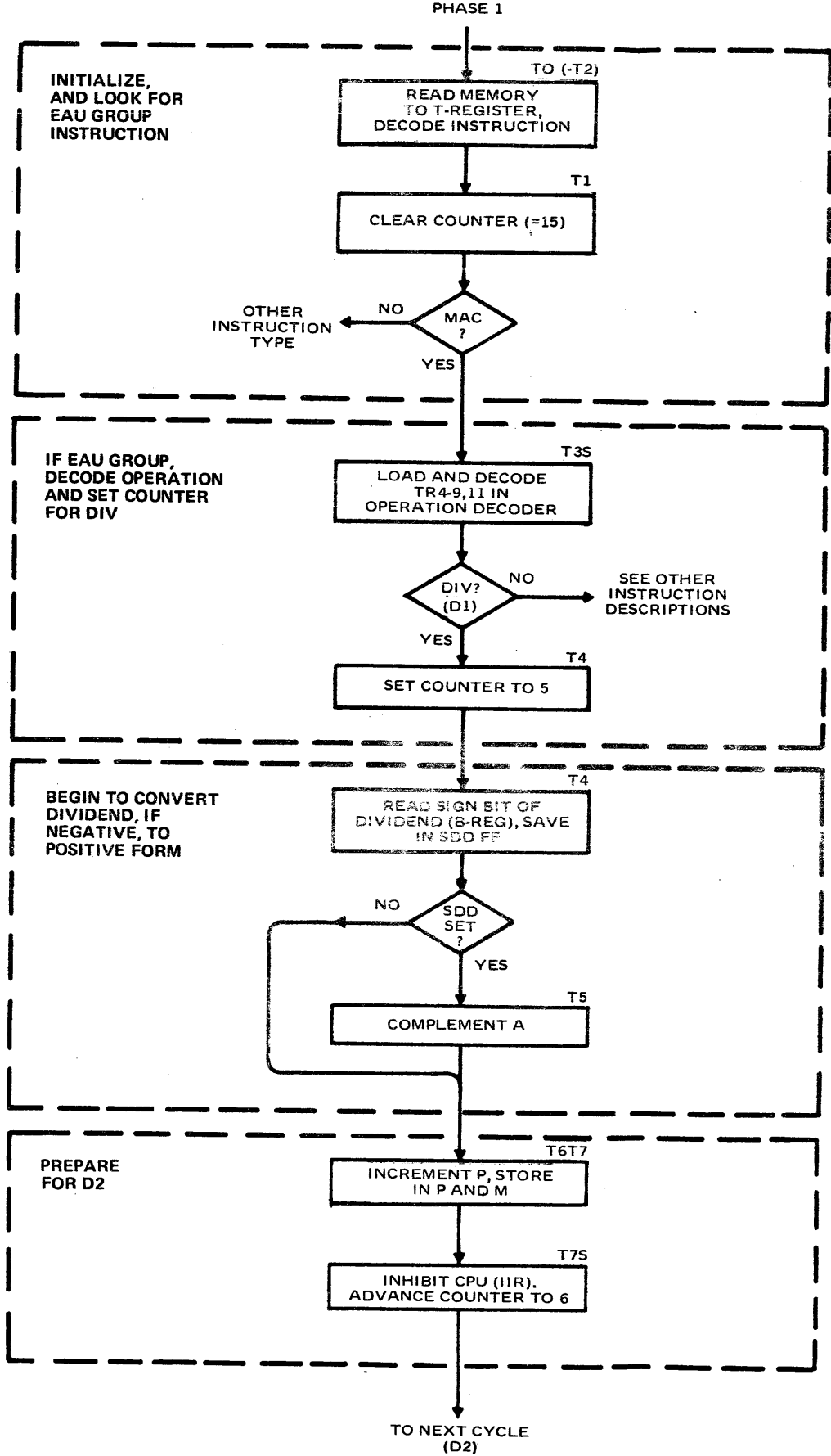
Figure 5-28. Divide Cycle 1
