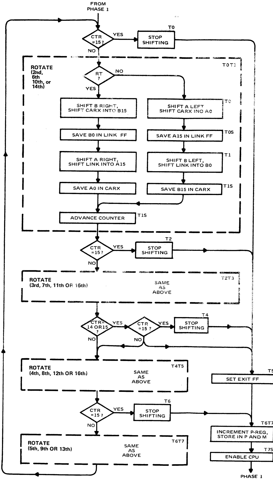
Figure 5-43. Rotate Loops
