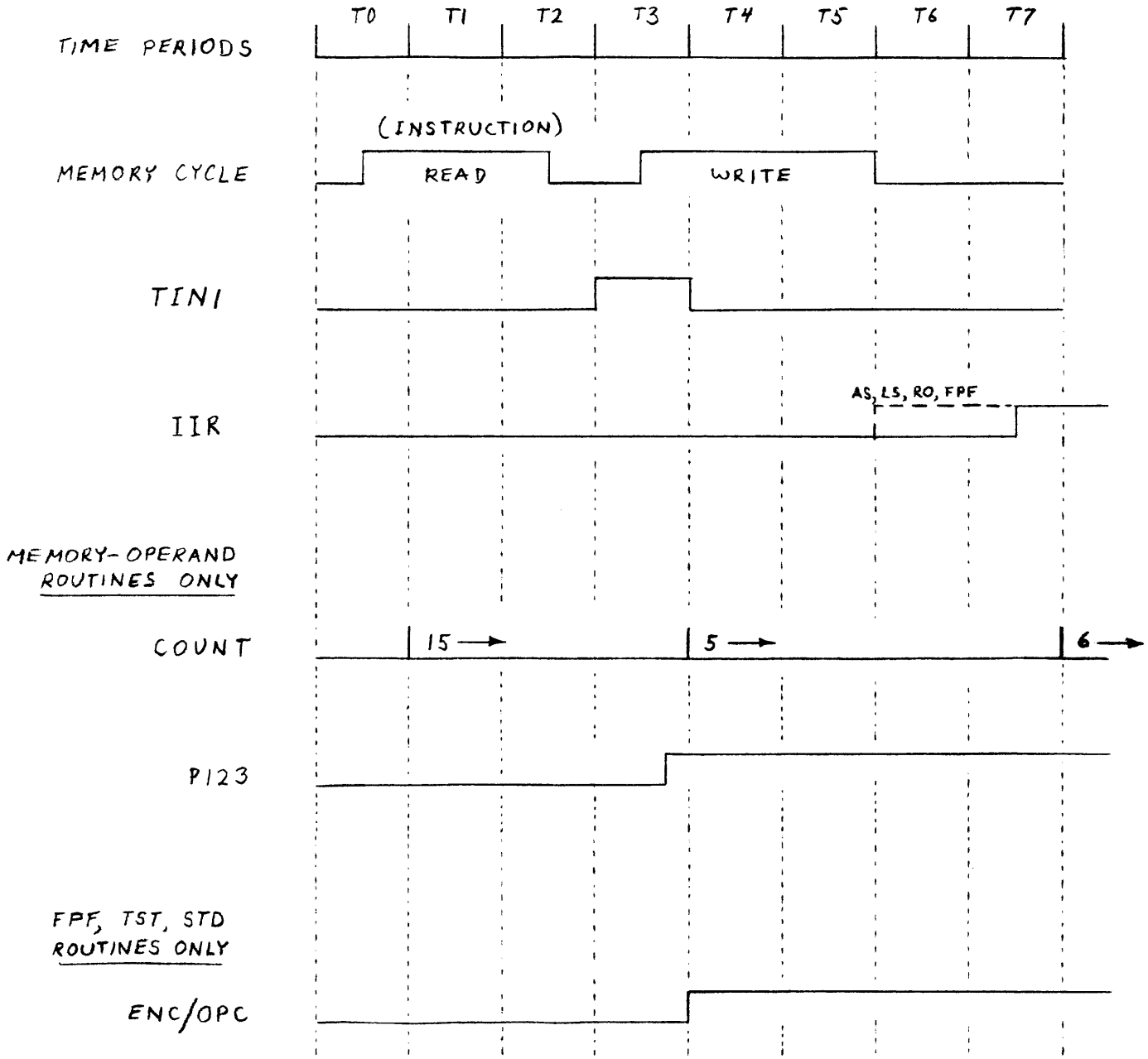
Figure 5-5. Phase 1 Timing
