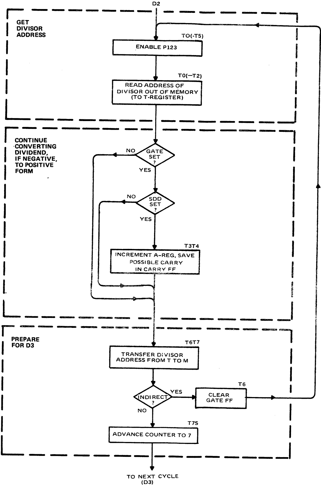
Figure 5-29. Divide Cycle 2
