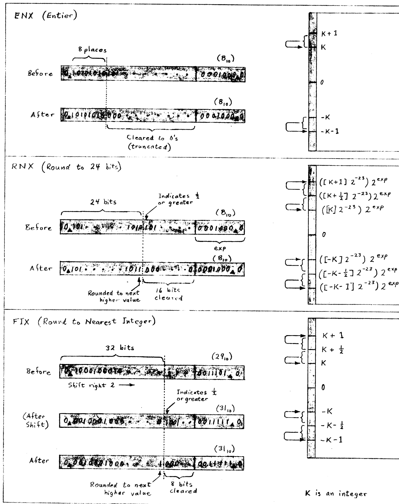
Figure 3-5. Examples of ENX, RNX, and FIX
