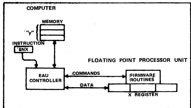
Figure 1-2. Floating Point Processor as a Calculator
