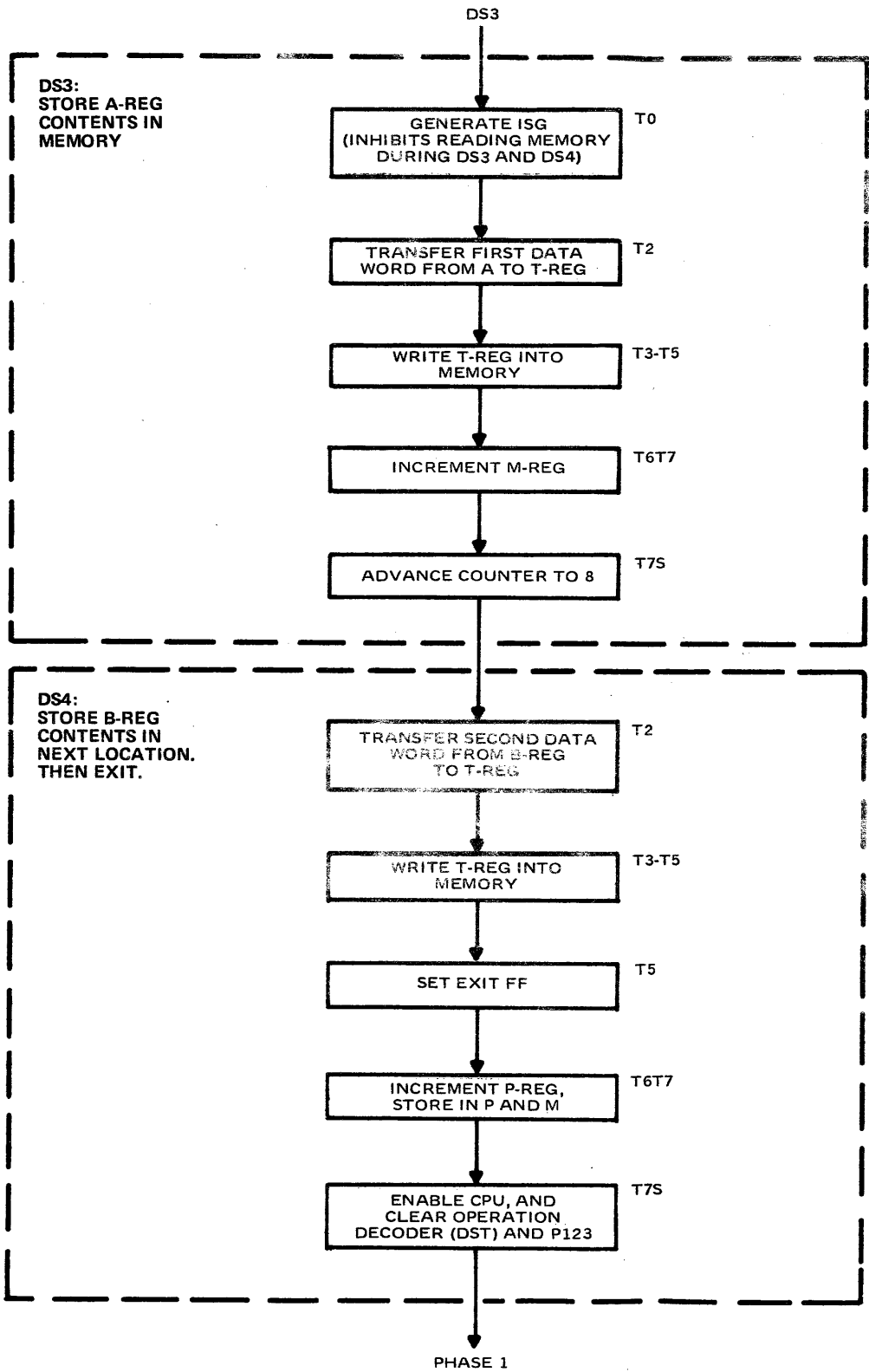
Figure 5-37. Double Store Cycles 3 and 4
