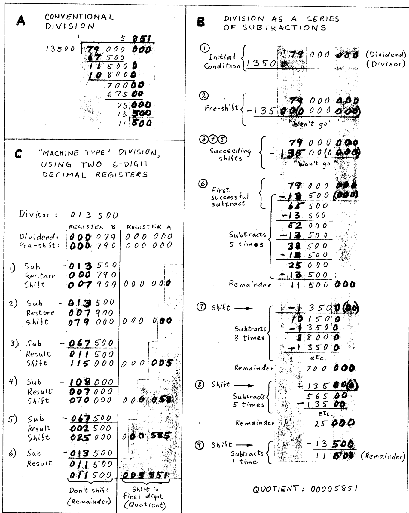
Figure 5-18. Decimal Division
