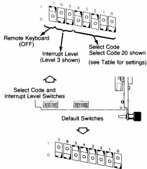
Figure 5-12. HP 98628A Datacomm Interface Switches
