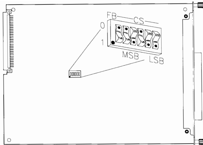
Figure 5-25. HP 98725A LGB Interface Switches
