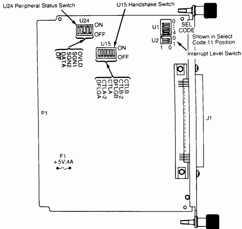
Figure 5-6. HP 98623A BCD Interface switches.
