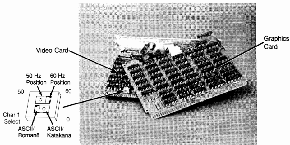
Figure 5-3. Display Compatibility Interface switches.
