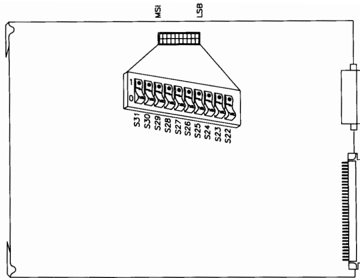
Figure 3-3. Built-in RAM switch settings
