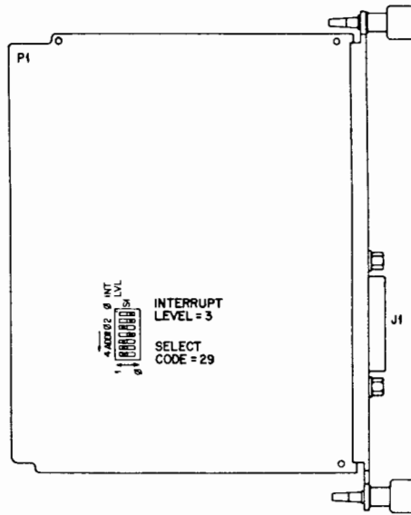
Figure 5-13. Multiprogrammer Interface Switches
