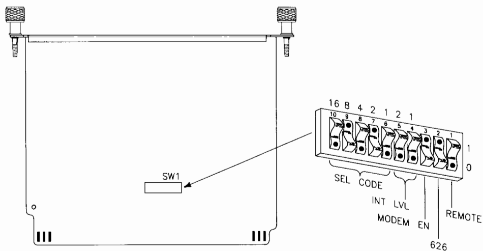
Figure 5-17. HP 98644A RS-232C Serial Interface switches.
