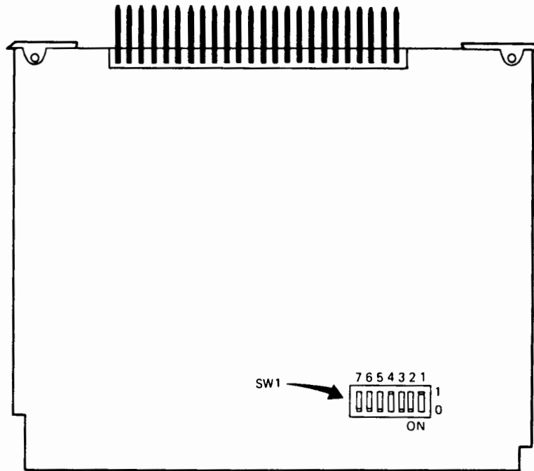
Figure 5-14. Analog Input Card Switches
