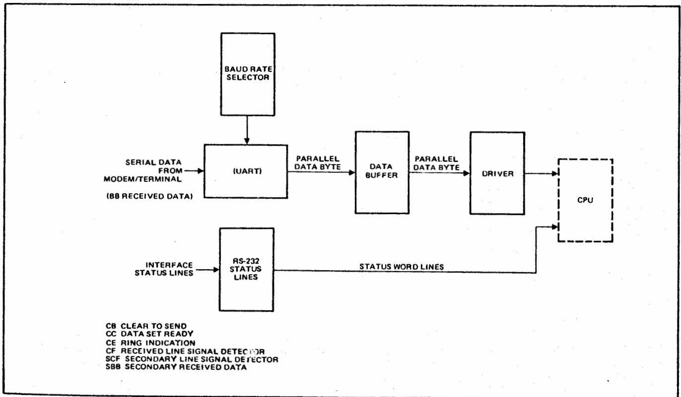
Figure 2-3. Receive Mode Data Transfer
