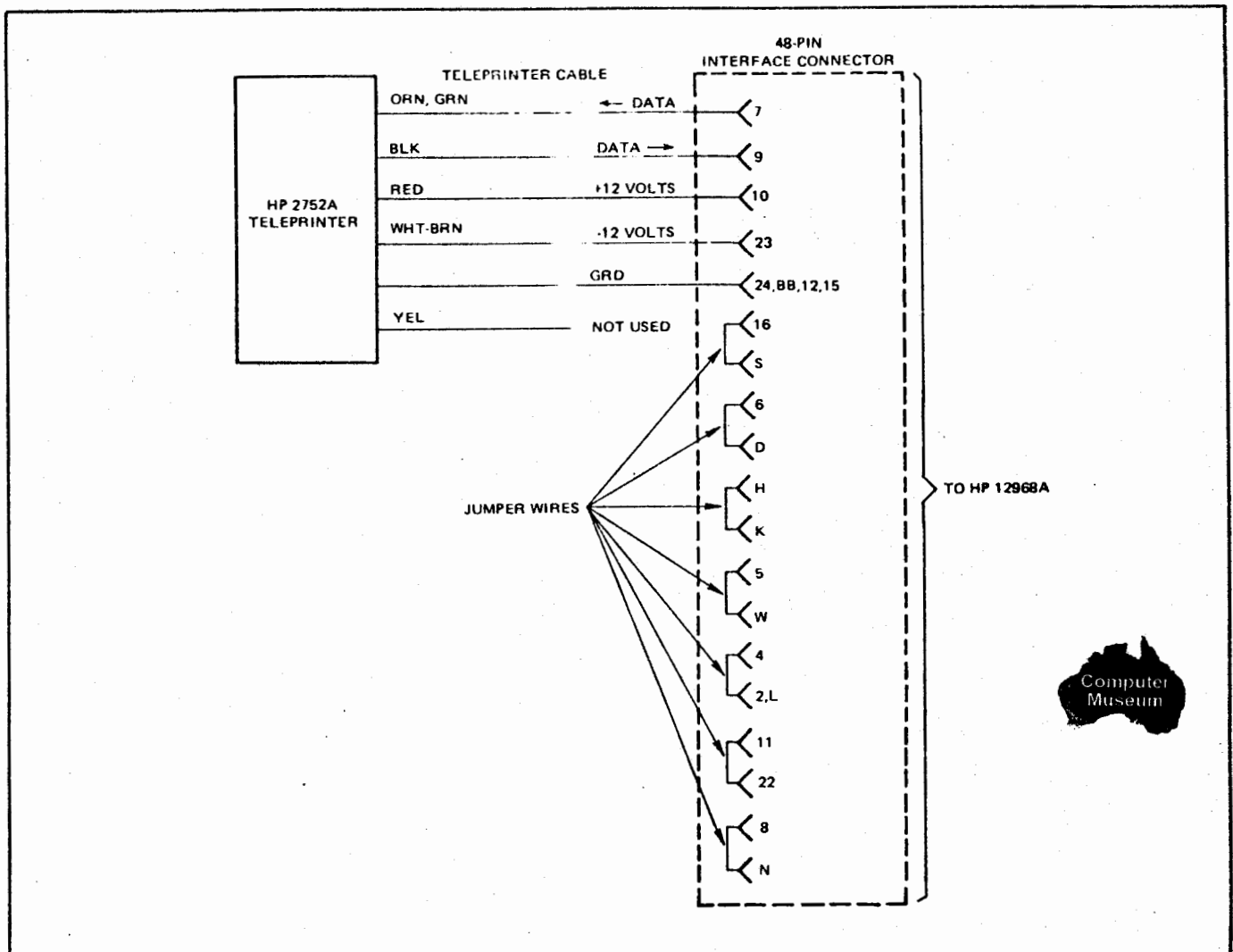
Figure 4-2. Interface Cable Connections for HP 2752A Teleprinter
