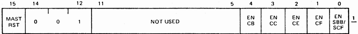
Enable Device Status Interrupt Word (Word 1)
