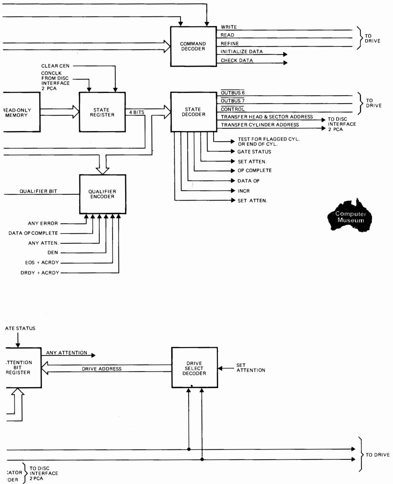
Figure 4-3. Disc Interface 1 PCA Block Diagram
