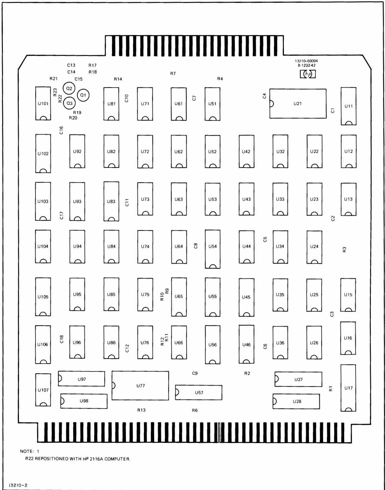
Figure 5-1. Disc Interface 1 PCA Parts Location Diagram
