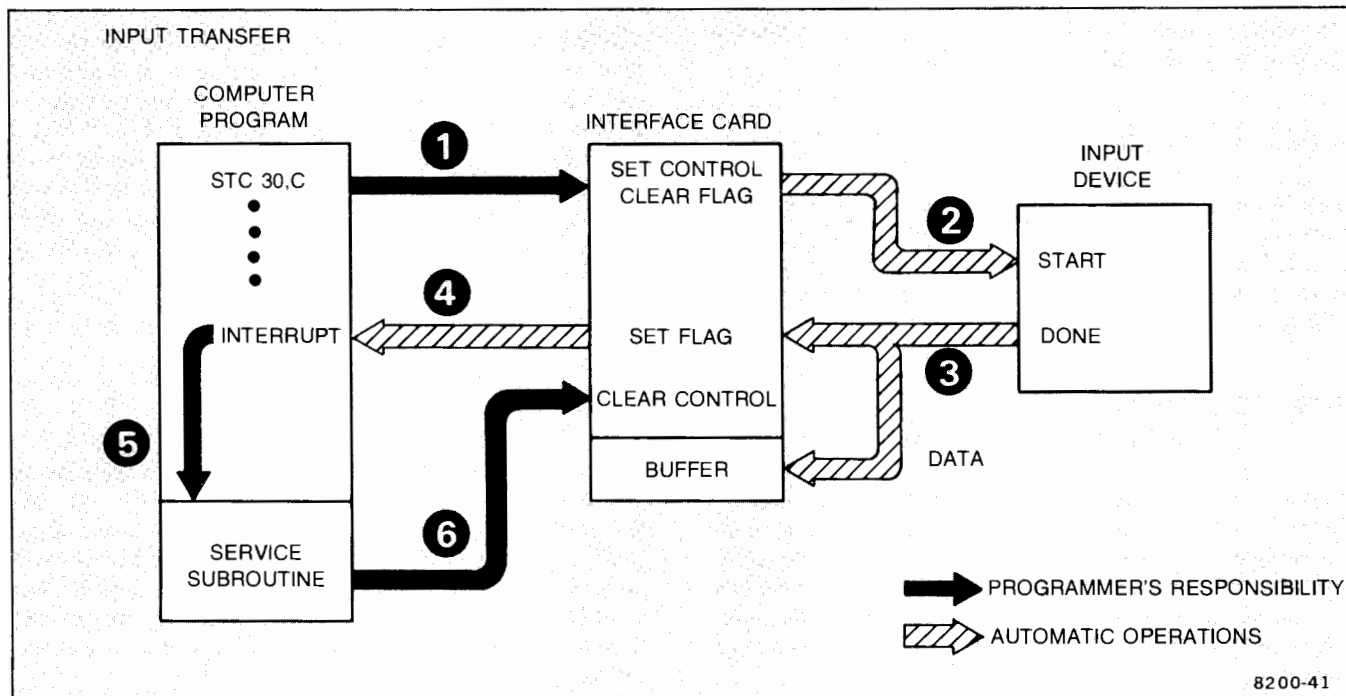
Figure 7-7. Input Data Transfer (Interrupt Method)
