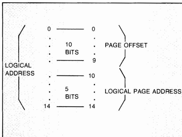
Figure 4-1. Basic Logical Memory Addressing Scheme
