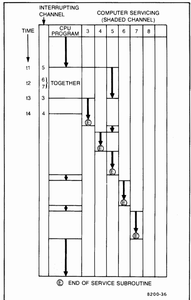
Figure 7-4. Interrupt Sequences
