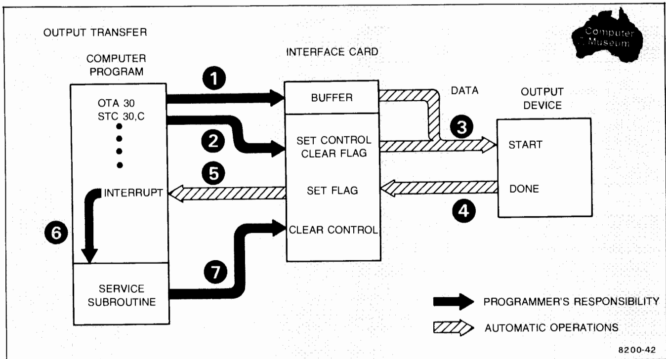
Figure 7-8. Output Data Transfer (Interrupt Method)
