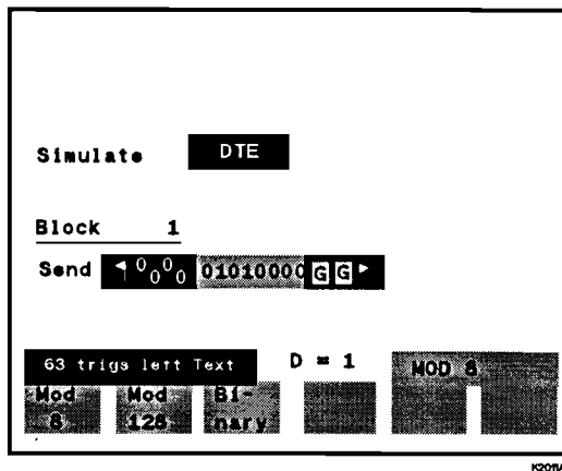
Figure 2-12. Selecting GFI in Level 3 Send String
