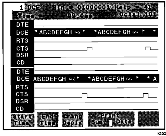
Figure 3-2. Timing Interval in Data & State Format
